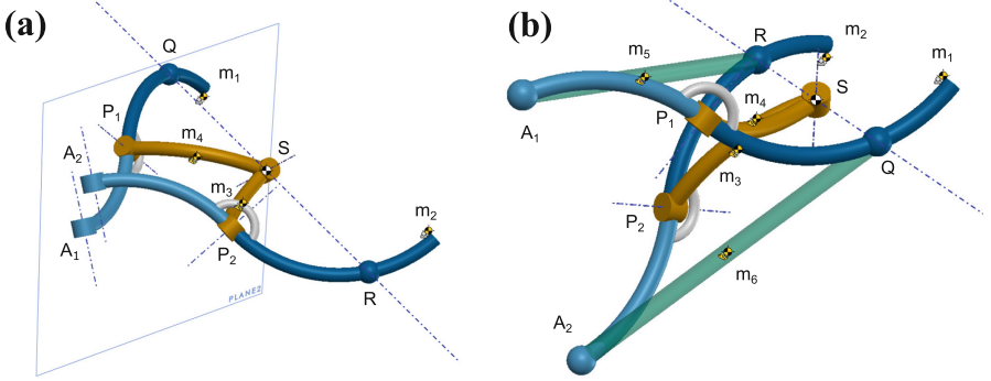
Fig. 2. a) Balanced spherical pantograph design with the similarity plane through S normal to the line through Q , S and R ; b) Additional links with spherical joints are needed to constrain the pantograph properly and have the common CoM in base pivot S for all motions.
