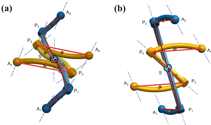
Fig. 8. Projections on two orthogonal planes of the two S-geometries.
