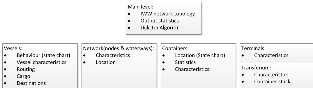
Figure 4-1: Anylogic levels overview
