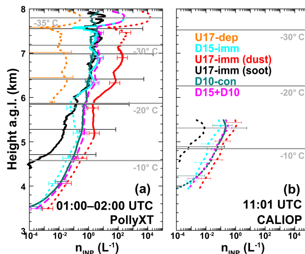
Figure 11. INP concentration profiles estimated from the measurements with (a) PollyXT between 01:00 and 02:00 UTC on 21 April 2016 and (b) CALIOP at 11:01 UTC on 21 April 2016. Temperature levels are derived from the WRF and MERRA-2 models. Colors refer to different INP parameterizations. Solid lines mark the temperature range for which the corresponding parameterization has been developed. Dashed lines refer to the extrapolated temperature range (see Table 1).
