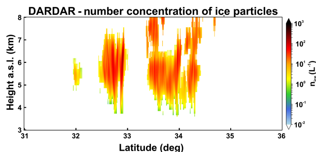
Figure 12. Spatial distribution of the DARDAR ice particle number concentrations at 11:01 UTC on 21 April 2016.
