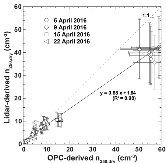
Figure 8. Correlation plot of n_{250,\text{dry}} obtained from drone-based OPC measurements and inferred from lidar observations (values for a mixture of mineral dust and continental pollution, black in Fig. 7) during coordinated activities on 5, 9, 15 and 22 April 2016. The solid line marks the linear regression with the corresponding function and squared correlation coefficient given in the plot. The 1 : 1 line is given as a dashed line.
