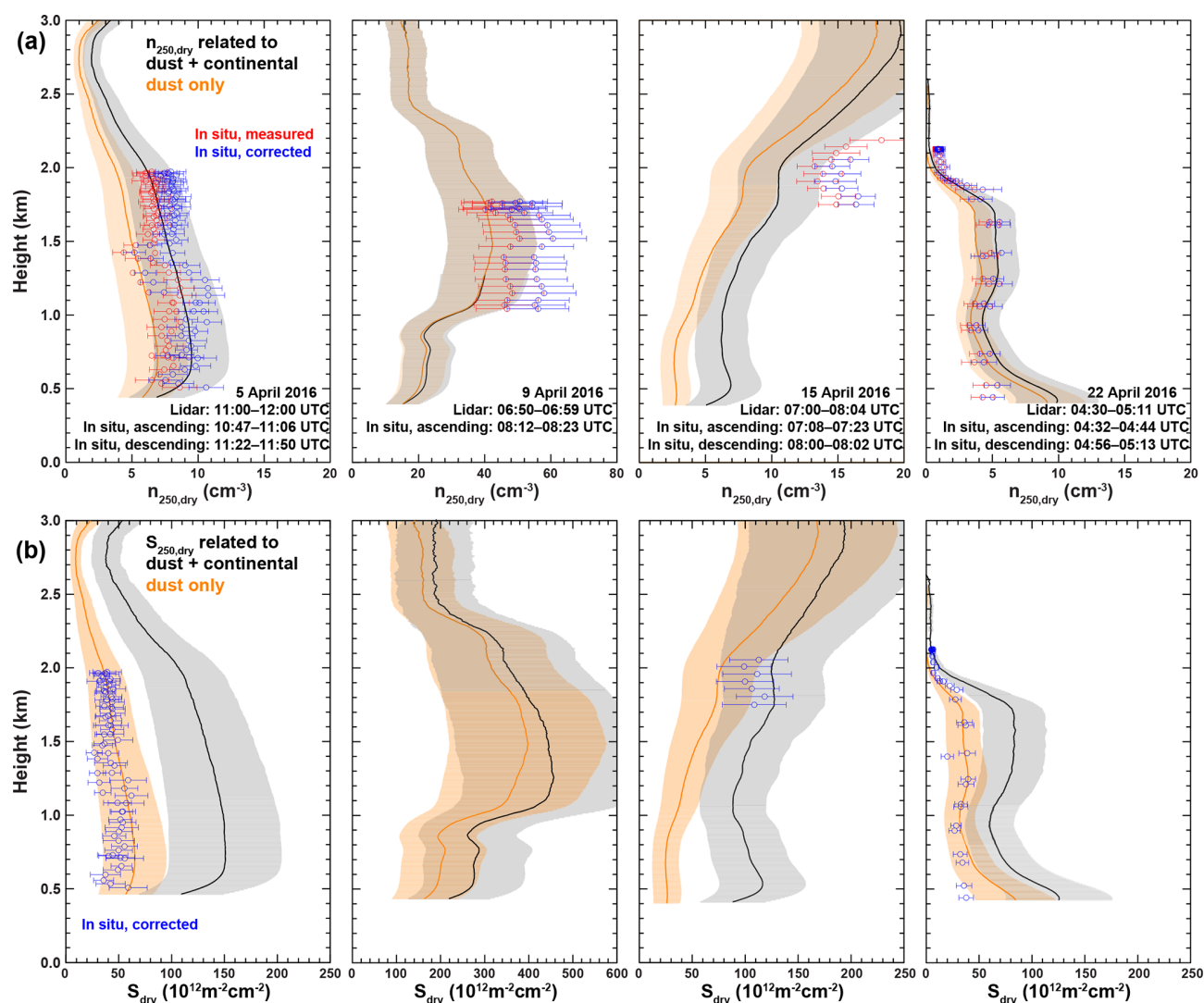
Figure 7. Profiles of n_{250,\text{dry}} (upper panel) and S_{\text{dry}} (lower panel) obtained from PollyXT and in situ measurements (UAV uncorrected data in red, UAV corrected data in blue) on 5, 9, 15 and 22 April 2016. The lidar-derived profiles refer to dust-only concentrations (orange), as well as the combination of dust and continental pollution concentrations (black).
