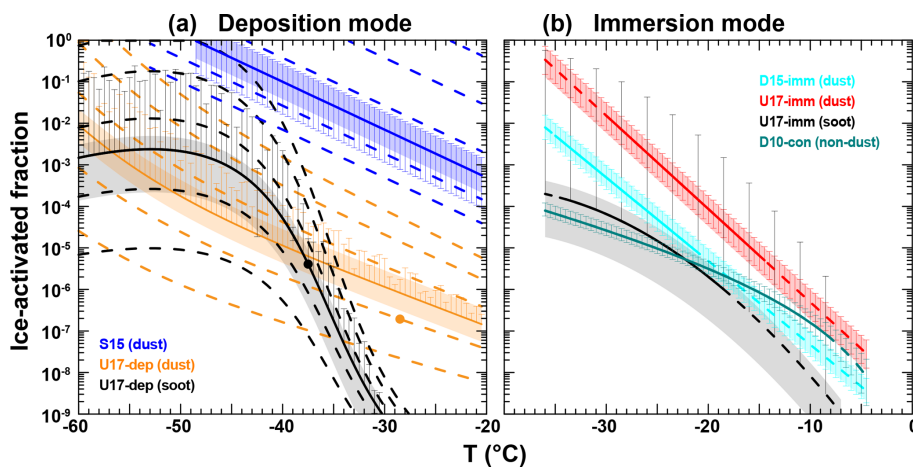
Figure 1. Fraction of ice-activated particles for the deposition nucleation (a) and immersion freezing (b) parameterizations used in this study. The particle concentrations used are derived assuming an extinction coefficient of 50 \text{ Mm}^{-1} for each of the different aerosol types (dust, continental, soot). The shaded areas take into account a range of the extinction coefficient from 10 \text{ Mm}^{-1} (lower limit) to 200 \text{ Mm}^{-1} (upper limit). The error bars mark the error of the respective parameterizations from error propagation using the uncertainties provided in Table 2. Negative error bars that exceed the scale are not shown. In the deposition mode (a), the bold lines correspond to ice supersaturation of 1.15 and the dashed lines to ice supersaturation of 1.05, 1.1, 1.2, 1.3 and 1.4. The black and orange dots indicate the maximum temperatures for which the parameterizations have been developed. In the immersion mode (b), the parameterizations are extrapolated over the immersion freezing temperature range (dashed lines).
