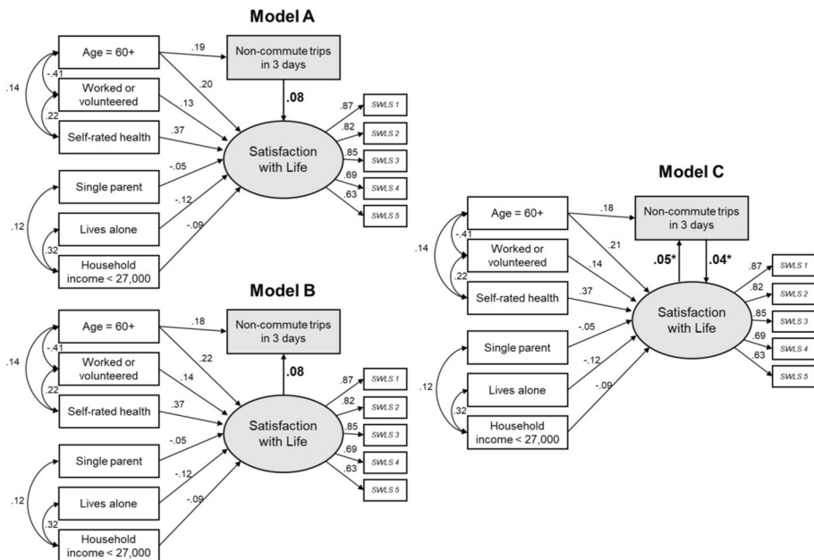
Fig. 2 Alternate structural equation model specifications. Note All coefficients are statistically significant, p < .05 , except those indicated by an asterisk
