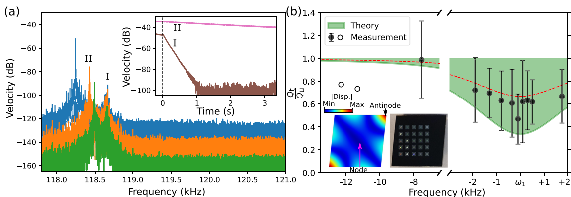
FIG. 4. (a) Mechanical velocity spectrum [20 log 10 ( v/v_{\text{ref}} ) with v_{\text{ref}} = 1 \text{ ms}^{-1} ] of three different devices, showing fundamental mode (II) close to the substrate mode (I) by driving with white noise. Inset: ringdowns of the untaped device fundamental mode (II) and substrate mode (I), showing the difference in their Q's. (b) Ratio of Q_t^2 measured on a taped ( Q_t ) vs untaped ( Q_u ) substrate: the increase in substrate losses causes a decrease in Q_t^2 when the modes are close in frequency. Theory curve shows expected reduction in Q_t^2 around \omega_1 for Q_1^t = 1.2 \times 10^4 \rightarrow 3 \times 10^3 when applying tape. Insets show the simulated mode shape of the substrate mode and a photo of the fabricated chip with 25 devices.
