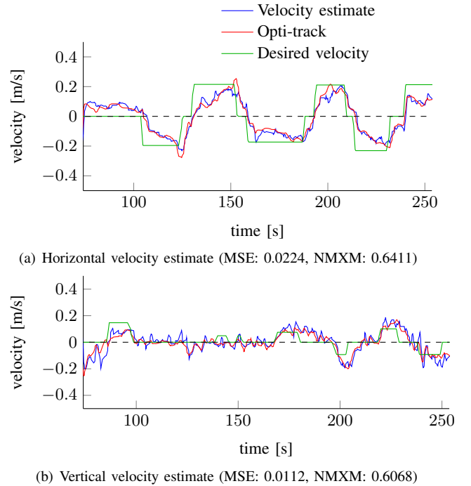
Fig. 8: The velocity estimate of the AR.Drone 2.0 and stereo-board assembly during a velocity control task with ground-truth as measured by OptiTrack. MSE and NMXM values are calculated for the entire flight.
