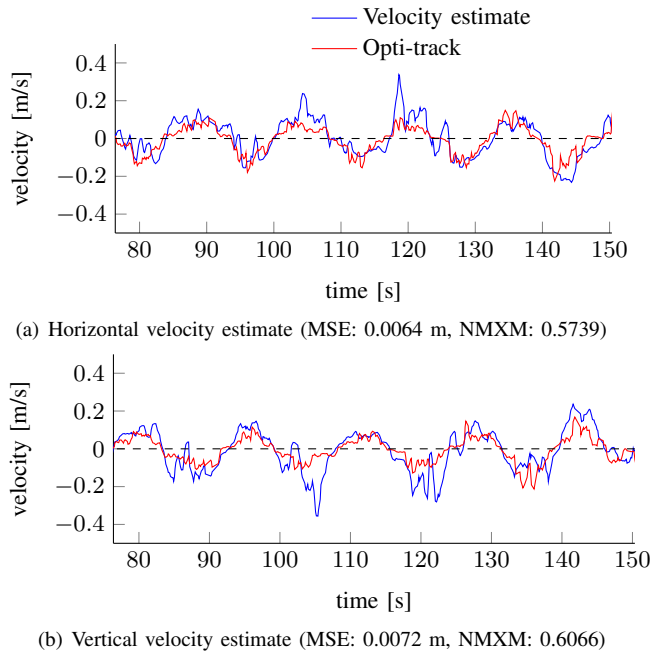
Fig. 9: Velocity estimates calculated by the pocket drone and stereo-board assembly, during an OptiTrack guided flight. MSE and NMXM values are calculated for the entire flight.
