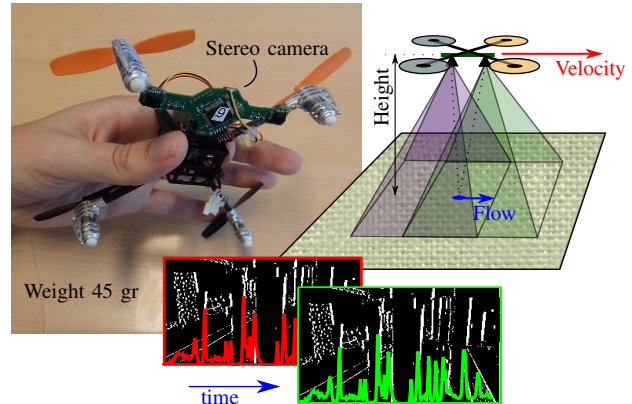
Fig. 1: Pocket drone with velocity estimation using a downward looking stereo vision system. A novel efficient optical flow algorithm runs on-board an STM32F4 processor running at only 168 MHz and with only 192 kB of memory. The so-determining optical flow and height, with the stereo-camera, provide the velocity estimates necessary for the pocket drone's low level control are obtained.
