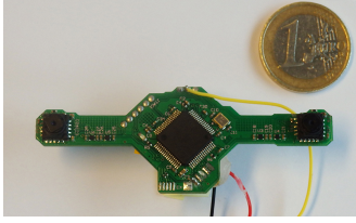
Fig. 6: 4 gram stereo-camera with a STM32F4 microprocessor with only 168 MHz speed and 192 kB of memory. The two cameras are located 6 cm apart from each other.
