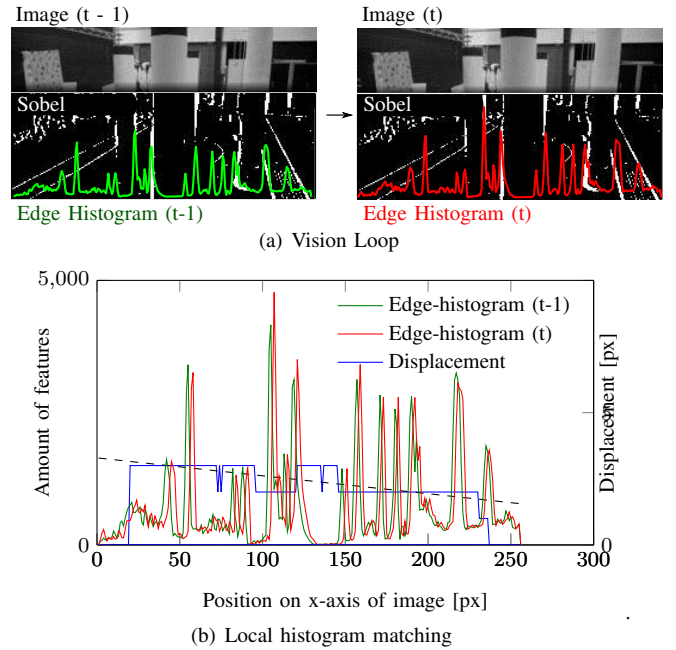
Fig. 2: (a) The vision loop with for creating the edge feature histograms and (b) the matching of the two histograms (previous frame (green) and current frame (red)) with SAD. This results in a pixel displacement (blue) which can be fitted to a linear model (dashed black line) for a global estimation.
