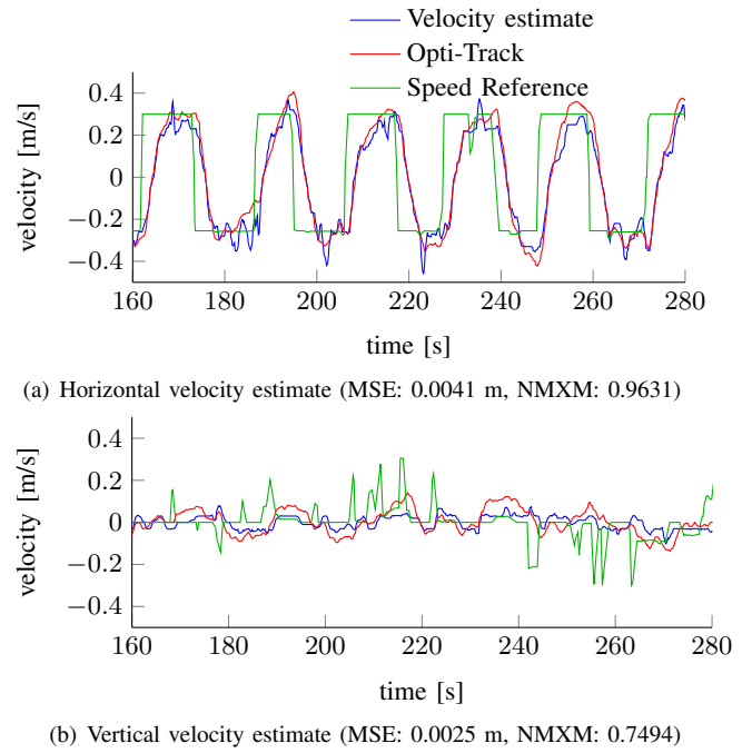
Fig. 10: Velocity estimates calculated by the pocket drone and stereo-board assembly, now using estimated velocity in the control. MSE and NMXM values are calculated for the entire flight which lasted for 370 seconds, where several external speed references were given for guidance.
