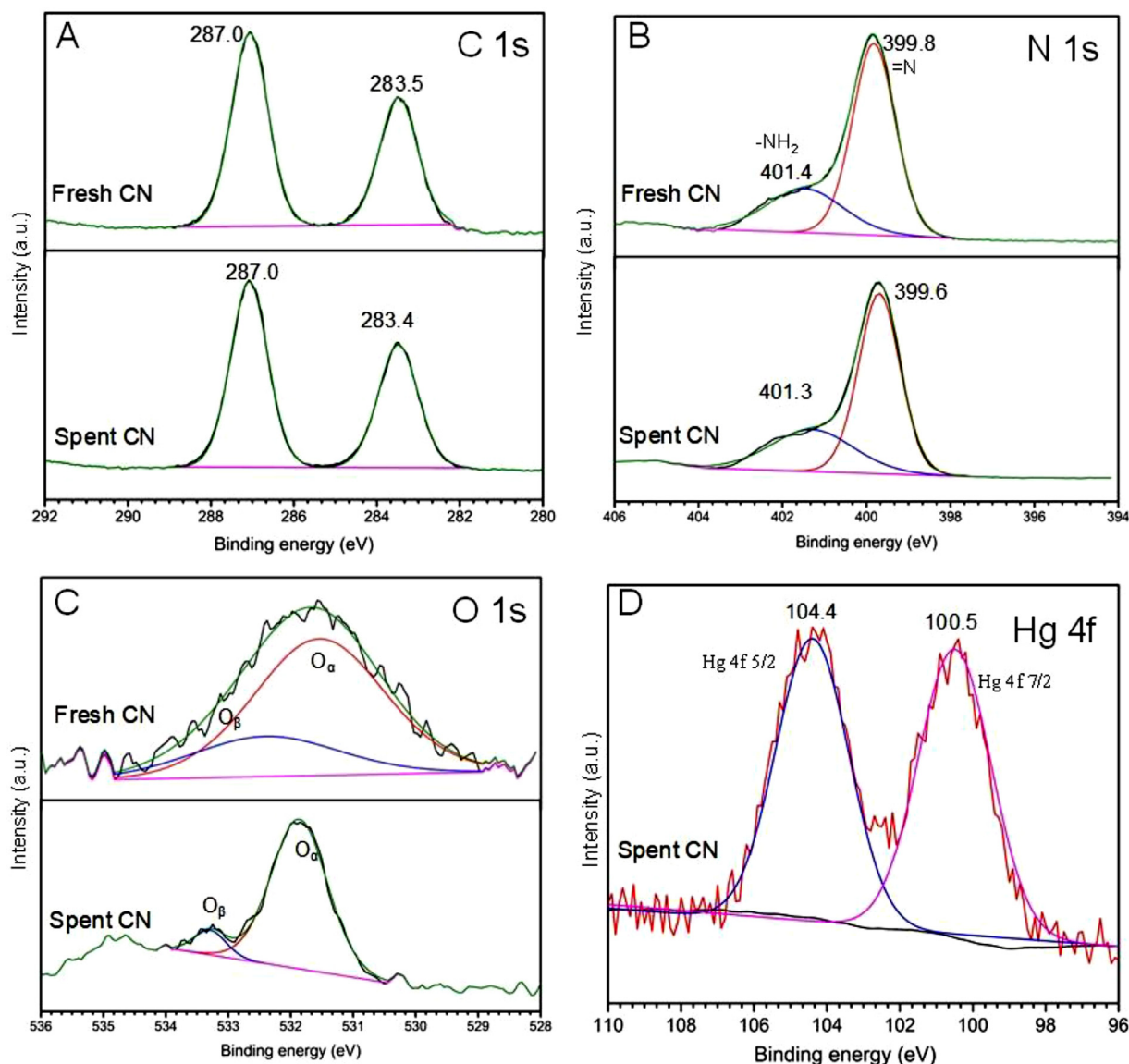
Fig. 4. XPS spectra of g-C 3 N 4 before and after the adsorption. (A) C 1 s, (B) N 1 s, (C) O 1 s, and (D) Hg 4f.
