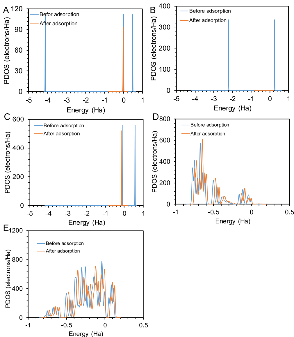
Fig. 5. PDOS of atoms (Hg, C 3 N 4 ) for surface system before and after Hg 0 adsorption on g-C 3 N 4 surface. (A) Hg s orbital; (B) Hg p orbital; (C) Hg d orbital; (D) s orbital of C and N; (E) p orbital of C and N. The Fermi level is set to be zero.
