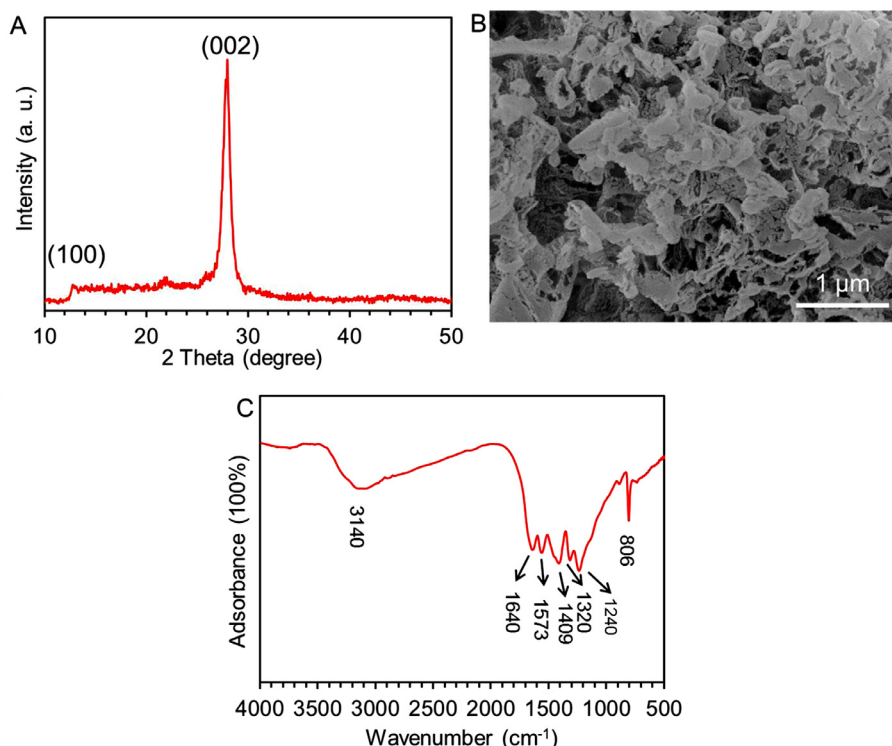
Fig. 1. The XRD pattern (A), SEM (B) and FT-IR (C) curve of as-prepared g-C 3 N 4 sample.
