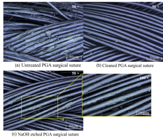
Fig. 12 Morphologies of the untreated and treated PGA multifilament surgical sutures. (a) untreated PGA surgical suture; (b) cleaned PGA surgical suture; (c) NaOH-etched PGA surgical suture.
