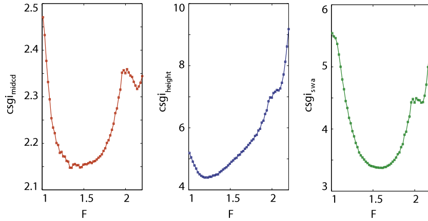
Figure 4. Gain in sensitivity of ICFS compared to CFS when csqi as a function of overlap parameter F is plotted for midcd (left), height (center) and swa (right) in the range 1.01 \leq F \leq 2.2 . Improvement in sensitivity is seen for all cases.
