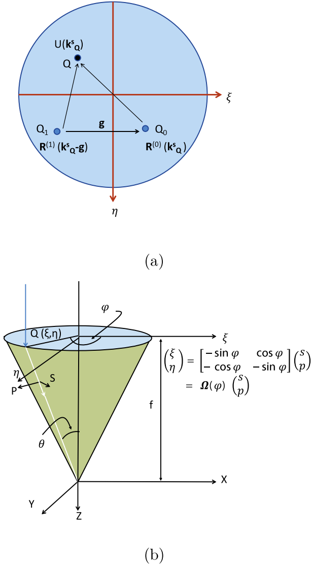
Figure 2. (a) The objective pupil plane where a point Q , which corresponds to the scattered transverse wavevector \mathbf{k}_Q^s , is contributed by the waves from direction \mathbf{k}_{Q_0}^s (corresponding to point Q_0 ) and \mathbf{k}_{Q_1}^s - \mathbf{g} (corresponding to point Q_1 ), respectively, through the superposition of their zeroth and first orders. Here, \mathbf{g} is the grating vector and \hat{\xi}, \hat{\eta} is the orthonormal basis at the pupil plane parallel to the (\hat{x}, \hat{y}) -basis, with -NA \leq \xi, \eta \leq NA . (b) An illustration of how the focusing action of the objective is modeled. The objective transforms a ray incident at Q(\xi, \eta) on its pupil plane to a plane wave of incidence angle (\theta, \varphi) . They are related by \varphi = \tan^{-1}(\eta/\xi) and \theta = \sin^{-1}\sqrt{\xi^2 + \eta^2} . The polarization of the incident ray is set to be in the pupil plane by a polarizer placed before the objective (not shown here) and, thus, expressible in \hat{\xi}, \hat{\eta} . It is also required to transform this polarization from basis \hat{\xi}, \hat{\eta} to S, P relative to the plane of incidence. This is carried out in two steps: first the rotation matrix \Omega(\varphi) is used to transform from \hat{\xi}, \hat{\eta} to an intermediate polar basis, and then this is transformed into the S, P basis with a unit matrix. Given the S, P components and the angles \theta, \varphi , one has sufficient information to define the incident wave on the grating.
