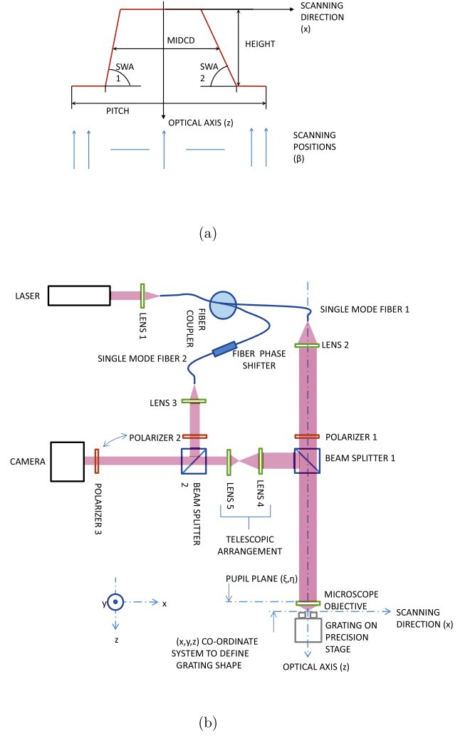
Figure 3. The grating parameters and the scanning are defined in (a). In the modeling, the center of the pitch is assumed to be on the z -axis without scan (initial position). The scanning positions are designated by \beta , with \beta = (0, 1, \dots, \beta_{\min} - 1) . If the grating vector has only an x -component, scanning is needed only along x and the \beta th scanning position denotes a shift of \beta\Delta x from the origin ( \Delta x is the scanning step size). (b) A possible scheme of the interferometric coherent scatterometry setup. The coordinate plane x-y is located in the back focal plane of the objective. The fiber coupler creates the reference and incident waves from an intensity stabilized laser. The scattered wave from the sample and the reference are superposed on beam splitter 2. Polarizers 2 and 3 are always parallel, as indicated by the arrow. The scanning is performed by a precision stage on which the sample is placed, whereas the reference phase shifts are introduced by a fiber phase shifter. Polarizer 1 sets the polarization of the incident wave.
