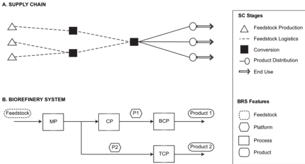
Fig. 2.1. Schematic example of a biorefinery project (supply chain and biorefinery system): As part of the supply chain (SC), feedstock from several locations is transported to distributed and centralized conversion centres, from which products are distributed to reach the final consumer and be used (A). In the biorefinery system (BRS), it is illustrated that feedstock pre-processing is mechanical (MP), and that chemical (CP), biochemical (BCP) and thermochemical (TCP) conversions are used to process two platforms (P1: Platform 1, P2: Platform 2) into two products (B).
