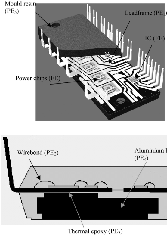
Fig. 4. Moulded lead frame power module.
