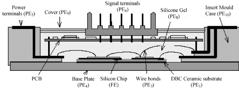
Fig. 2. Conventional intelligent power module (IPM) [15].
