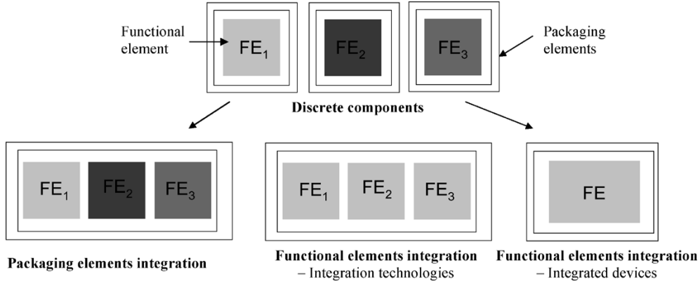
Fig. 1. Functional versus PEs integration.
