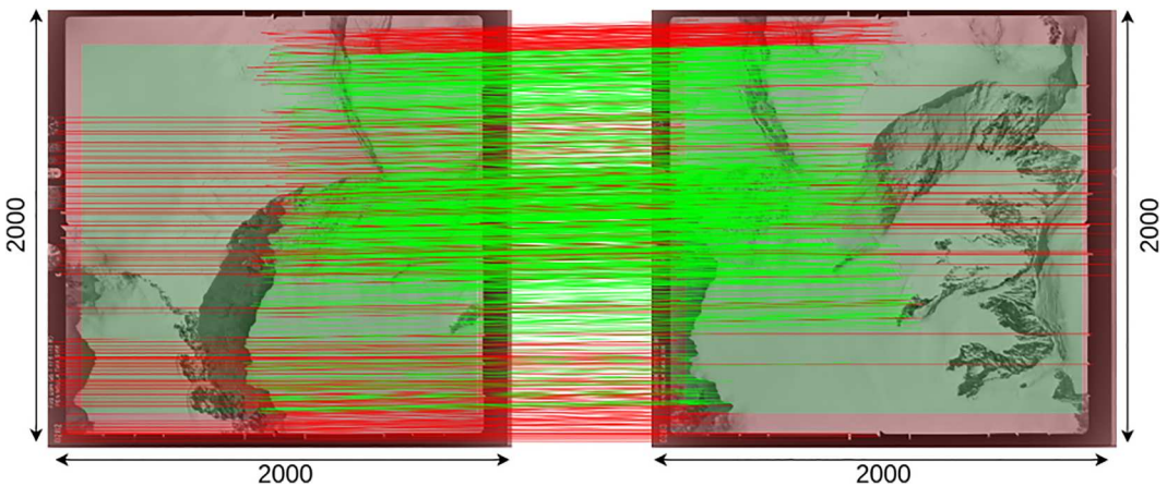
Figure 5. Initial matching between two images (IDs CA216632V0282 and CA216632V0283), that are resized to 2000 \times 2000 pixels. 881 valid matches (green lines) and 407 masked matches (red lines) are found.
