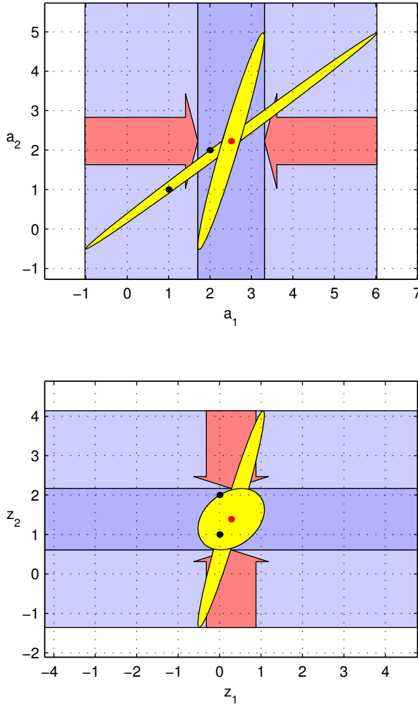
Figure A.1 Illustration of the stepwise decorrelation of the 2-dimensional search space by means of an integer Z-transformation. The original very elongated ellipsoidal search space (top) and the almost fully decorrelated nearly circular one (bottom) have the same size and are centered around the original ambiguities. (Figures courtesy of Peter Joosten).
