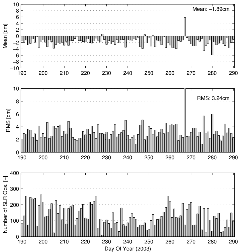
Figure 3.12 SLR comparison statistics for RDOD CHAMP ephemerides over the DOY 190 - 290, 2003 data arc. Shown are the mean offset (top) and the RMS (middle) of the SLR fit as well as the number of data points (bottom) used to obtain the statistics.
