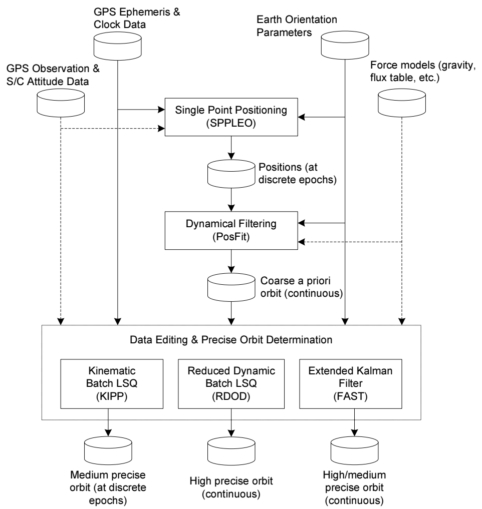
Figure 3.7 Processing scheme for GPS based precise orbit determination of LEO satellites using the GHOST toolkit.
