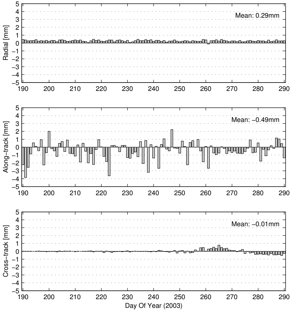
Figure 4.17 Daily mean offset in radial, along-track and cross-track direction between the float and fixed ambiguity reduced dynamic (EKF) relative position solutions.
