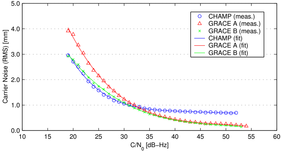
Figure 2.7 Upper limit of the carrier phase noise (measured and fitted) on the L_1 observation, as function of the carrier to noise density ratio ( C/N_0 ) for CHAMP, GRACE A and GRACE B.
