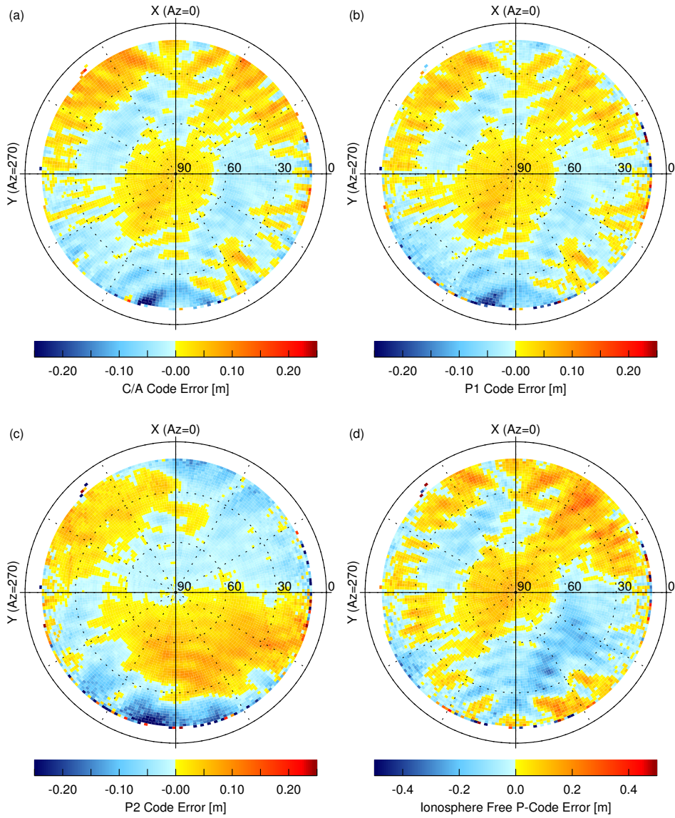
Figure 2.3 Systematic errors on the C/A (a), P_1 (b), P_2 (c) and ionosphere free (d) pseudorange observation data obtained from the the main POD antenna of the GRACE A BlackJack GPS receiver. The errors are expressed in the body fixed antenna diagram (see text).
