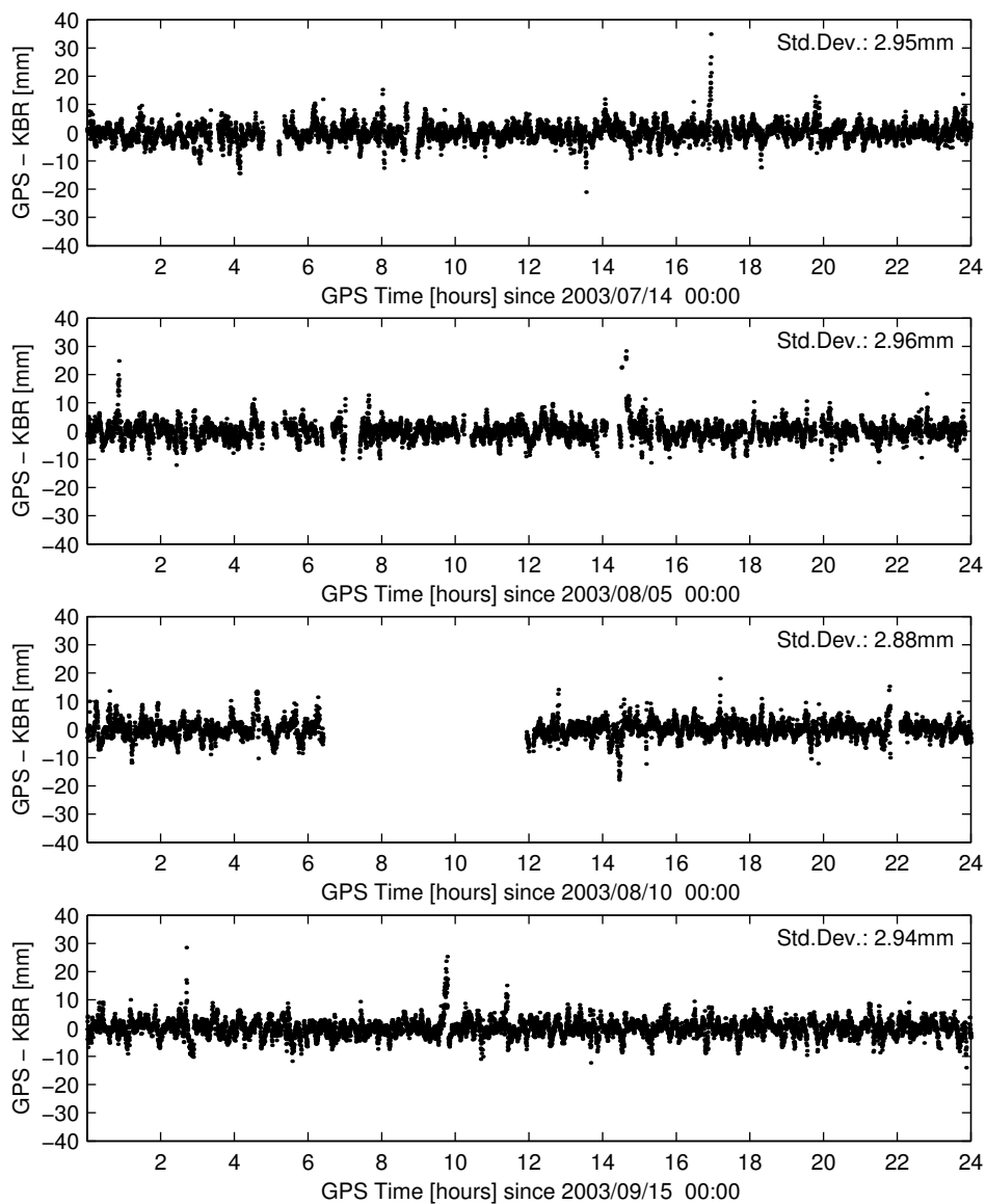
Figure 4.22 Time series of the KBR comparison residuals of the GRACE relative position solution. The relative position is obtained from the kinematic SPP process using the ionosphere free carrier phase observable constructed from L_A and L_2 , complemented with the integer ambiguities from the EKF. Only solutions with a PDOP value of 7 or lower are displayed and used. Shown are the results for (top down) DOY 195, DOY 217, DOY 222 and DOY 258.
