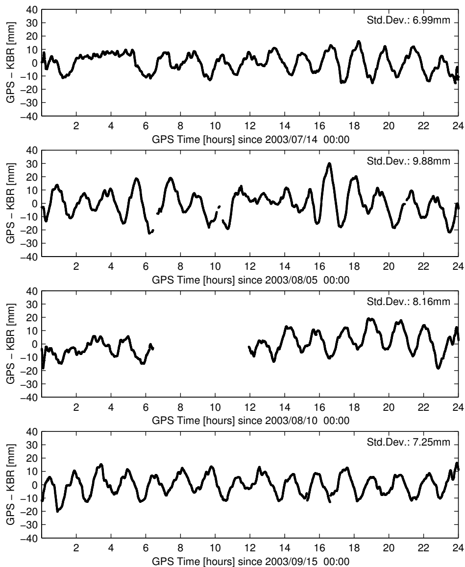
Figure 4.9 Time series of the KBR comparison residuals of the GRACE relative position solution. The relative position is obtained from the EKF with float ambiguities. Shown are (top down) DOY 195, DOY 217, DOY 222 and DOY 258.
