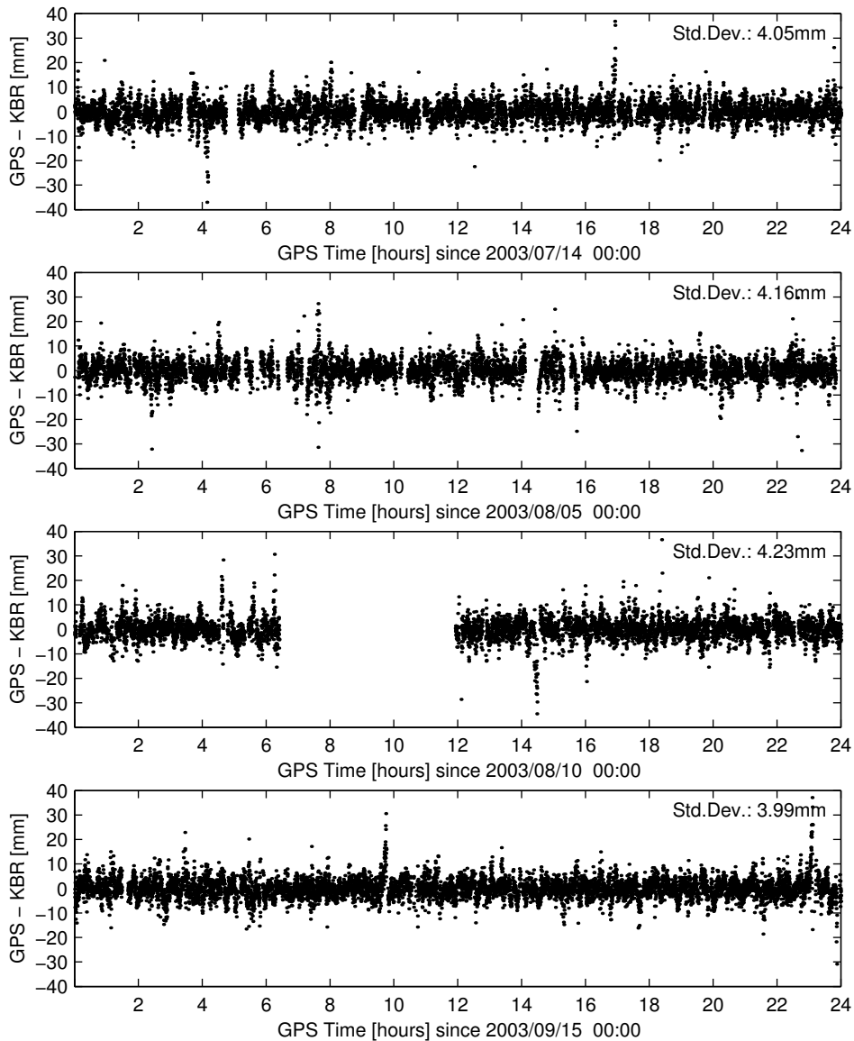
Figure 4.13 Time series of the KBR comparison residuals of the GRACE relative position solution. The relative position is obtained from the kinematic carrier phase data only SPP process, using the fixed ambiguities from the EKF. Only solutions with a PDOP value of 7 or lower are displayed and used. Shown are (top down) DOY 195, DOY 217, DOY 222 and DOY 258.
