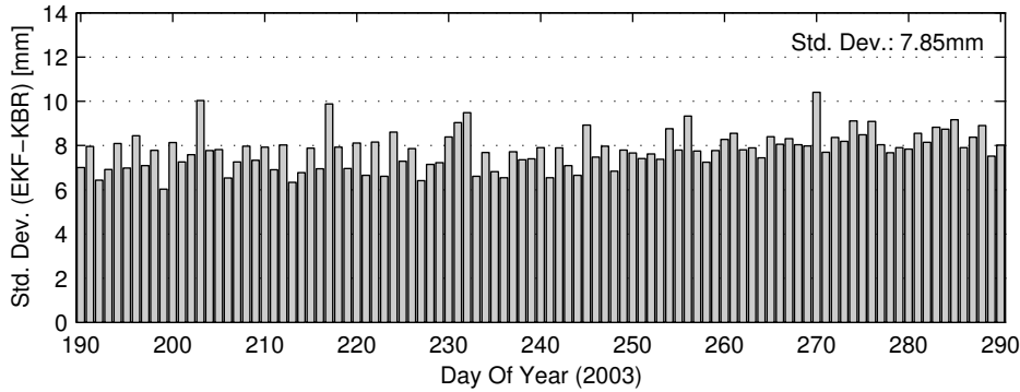
Figure 4.10 Daily standard deviations of the GRACE relative position, constructed by processing SD code and carrier phase observations with float ambiguities, when compared to the KBR measurements.
