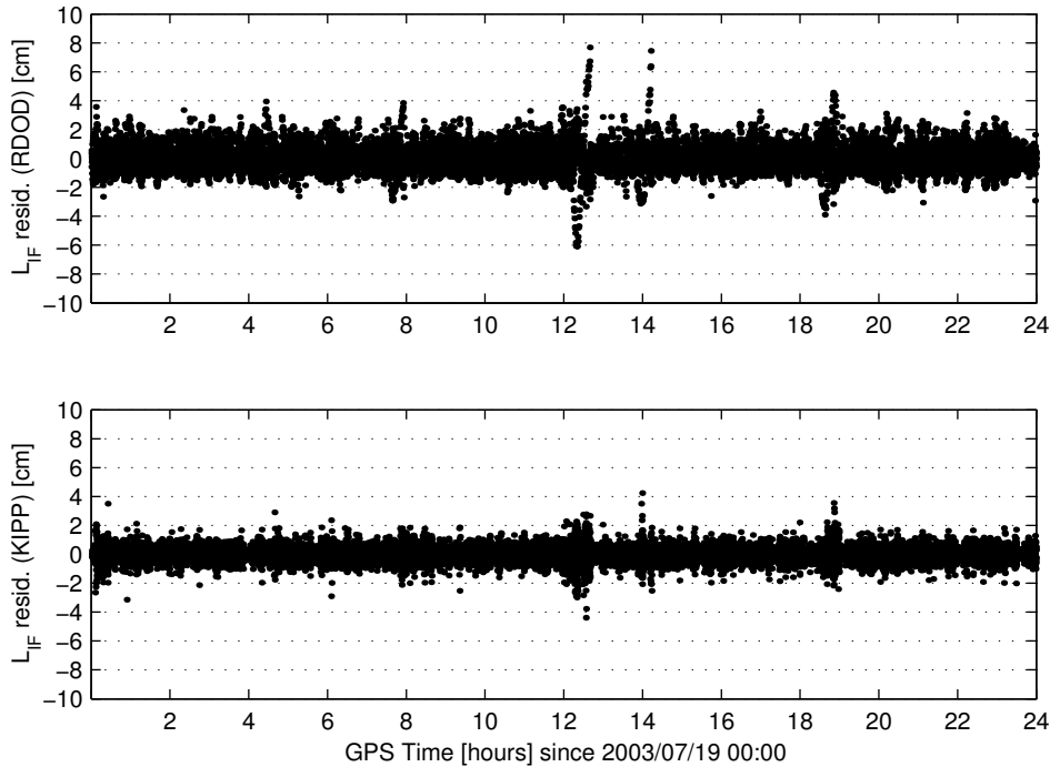
Figure 3.9 Post-fit residuals of the kinematic (KIPP, bottom) and reduced-dynamic (RDOD, top) batch LSQ orbit determination for GRACE A on July 19, 2003 (DOY 200).
