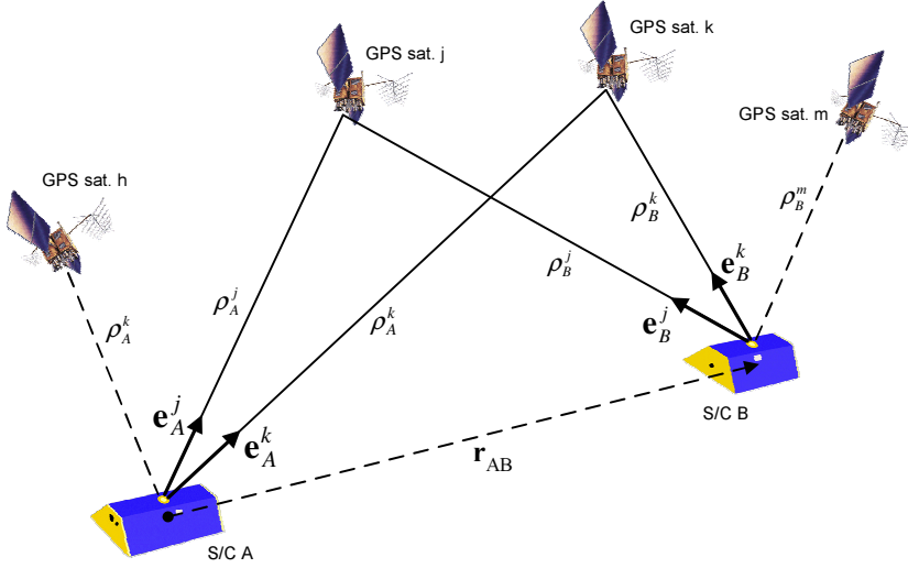
Figure 2.1 Overall viewing geometry for relative (spacecraft) positioning using differenced GPS observations. GPS satellites j and k are commonly observed by both receivers and thus SD and DD observations can be formed. This is not the case for GPS satellites h and m , which are only observed by one receiver.
