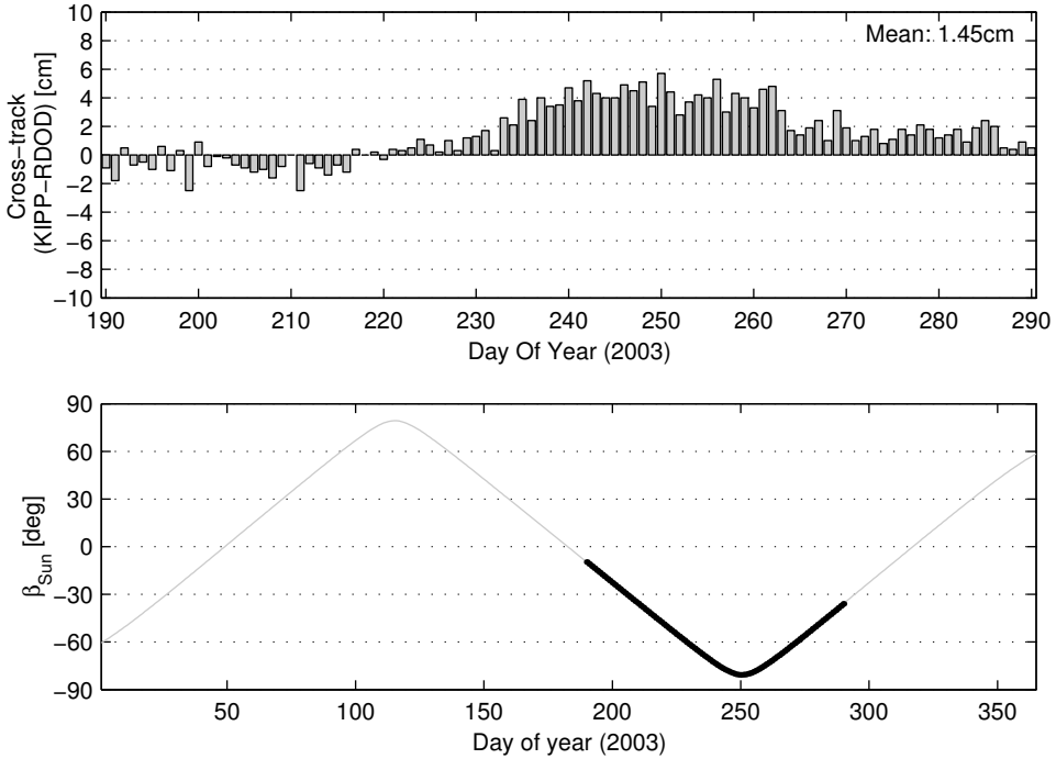
Figure 3.10 Cross-track mean offset for the CHAMP KIPP-RDOD comparison (top) over the entire data arc, together with the angle between the Sun vector and the CHAMP orbital plane (bottom) for 2003. The period corresponding to the data arc is highlighted.
