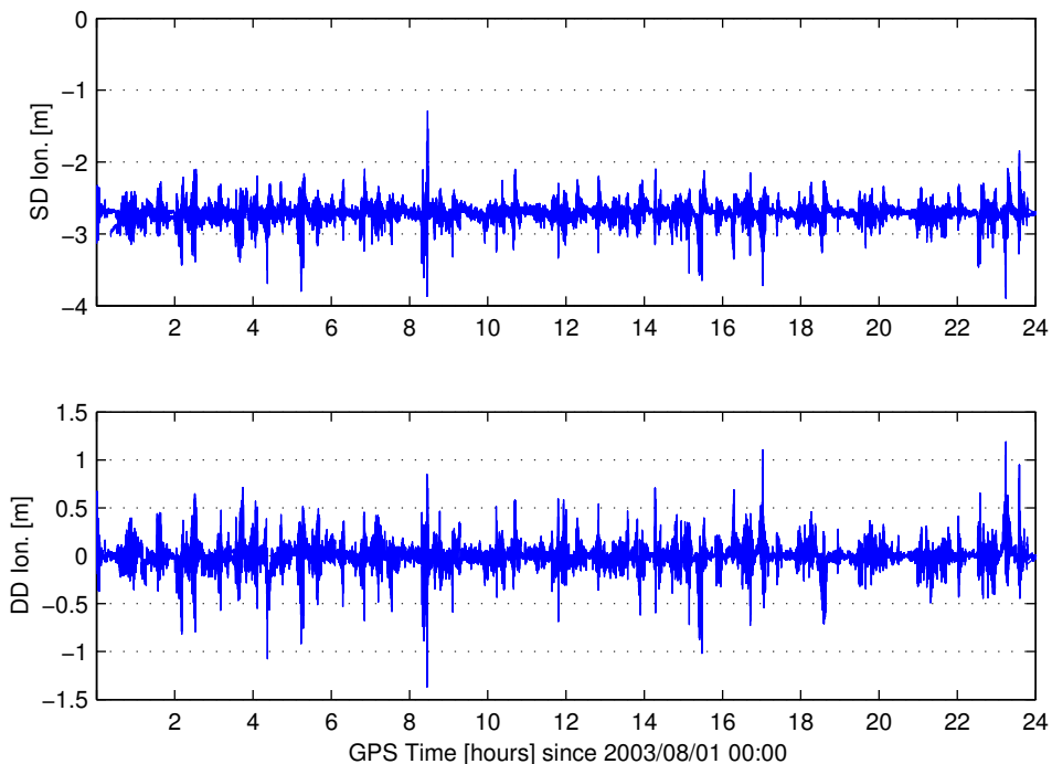
Figure 4.7 The SD (top) and DD (bottom) ionospheric path delays between the GRACE S/C for August 1, 2003 (DOY 213).
