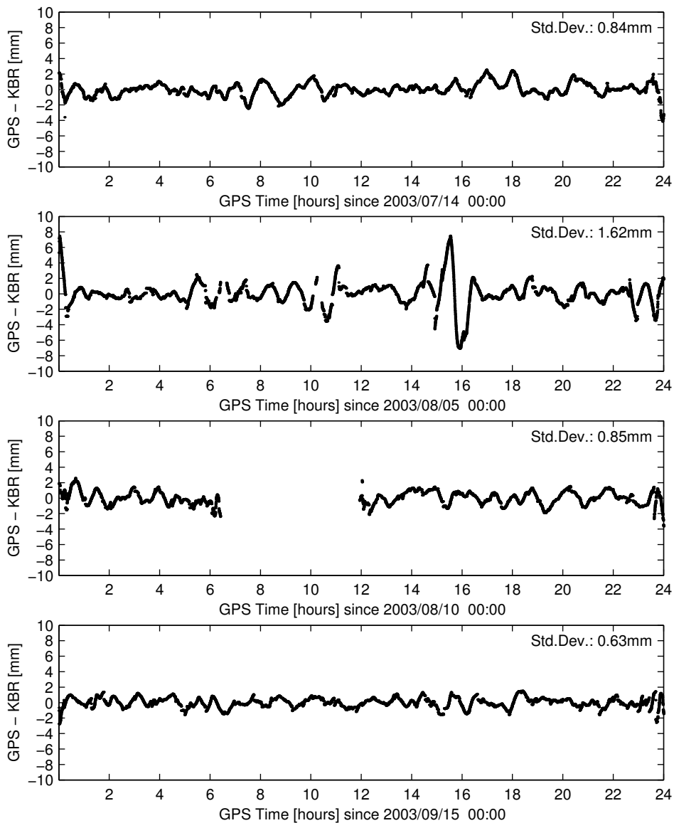
Figure 4.12 Time series of the KBR comparison residuals of the GRACE relative position solution. The relative position is obtained from the EKF when fixing DD ambiguities to integer values. Shown are (top down) DOY 195 (average situation), DOY 217 (worst case), DOY 222 (extended data gap) and DOY 258 (best overall fit).
