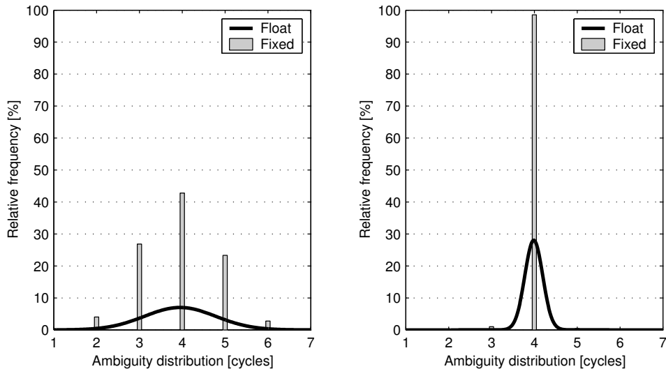
Figure 4.1 Distribution of a double difference ambiguity as real-valued (float) and accompanying integer (fixed) solution (Source: [Joosten and Tiberius, 2000]). In the left figure the probability mass for the correct value (4) is still low, in the right figure this might already be high enough to neglect the stochastic nature of the ambiguity.
