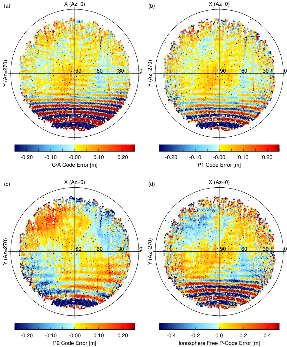
Figure 2.5 Systematic errors on the C/A (a), P_1 (b), P_2 (c) and ionosphere free (d) pseudorange observation data obtained from the the main POD antenna of the GRACE B BlackJack GPS receiver during the time the occultation antenna was active. The errors are expressed in the body fixed antenna diagram (see text).
