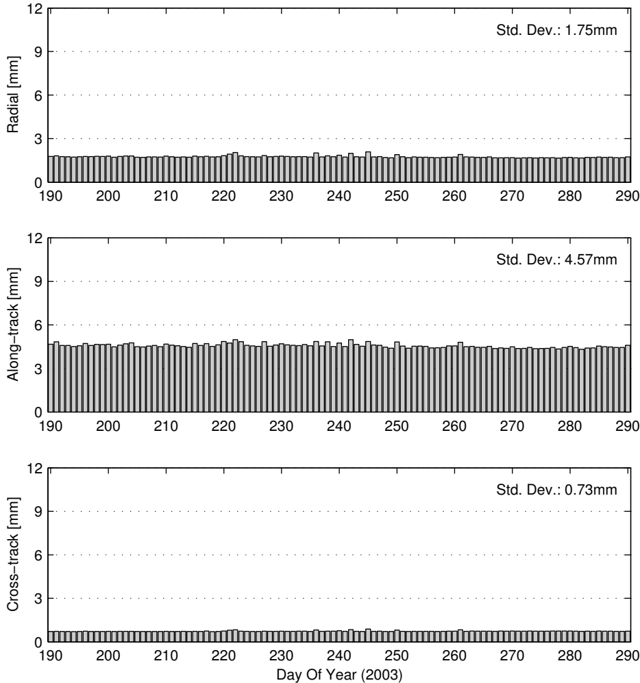
Figure 4.19 Daily formal variances of the extended Kalman filter in radial, along-track and cross-track direction, in the comparison between the float and fixed ambiguity relative position solutions.
