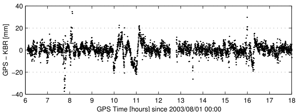
Figure 4.2 KBR Fit of the kinematic single point positions using integer ambiguities, obtained from the kinematic batch LSQ.
