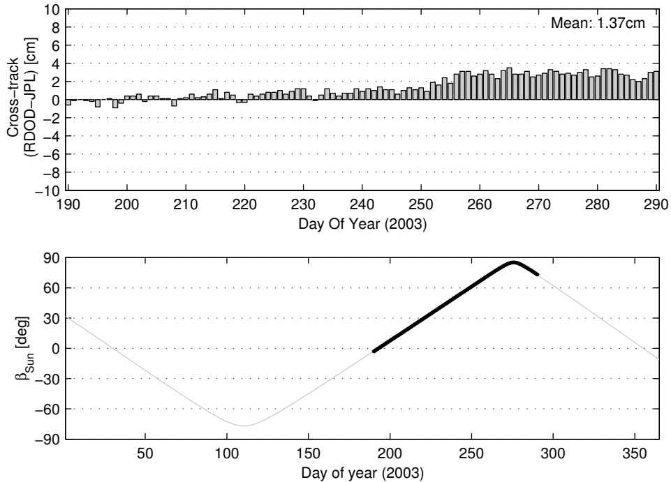
Figure 3.11 Cross-track mean offset for the GRACE B RDOD-JPL comparison (top) over the entire data arc, together with the angle between the Sun vector and the GRACE orbital plane (bottom) for 2003. The period corresponding to the data arc is highlighted.
