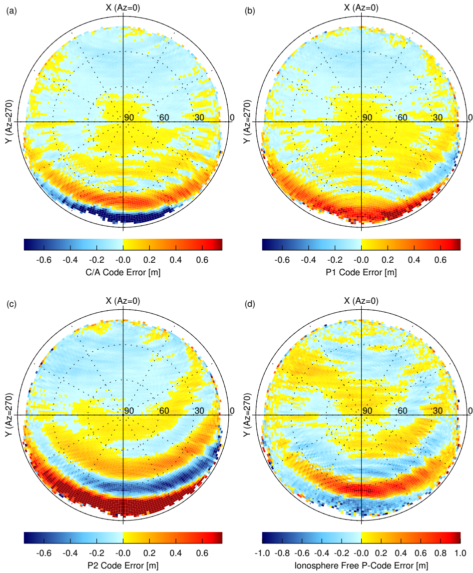
Figure 2.2 Systematic errors on the C/A (a), P_1 (b), P_2 (c) and ionosphere free (d) pseudorange observation data obtained from the main POD antenna of the CHAMP BlackJack GPS receiver. The errors are expressed in the body fixed antenna diagram (see text).
