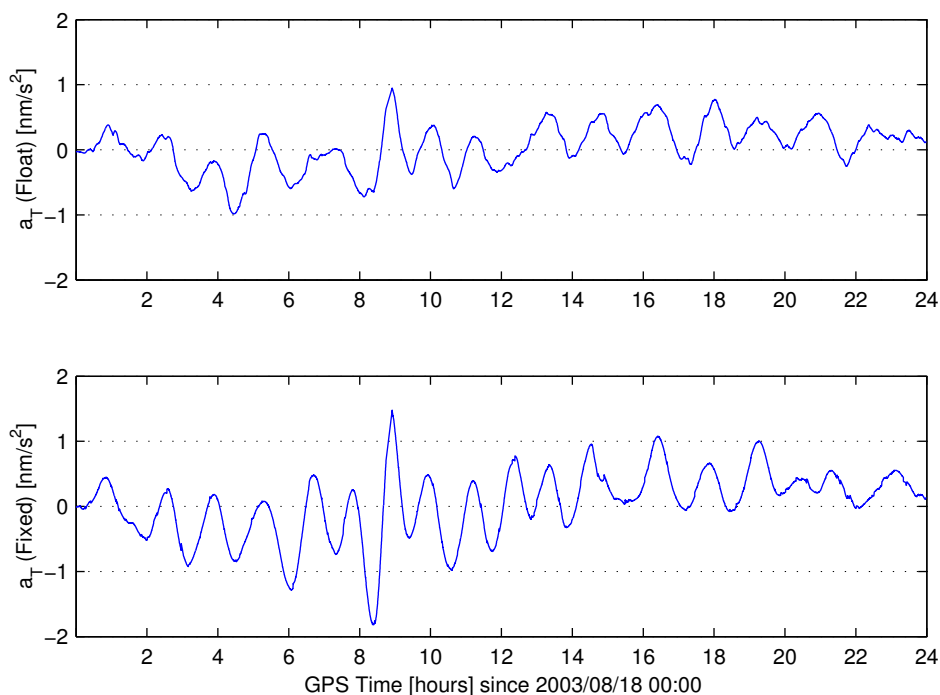
Figure 4.6 Relative empirical accelerations in the along-track direction ( a_T ) for the FRNS program for August 18, 2003 (DOY 230). Shown are the situations with float (top) and fixed (bottom) ambiguities
