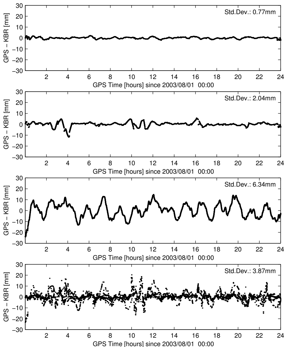
Figure 4.23 Time series of the KBR comparison residuals of the GRACE relative position solution. Shown are the results of different ambiguity resolution and fixing concepts for DOY 213. Top-down are given the solution with the overall integer validation scheme applied, the solution with an integer validation scheme not screening the individual ambiguity residuals, the float solution, and the solution with 'locally' fixed integers.
