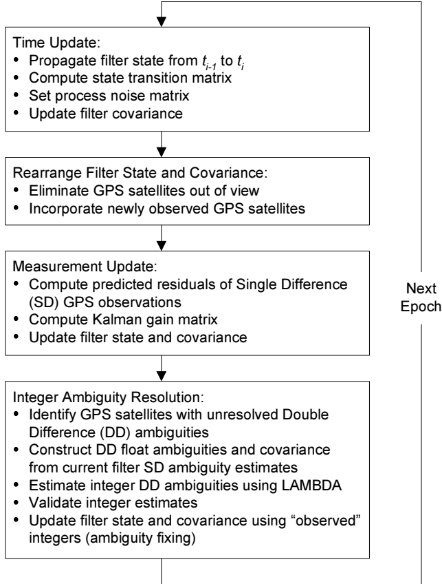
Figure 4.3 Epoch wise processing scheme of the Extended Kalman Filter for relative positioning of spacecraft.
