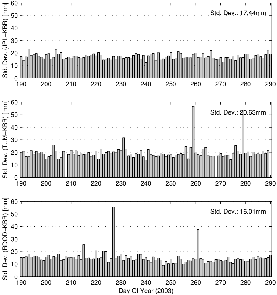
Figure 4.8 Daily standard deviations of the GRACE relative position, constructed from the individual satellite orbits, when compared to the KBR measurements.
