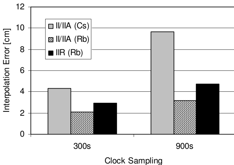
Figure 3.1 RMS error of GPS clock interpolation for 5 and 15 minute intervals. (Source: [Montenbruck et al., 2005b])
