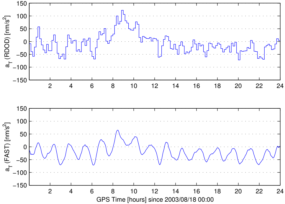
Figure 3.8 Empirical accelerations of GRACE B in the tangential, a_T , or along-track direction for both the reduced dynamic batch LSQ (top) and the EKF (bottom) for August 18, 2003 (DOY 230).
