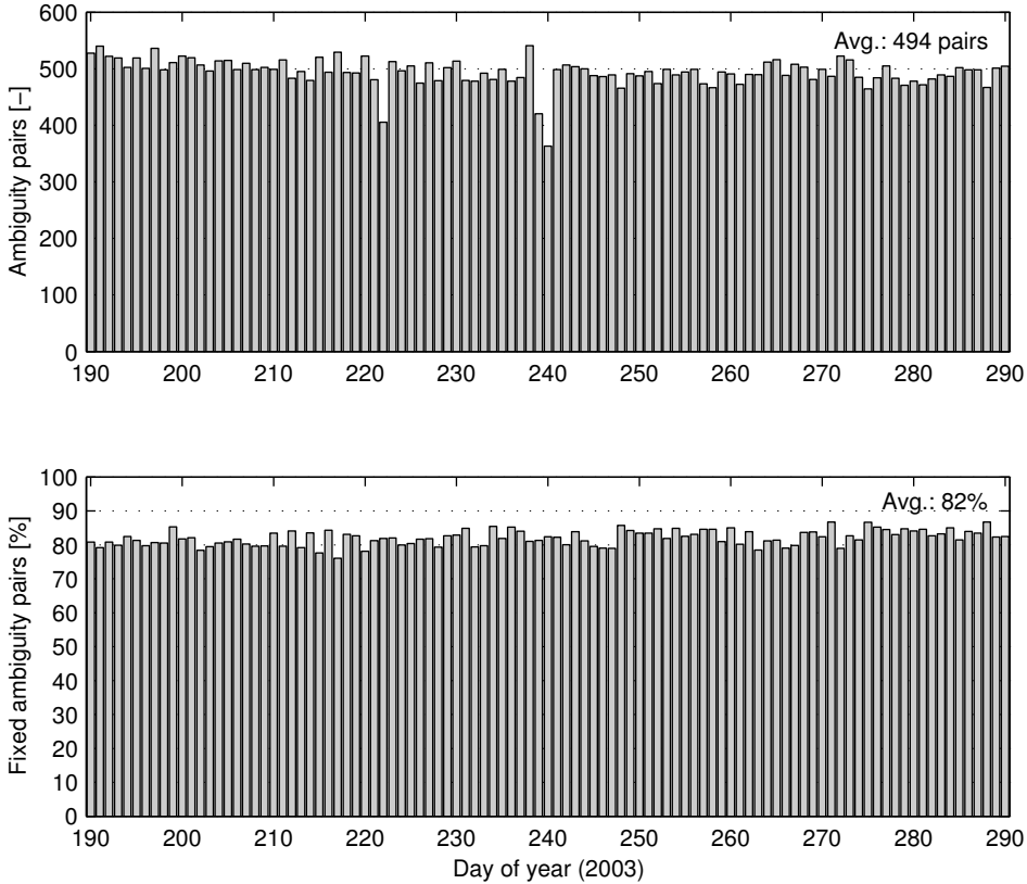
Figure 4.11 The total number of SD ambiguity pairs processed by the EKF on a daily basis (top), as well as the percentage of them that are eventually part of a fixed integer DD value (bottom).
