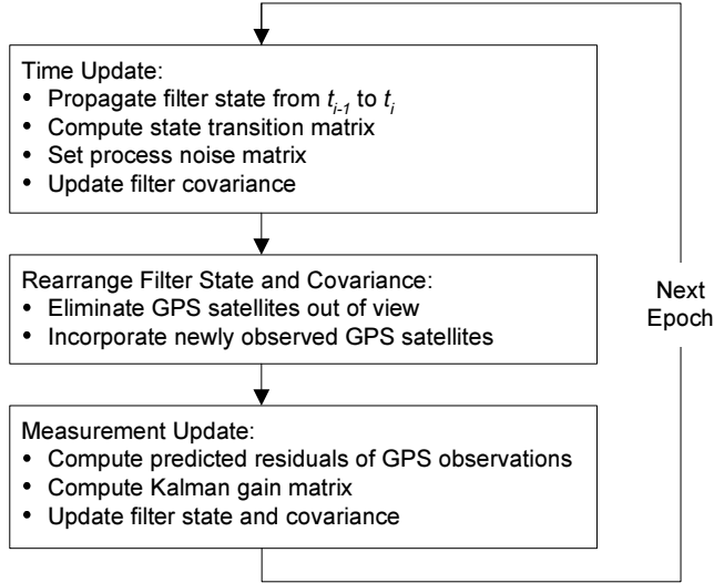
Figure 3.5 Extended Kalman Filter processing scheme for GPS based precise orbit determination
