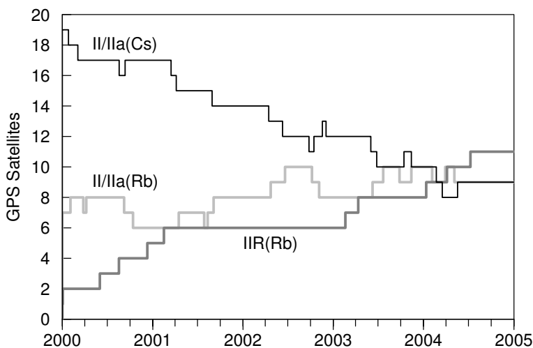
Figure 3.2 Number of GPS satellites operating cesium (Cs) and rubidium (Rb) clocks over time. (Source: [Montenbruck et al., 2005b])
