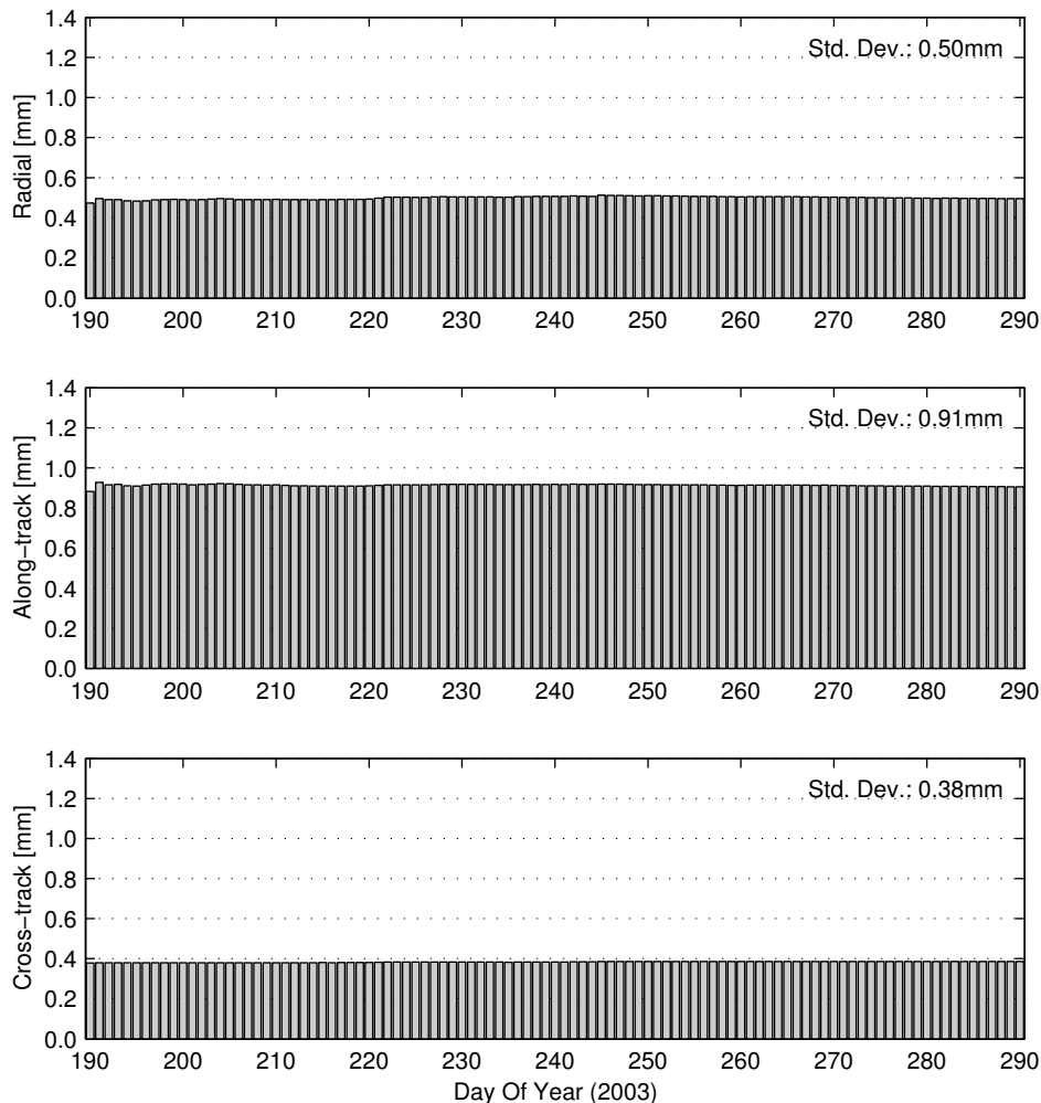
Figure 4.20 Daily formal variances of the extended Kalman filter in radial, along-track and cross-track direction, when constructing the fixed ambiguity relative position solution.
