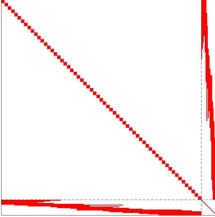
Figure 3.3 Structure of the normal equations for kinematic least-squares batch estimation of epoch-wise position and clock corrections, as well as carrier phase biases over continuous tracking arcs.
