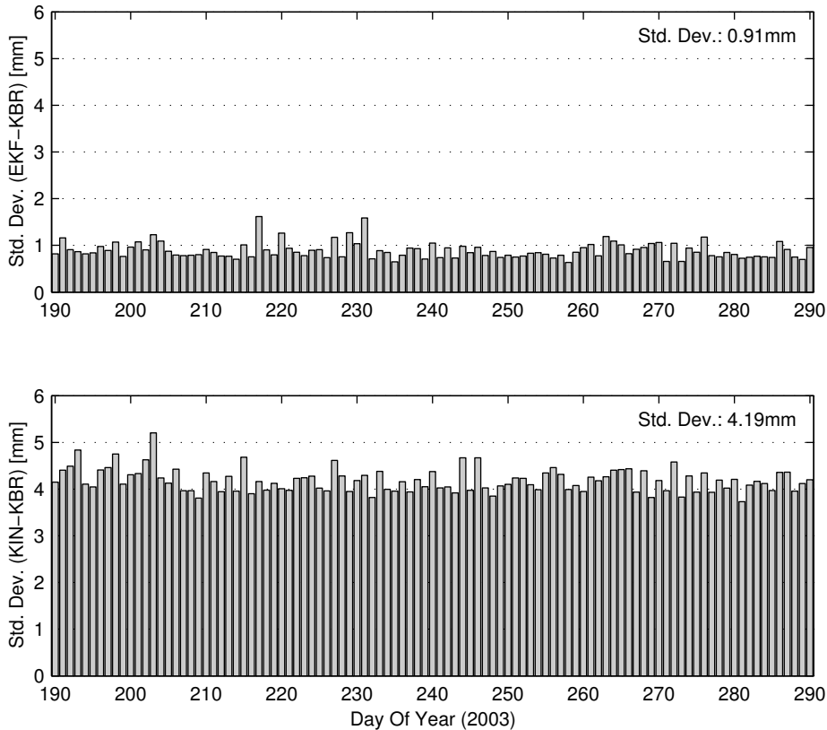
Figure 4.14 Daily standard deviations of the GRACE relative position, constructed by processing SD code and carrier phase observations with fixed ambiguities, when compared to the KBR measurements. The top figure shows the reduced dynamic solution from the EKF, the bottom one the kinematic SPP position solution constructed using carrier phase data in conjunction with the integer DD ambiguities from the EKF.
