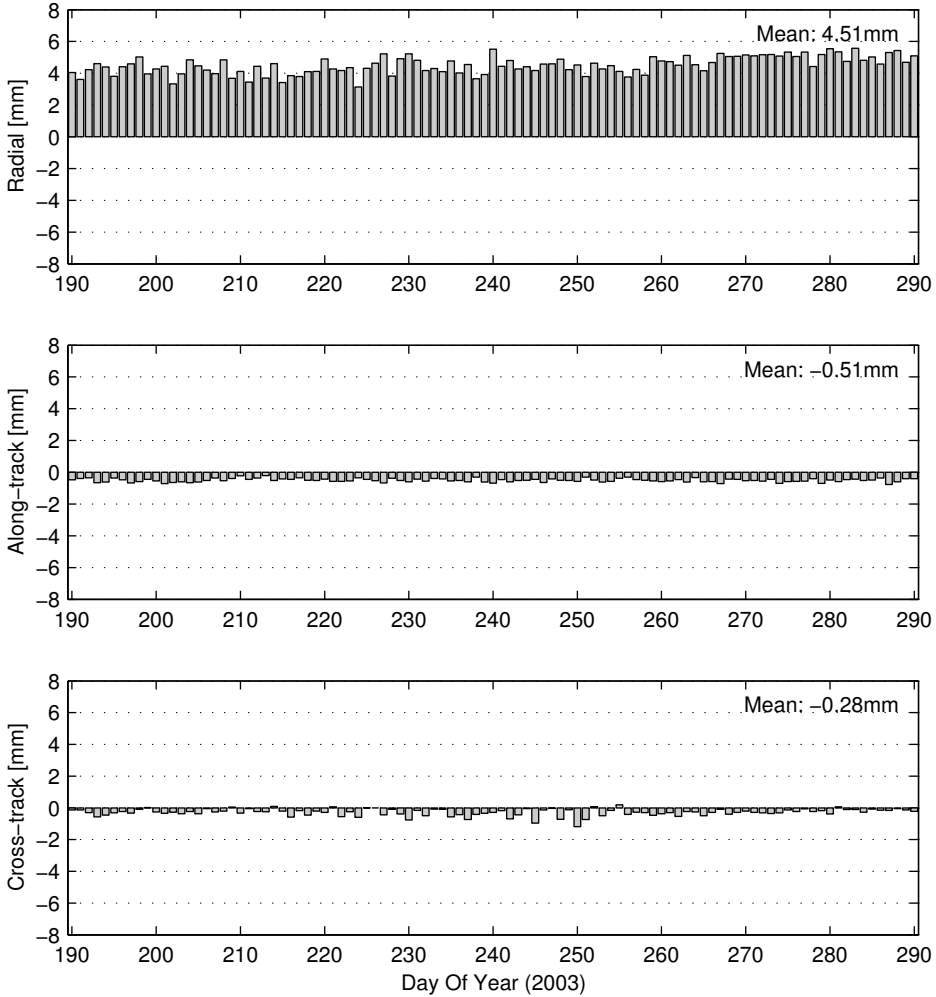
Figure 4.15 Daily mean offset in radial, along-track and cross-track direction between the kinematic and reduced dynamic relative position solution, both constructed using fixed integer ambiguities.
