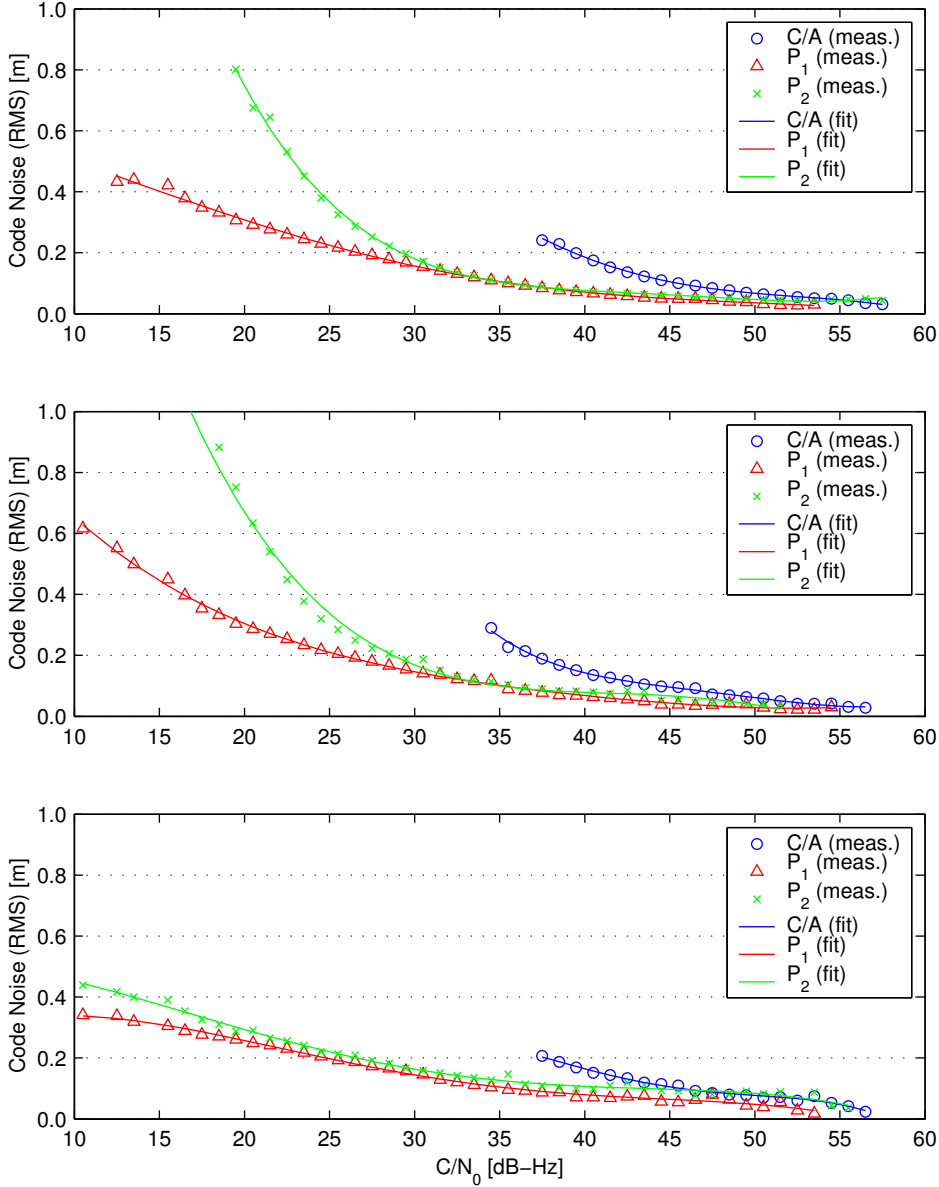
Figure 2.6 Pseudorange noise (measured and fitted), after the removal of the systematic effects, as function of the carrier to noise density ratio ( C/N_0 ) for CHAMP (top), GRACE A (middle) and GRACE B (bottom).
