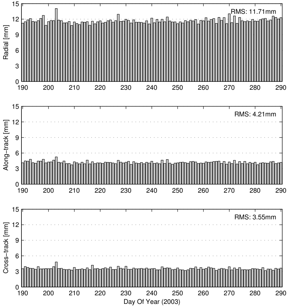
Figure 4.16 Daily RMS values in radial, along-track and cross-track direction of the comparison between the kinematic and reduced dynamic relative position solution, both constructed using fixed integer ambiguities.
