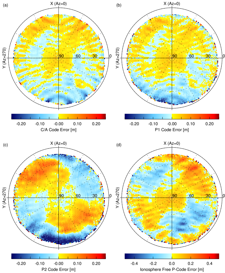
Figure 2.4 Systematic errors on the C/A (a), P_1 (b), P_2 (c) and ionosphere free (d) pseudorange observation data obtained from the the main POD antenna of the GRACE B BlackJack GPS receiver. The errors are expressed in the body fixed antenna diagram (see text).
