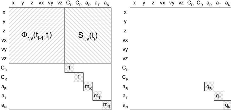
Figure 3.6 The structure of the transition ( \Phi_Y , left) and the process noise ( Q_Y , right) matrices, concerning the dynamic parameters in the EKF.
