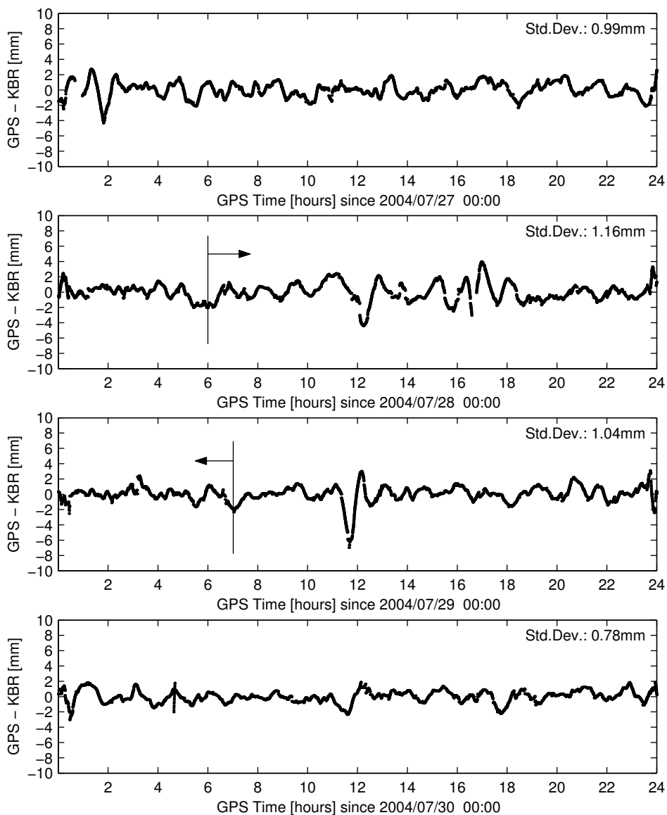
Figure 4.21 Time series of the KBR comparison residuals of the GRACE relative position solution. The relative position is obtained from the EKF when fixing ambiguities to integer values. Shown are (top down) DOY 209, DOY 210, DOY 211 and DOY 212 of 2004. The period over which the GPS occultation antenna was activated (DOY 210 and 211) has been marked.
