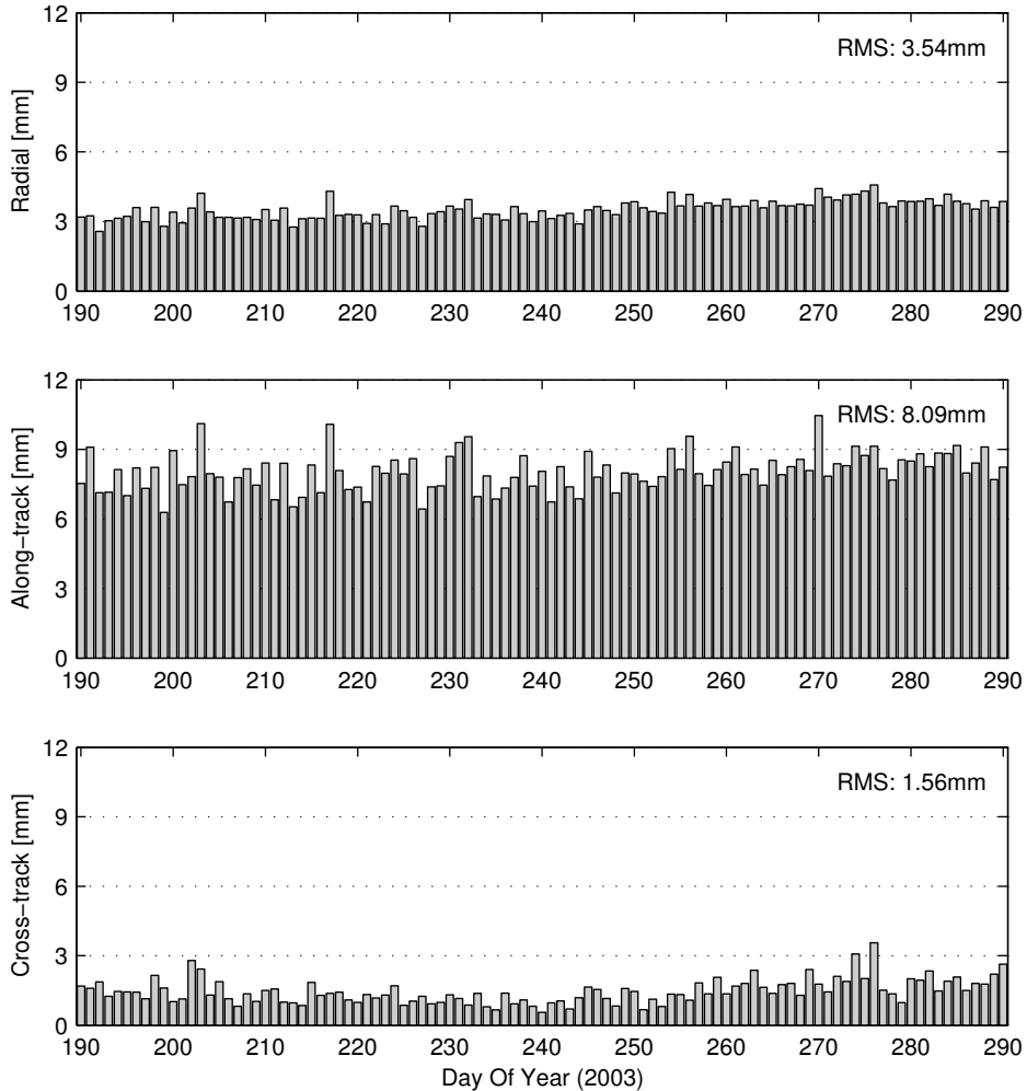
Figure 4.18 Daily RMS values in radial, along-track and cross-track direction of the comparison between the float and fixed ambiguity reduced dynamic (EKF) relative position solutions.
