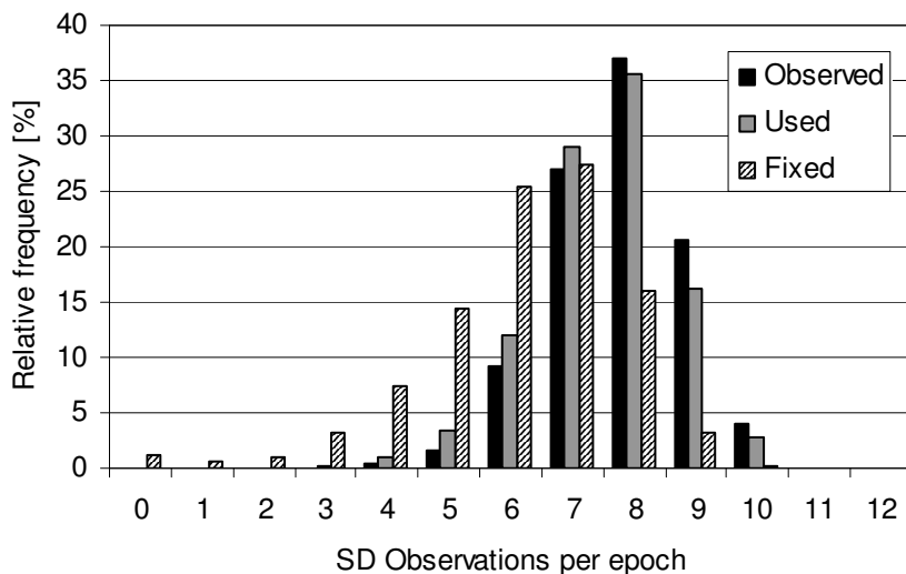
Figure 4.5 Average distribution, for the entire 101-day GRACE data arc, of the number of SD observations per epoch. Shown are the available SD observations ('Observed'), the ones used ('Used') by the filter and the ones of which the SD carrier phase ambiguity is part of an already resolved integer DD ambiguity ('Fixed').
