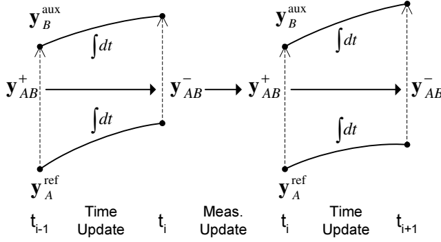
Figure 4.4 Illustration of the propagation of the relative spacecraft state over the time and measurement update. (Source: [Kroes et al., 2005])
