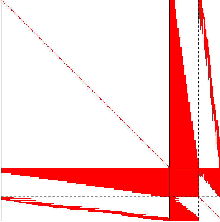
Figure 3.4 Structure of the normal equations for least-squares batch estimation of epoch-wise clock corrections, dynamic orbit parameters and carrier phase biases over continuous tracking arcs.
