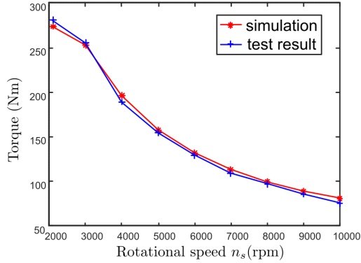
Fig. 4. Torque-speed curve comparison between the test results and the simulated results.
