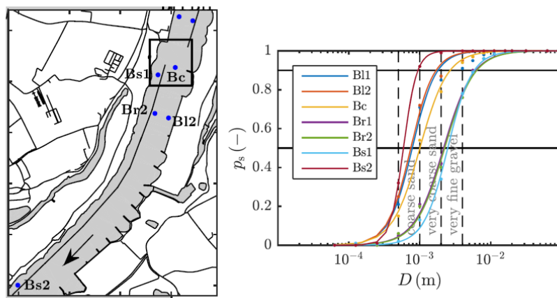
Figure 5 – Bed sample locations (left) and gradation of the samples (right) [De Ruijsscher et al. (2020)]
