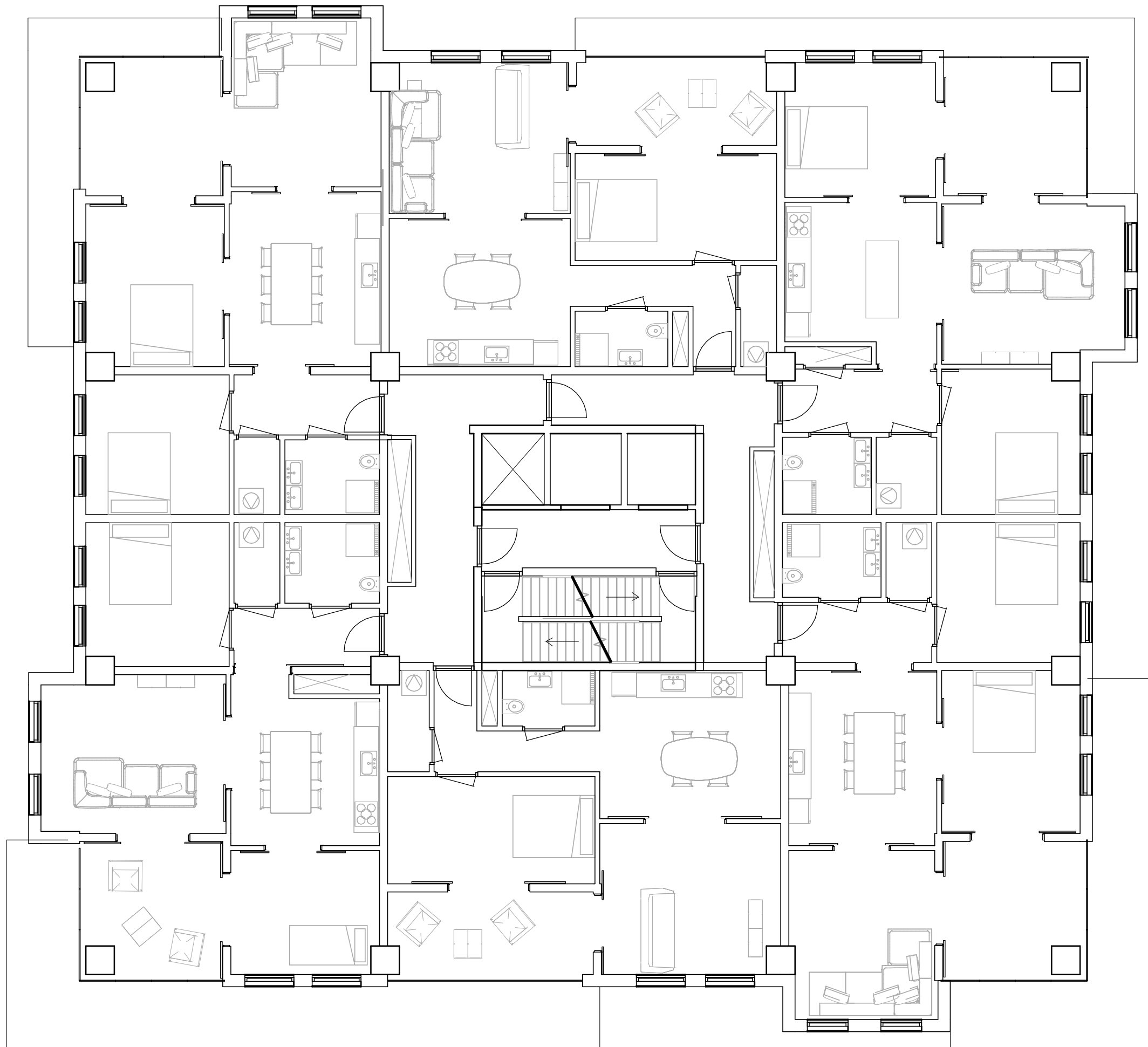
TOWER PLAN - 6 UNITS
