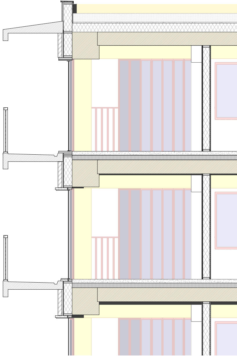
inside elevation 1:20
