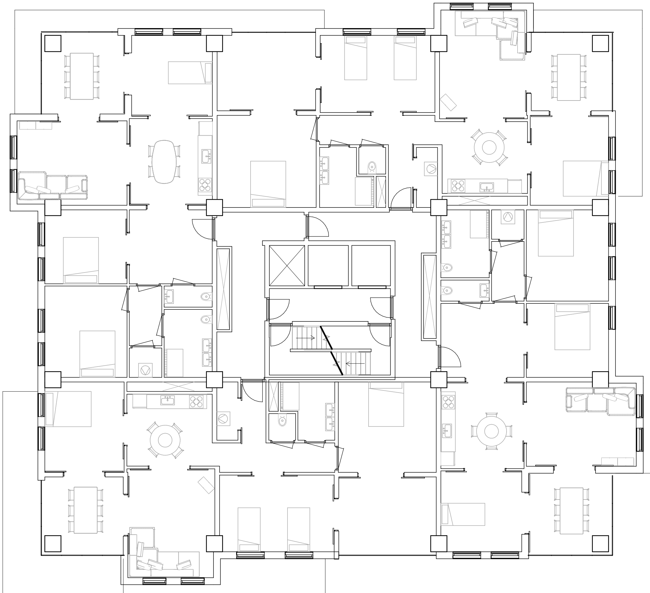
TOWER PLAN - 4 UNITS
