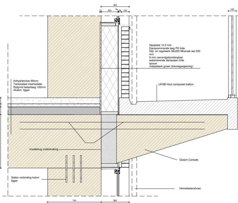
facade detail 1 : 10
