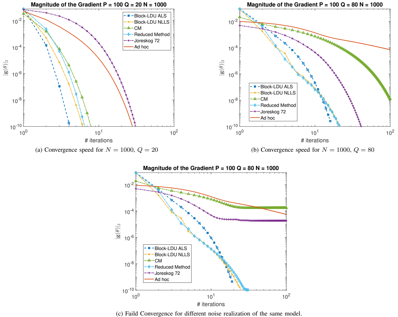
Fig. 1: Convergence for P = 100 sensors and varying number of samples N and sources Q .
