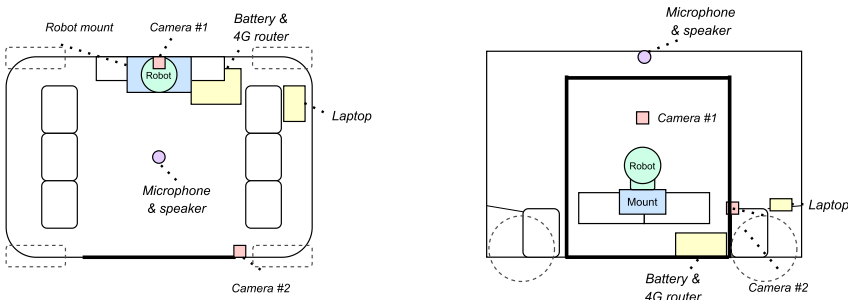
Fig. 6. A schematic of our experimental setup. Left : A top-down view. Right : A side view. The door of the bus is marked with a thicker line on the bottom-middle of the schematic, with the seats on the left and right side. The mount with the robot on top is visible in the middle, with the speaker and microphone in the ceiling of the bus. Miscellaneous equipment is on the floor and behind the passengers to the right.
