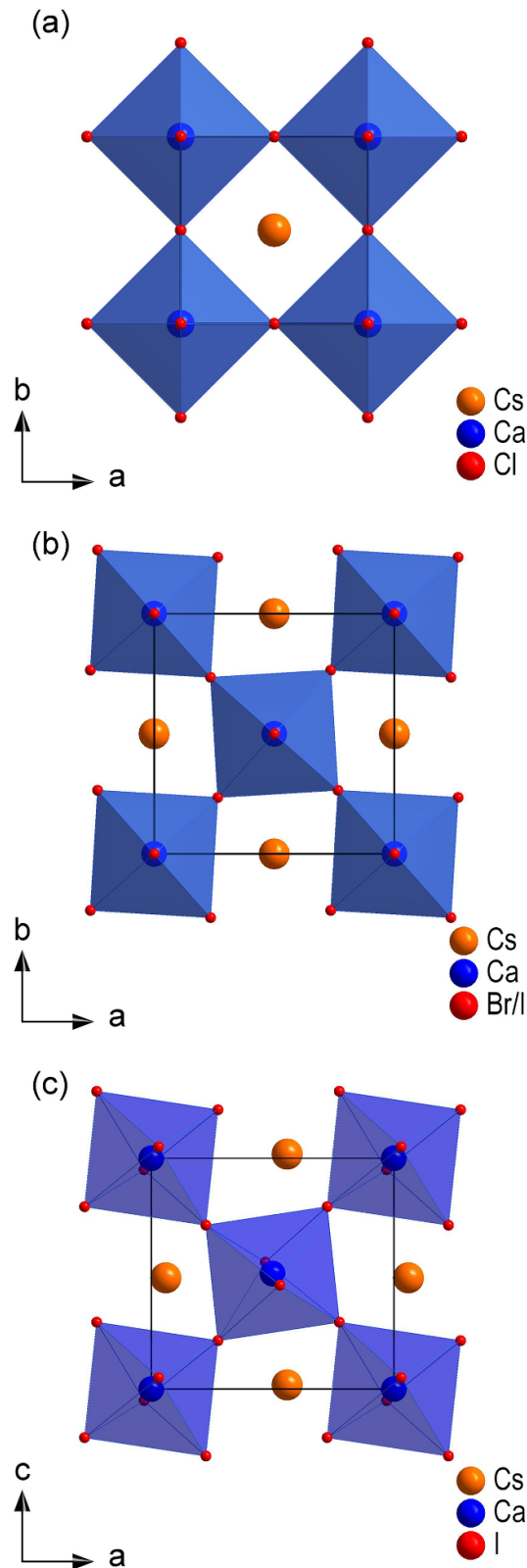
Figure 2. Crystal structures of (a) \text{CsCaCl}_3 , (b) \text{CsCaBr}_{1.2}\text{I}_{1.8} , and (c) \text{CsCaI}_3 that respectively adopt the structures of \text{CaTiO}_3 , \text{NaNbO}_3 , and \text{GdFeO}_3 type perovskites.
