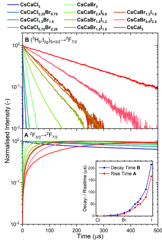
Figure 9. Room temperature decay curves of (^3\text{H}_6, t_{2g})_{S=3/2} \rightarrow ^2\text{F}_{7/2} emission B (top) and ^2\text{F}_{5/2} \rightarrow ^2\text{F}_{7/2} emission A (bottom) after laser excitation into the (^3\text{H}_6, t_{2g})_{S=1/2} levels. The curves of emission A display a clear risetime phenomena. The inset shows that its duration is close to the decay time of emission B.
