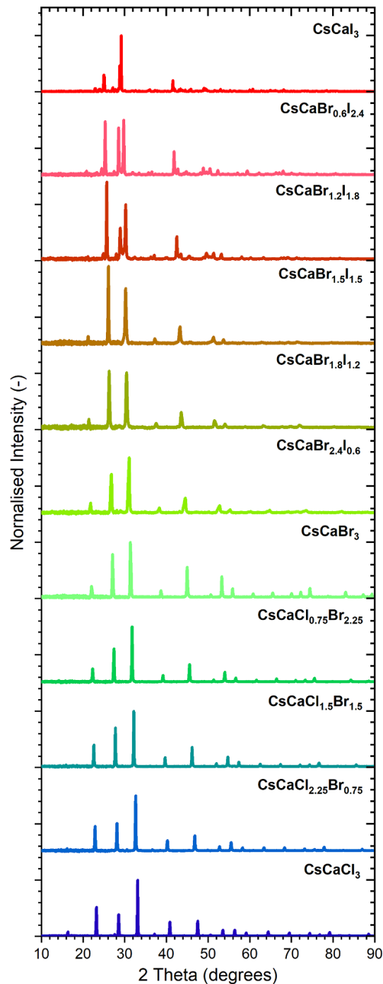
Figure 1. Powder x-ray diffraction patterns of the \text{CsCa}(\text{Cl/Br/I})_3\text{:Tm}^{2+} and \text{CsCa}(\text{Br/I})_3\text{:Tm}^{2+} samples at room temperature. The corresponding crystallographic data is summarised in table 1.
