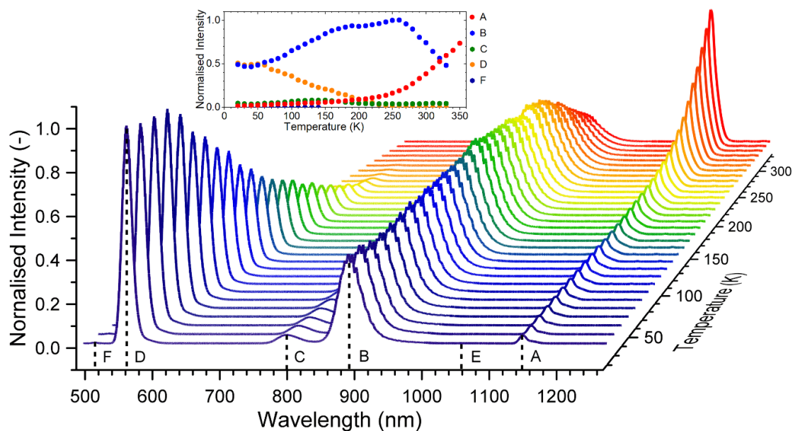
Figure 10. 3D-Plot showing the qualitative behaviour of the six \text{Tm}^{2+} emissions (A–F) in \text{CsCaI}_3:\text{Tm}^{2+} over temperature. The complementary inset presents the integrated luminescence signals over temperature and allows for a qualitative description of the observed trends. The spectra are corrected for the sensitivity of detection and normalised on the (^3\text{F}_4, t_{2g})_{S=3/2} \rightarrow ^2\text{F}_{7/2} emission D at 20 K. Photoexcitation occurred into the (^3\text{F}_4, t_{2g})_{S=1/2} levels at 455 nm.
