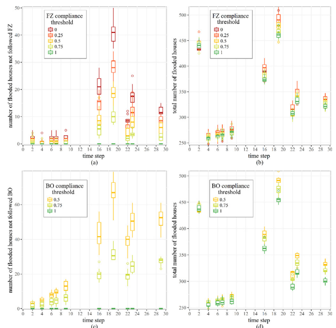
Fig. 4. The effects of FZ and BO on the number of flooded houses over time. (a) and (b) show the number of flooded houses that do not comply with the FZ and the total number of flooded houses, respectively, for FZ compliance thresholds between 0 and 1. For these figures, the BP and BO compliance thresholds are 0 and 0.5, respectively. (c) and (d) show the number of flooded houses that do not comply with the BO and the total number of flooded houses, respectively, for BO compliance thresholds between 0.5 and 1. For these figures, both the BP and FZ compliance thresholds are 0.
