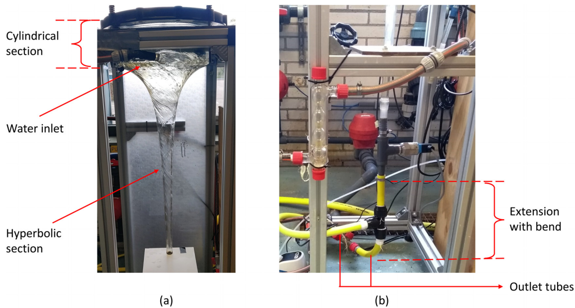
FIG. 1. Experimental setup divided into (a) funnel and (b) extension parts.
