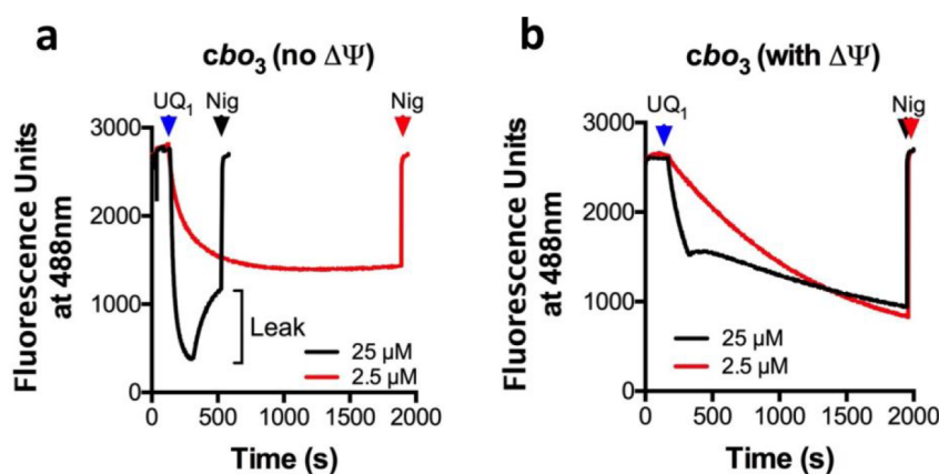
Figure 3. LAiR reveals regulatory mechanisms of cytochrome b 03 . a and b, Liposome acidification by reintegrated cbo 3 monitored by quenching of the ACMA fluorescence using the experimental system shown in Figure 1c. Typically, as protons are pumped into the proteoliposome lumen, an electrochemical gradient is formed across the membrane. Nigericin collapses any H + gradient completely. a, Proton pumping by cbo 3 in the presence of valinomycin. Valinomycin exchanges one K + for every H + entering the proteoliposome, thus abolishes ΔΨ (membrane potential) (i.e., absence of back-pressure on cbo 3 ); b, Proton pumping by cbo 3 in the absence of valinomycin (i.e., presence of increasing membrane potential and back-pressure on cbo 3 ). Various concentrations of Ubiquinol-1 (UQ 1 H 2 ) were used to start the reaction as shown. cbo 3 proteoliposomes were prepared using LAiR after a 30 min time period. For each experiment 3 biological replicates were performed with representative results shown.
