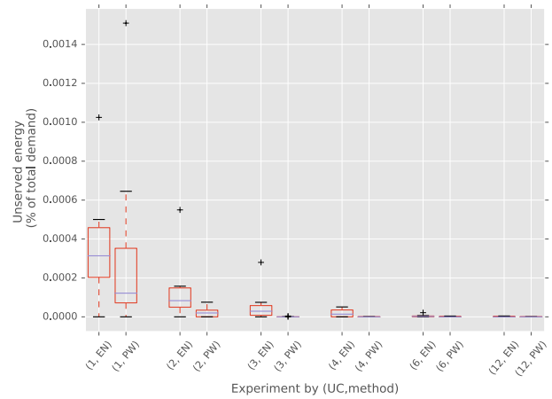
Fig. 7. Unserved energy in the DE system.
