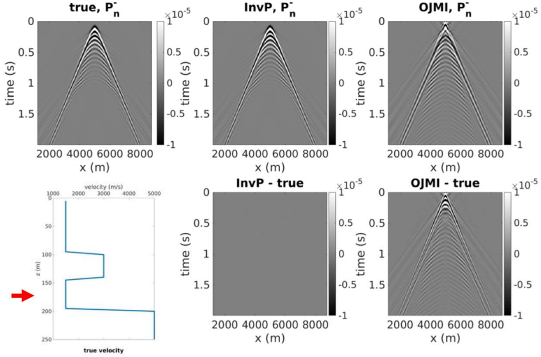
Figure 6. The situation when only internal multiples are considered and the maximum multiple order is 10. (Top left) The ground truth of the up-going and incoming wavefield p_n^- at z = 175 \text{ m} . (Top middle) The reconstructed up-going and incoming wavefield \widetilde{p}_n^- at z = 175 \text{ m} via the inverse propagation of the surface wavefield p_n^-(0) . (Top right) The reconstructed up-going and incoming wavefield \widetilde{p}_n^- at z = 175 \text{ m} via the backward propagation scheme used in the traditional JMI (OJMI). (Bottom left) The true 1.5D velocity with the red arrow pointing at the target subsurface interface. (Bottom middle) The difference between the reconstructed wavefield via the inverse propagation and the ground truth. (Bottom right) The difference between the reconstructed wavefield via the backward propagation and the ground truth.
