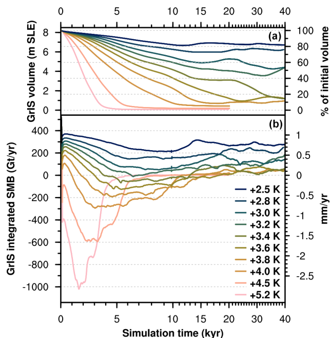
Figure 2. Time series of (a) GrIS volume and (b) integrated surface mass balance for the main runs presented in this study. Note that simulation time on the x axis is irregular (minor tick marks every 1000 years).
