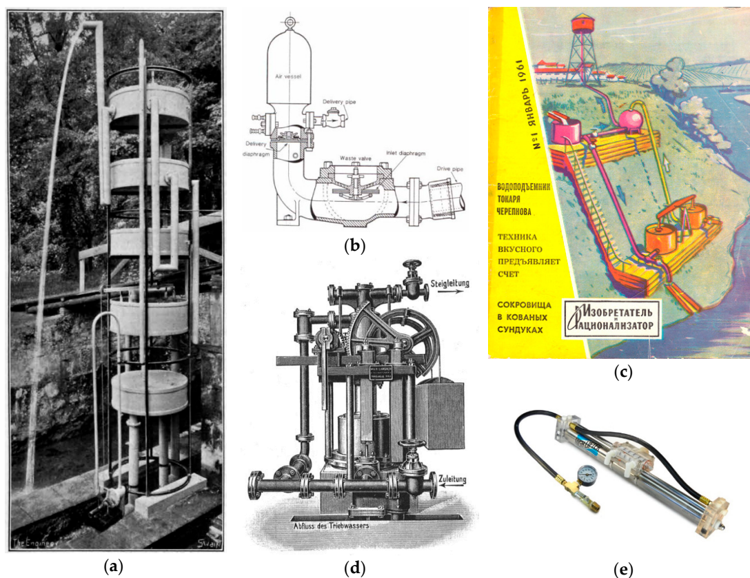
Figure 3. Different types of hydro-pneumatic water lifters: (a) Hydraumat [77]. © Grace's Guide Ltd. ( https://www.gracesguide.co.uk/The_Engineer_1922/07/07 ). CC BY-SA 4.0; (b) Scheme of an hydraulic ram pump (HRP) [78]. Reproduced with permission from Jeremy Milln. © The National Trust ( https://industrial-archaeology.org/wp-content/uploads/2016/04/AIA-News-93-Summer-1995.pdf ); (c) Illustration of the Cherepnov water lifter (CWL) installed at the former Gorky Oblast, Russia [75,79]. Reproduced with permission from “Inventor and Innovator” magazine. © Изобретатель и рационализатор ( http://i-r.ru/article/2254/ ); (d) Early model of Lambach pump (LP) [62]. © Hauptverein Deutscher Ingenieure in der Tschechoslowakischen Republik; (e) High lifter [80]. Reproduced with permission from Humboldt Solar Water Pump. © Humboldt Solar Water Pump ( http://www.humboldtsolarwaterpump.com/high-lifter-gravity-water-pump-for-your-off-grid-water-system/ ).
