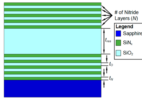
Figure 4. Structure of a Fabry–Perot interferometer using 9-layer distributed Bragg reflectors with \text{SiN}_x ( t_H = t_N ) as the high-index material and \text{SiO}_2 as the low-index material ( t_L = t_O ).
