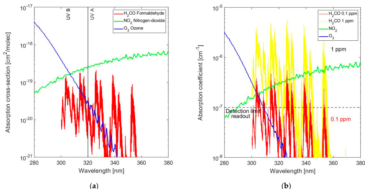
Figure 1. (a) Absorption cross-sections of formaldehyde (H 2 CO) and the two main interfering gases in near-UV: NO 2 and O 3 ; (b) Absorption coefficient of formaldehyde at 0.1 ppm and 1 ppm concentrations in the presence of NO 2 and O 3 in their concentrations in the lower atmosphere.
