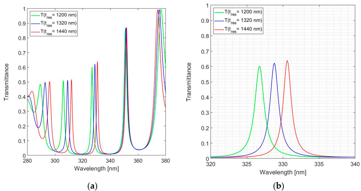
Figure 10. Calculated spectral transmittance for the 19-layer FPI with \text{SiN}_{1.49} used for n_H : (a) Full near-UV spectral range and (b) zoom in around the design wavelength.
