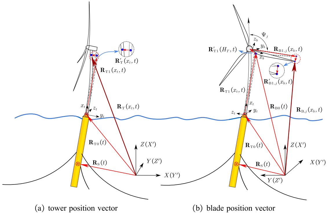
Fig. 2. FOWT tower (a) and blade (b) flexibility and deformation.
