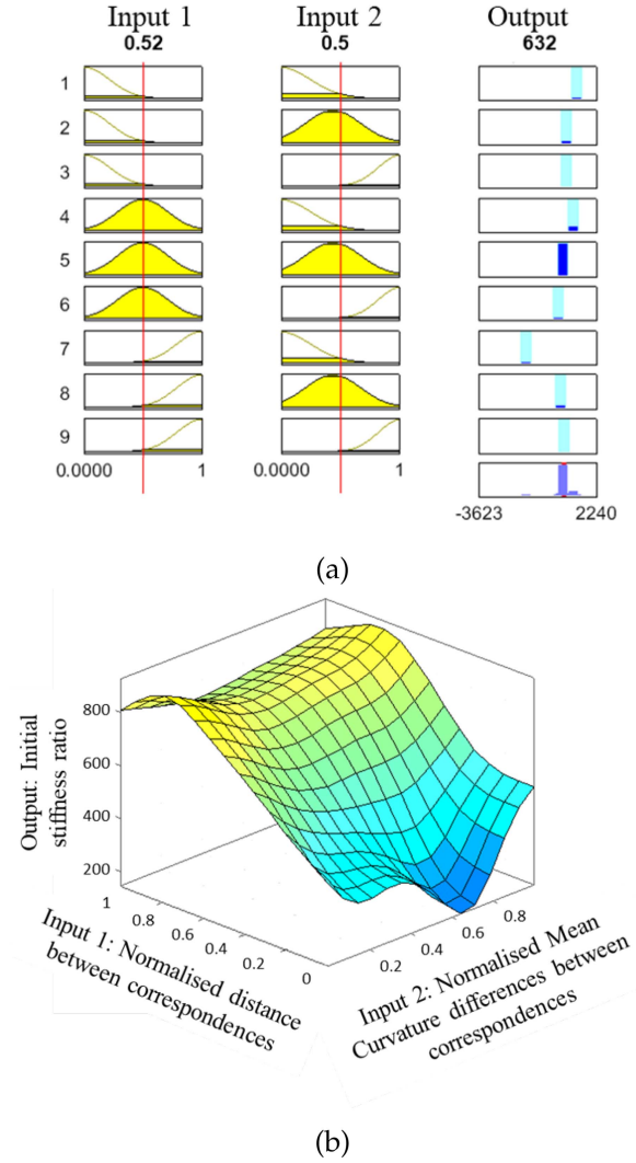
Fig. 6. ANFIS model. (a) Fuzzy rules. (b) Fuzzy surfaces for the intelligent estimator.
