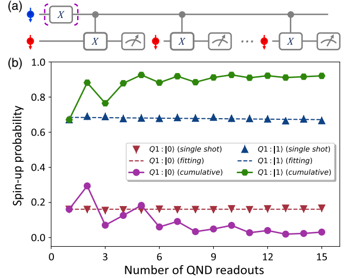
FIG. 2. (a) Circuit diagram for the repetitive QND readout scheme, using the same labels as in Fig. 1(c). (b) Spin-up probability obtained from individual QND readout cycles (triangles) and from a cumulative weighted majority vote (circles) for preparation of Q1 in state |1\rangle (blue) and in state |0\rangle (red). For the individual readout cycles, the visibility does not improve and in fact slightly decreases due to the finite relaxation time T_1 of Q1 . By fitting the measured P_1 for preparation of Q1 in state |1\rangle to an exponential, we estimate T_1 = 1.8 \pm 0.6 s. The cumulative weighted majority vote improves the logical readout visibility as more QND readout cycles are performed.
