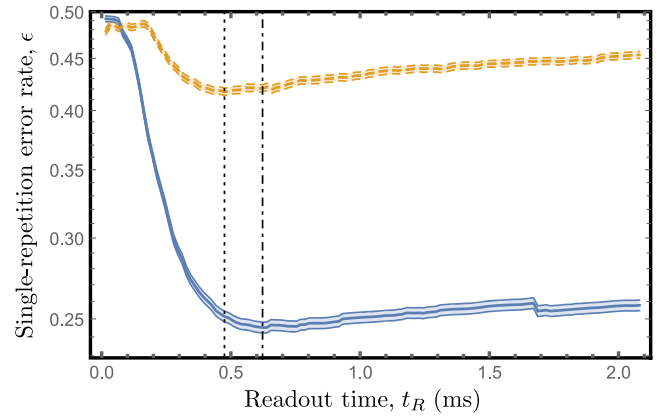
FIG. 4. Average single-repetition readout error rate \epsilon as a function of readout time t_R in the absence of added noise (solid blue line) and in the presence of added noise (dashed yellow line). The optimal readout time in the absence (presence) of added noise is indicated by the dot-dashed (dotted) line. In both cases, the shaded areas give the statistical uncertainty (see text). Finally, we note that the small discontinuity in the blue curve at t_R \approx 1.7 ms is a consequence of the finite histogram bin size and has no particular physical significance.
