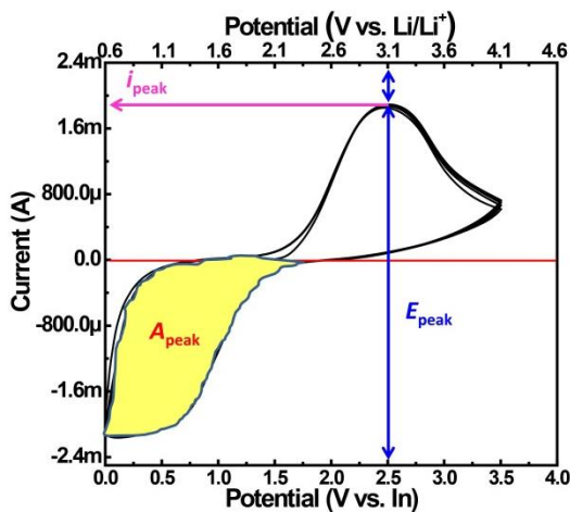
Figure 2.10: CV profiles of \text{Li}_2\text{S}/\text{Li}_6\text{PS}_5\text{Br}/\text{In} all-solid-state lithium batteries with a scan rate of 0.5 mV/s at room temperature.
