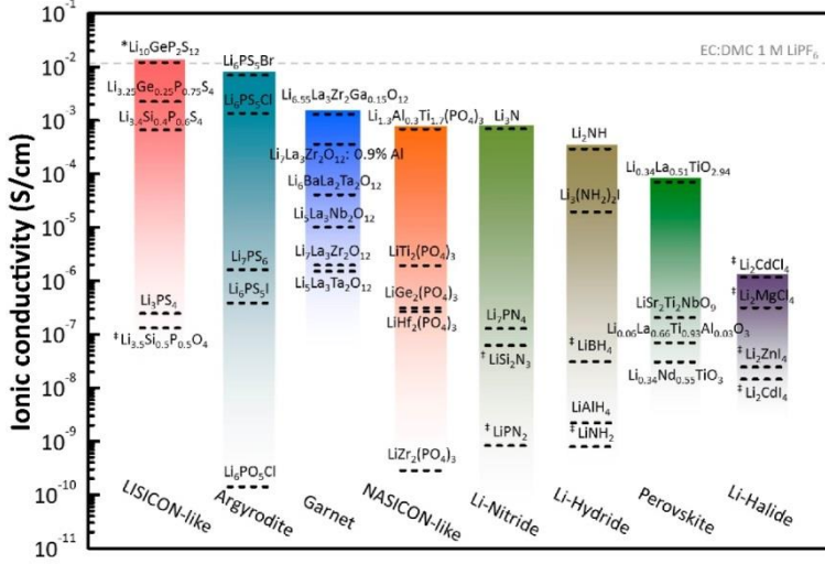
Figure 1.3: Lithium ion conductivity for published lithium-ion conductors. 4
