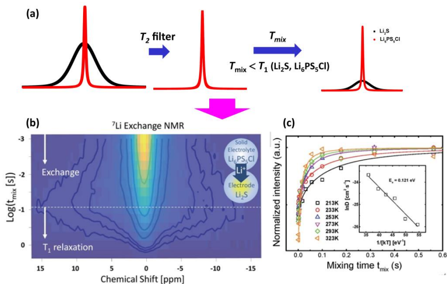
Figure 2.9: (a) Schematic of the 1D EXSY NMR experiment for Li 2 S and Li 6 PS 5 Cl mixture. (b) 2D 7 Li- 7 Li NMR exchange experiment probing the Li-ion transport from the electrolyte Li 6 PS 5 Cl phase to the electrode Li 2 S phase at room temperature. (c) Normalized intensity of the static Li 2 S 7 Li NMR spectrum, T_1 corrected, as a function of mixing time at different temperatures. The inset shows the temperature dependence of the diffusion parameter D , derived from the fits representing the diffusion model, see text. An Arrhenius law is used to fit the activation energy, E_a , representing the diffusion process over the boundary between the Li 6 PS 5 Cl solid electrolyte and the Li 2 S phases.
