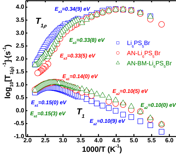
Figure 5.5: Temperature dependence of the ^7\text{Li} spin-lattice relaxation NMR rates T_{1(\rho)}^{-1} measured in both the laboratory and the rotating frame of reference for the \text{Li}_6\text{PS}_5\text{Br} , \text{AN-Li}_6\text{PS}_5\text{Br} and \text{AN-BM-Li}_6\text{PS}_5\text{Br} materials. The Larmor frequency is 155.506 MHz ( T_1^{-1} ) and the spin lock frequency is 20 kHz ( T_{1\rho}^{-1} ).
