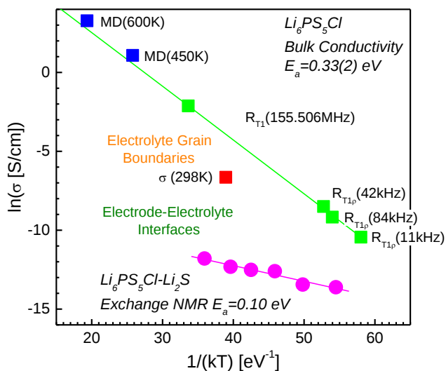
Figure 4.6: Li-ion conductivity in \text{Li}_6\text{PS}_5\text{Cl} deduced from the DFT based MD simulations, ^7\text{Li} Solid state NMR SLR experiments, 1D exchange experiments between the \text{Li}_2\text{S} electrode and \text{Li}_6\text{PS}_5\text{Cl} solid electrolyte and the room temperature impedance measurements.
