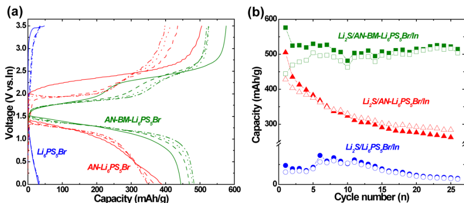
Figure 5.7: (a) Galvanostatic voltage curves for the first 4 cycles of the assembled nano- \text{Li}_2\text{S}/\text{Li}_6\text{PS}_5\text{Br} ( \text{Li}_6\text{PS}_5\text{Br} or \text{AN-Li}_6\text{PS}_5\text{Br} or \text{AN-BM-Li}_6\text{PS}_5\text{Br} )/In solid-state batteries at a current density of 0.064 \text{ mA}/\text{cm}^2 applied between 0 and 3.5 V vs. In (0.62 - 4.12 V vs. \text{Li}^+/\text{Li} ). The solid, dashed, dotted and dashed dotted lines represent cycles 1-4 respectively. (b) Capacity retention cycling of the solid-state batteries at a current density of 0.064 \text{ mA}/\text{cm}^2 applied between 0 and 3.5 V vs. In (0.62 - 4.12 V vs. \text{Li}^+/\text{Li} ).
