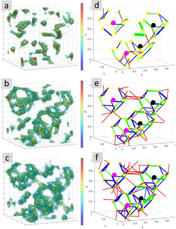
Figure 4.3: (a-c) The integrated Li-density of the Molecular Dynamics Simulations ( 10^{-10} second duration) in \text{Li}_6\text{PS}_5\text{Cl} at (a) 300 K, (b) 450 K and (c) 600 K. (d-f) Jump statistics derived from the Molecular Dynamics Simulations at (d) 300 K, (e) 450 K and (f) 600 K.
