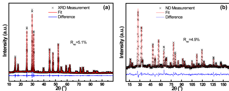
Figure 3.4: (a) X-ray Powder and (b) Neutron Powder diffraction pattern of Li_6PS_5Cl at room temperature (after annealing at 550 °C for 5 h) simultaneously refined by Rietveld refinement.
