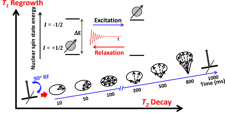
Figure 2.7: The evolution of the magnetization after it has been flipped by 90° pulse. The longitudinal and transverse are the regrowth process of the T_1 and the T_2 decay.
