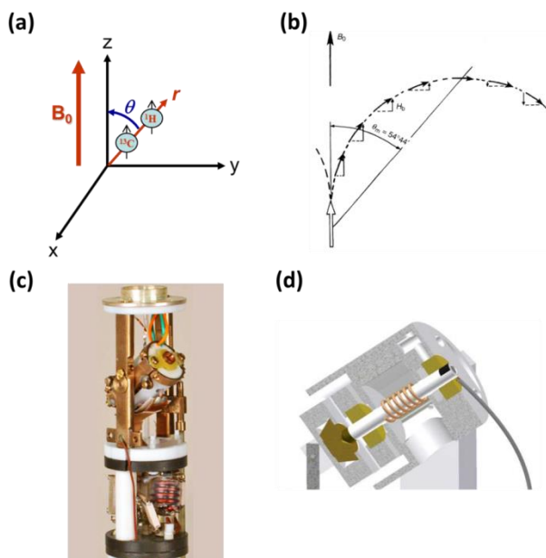
Figure 2.6: (a) The dipolar coupling between C and H. (b) Simulate a uniform distribution of magnetic moments in a powder by spinning the sample very fast at 54.74^\circ . (c) MAS probe. (d) The rotor in an MAS probe.
