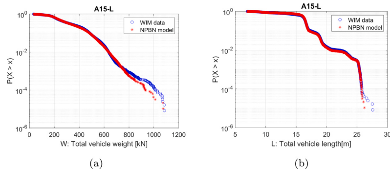
Fig. 7. Exceedance probability plots comparison between variables of interest ( W and L ) generated by the NPNB model and the WIM data in highway A15-L: (a) Total vehicle weight distribution [kN] for original data and data generated with NPNB model. (b) Total vehicle length distribution [m] for original data and data generated with NPNB model.
