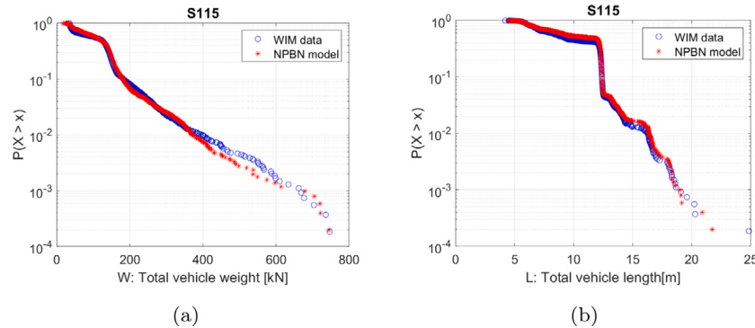
Fig. 10. Comparison between variables of interest generated by the NPNB model and the WIM data in S115 location: (a) Total vehicle weigh distribution [kN] for original data and data generated with the NPNB model, (b) Total vehicle length distribution [m] for original data and data generated with the NPNB model.
