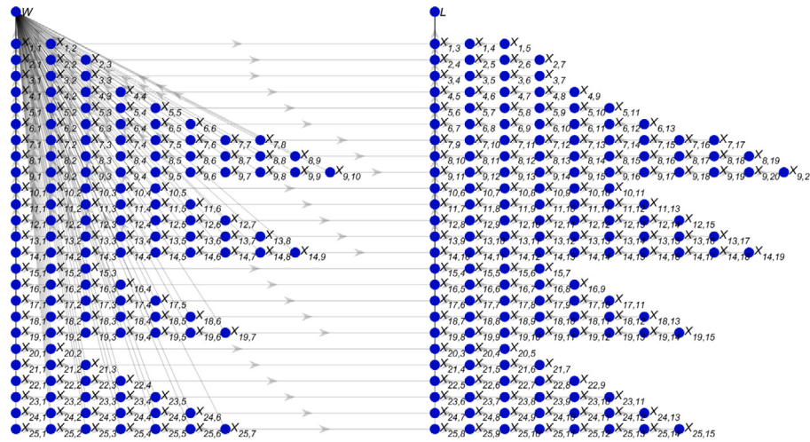
Fig. 3. BN model for A15-L highway of the WIM system in the Netherlands. The left side of the network represents the X_{i,j} axle loads. The right side represents the vehicle length X_{i,i+1} and the inter-axle distances X_{i,i+1} .
