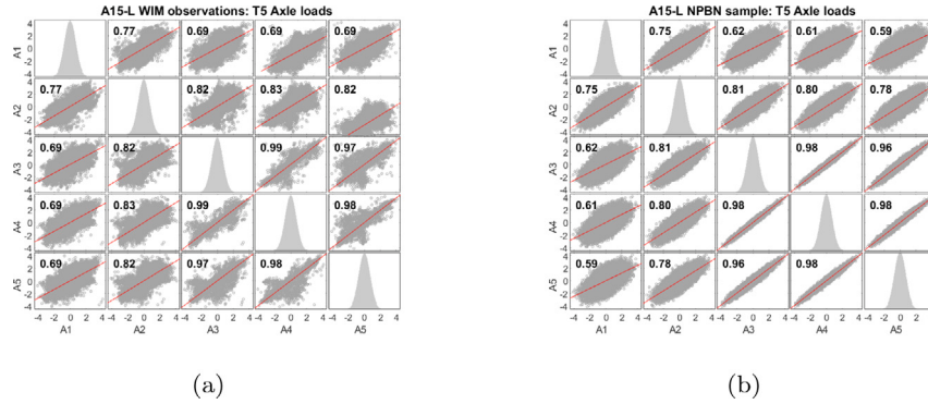
Fig. 5. Comparison between axle loads generated by the NPNB model and the WIM data of the T5 vehicle type in highway A15-L: (a) Correlation matrix for the empirical data standard transformed; (b) Correlation matrix for the synthetic data standard transformed.
