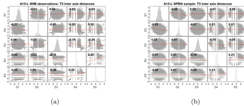
Fig. 6. Comparison between inter axle distances generated by the NPNB model and the WIM data of the T5 vehicle type in highway A15-L: (a) Correlation matrix for the empirical data standard transformed; (b) Correlation matrix for the synthetic data standard transformed.
