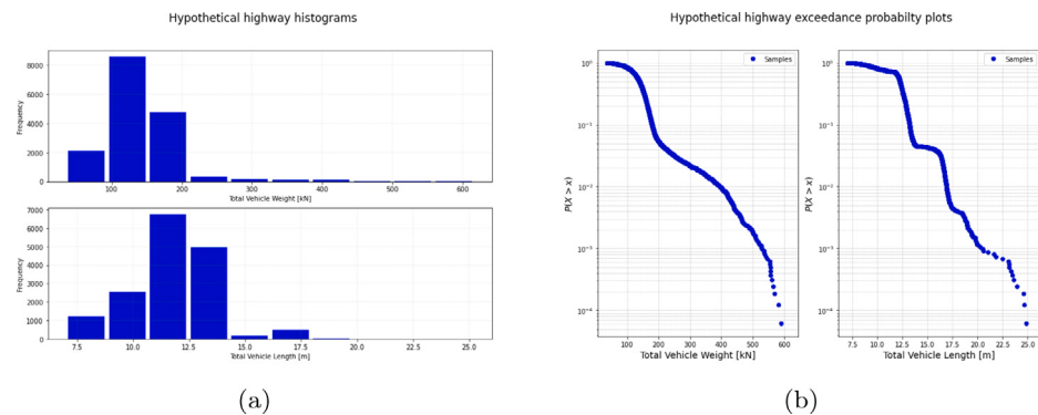
Fig. 14. NPNB WIM GUI output: (a) W and L histograms. (b) W and L exceedance probability plots.
