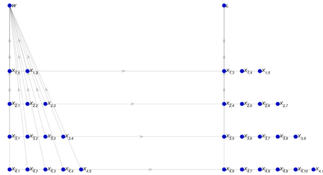
Fig. 9. NPNB model for S115 road WIM location. The left side of the network represents the X_{i,j} axle loads. The right side represents the vehicle length X_{i,n_{i+1}} and the inter axle distances X_{i,n_{i+1}+1,j} .
