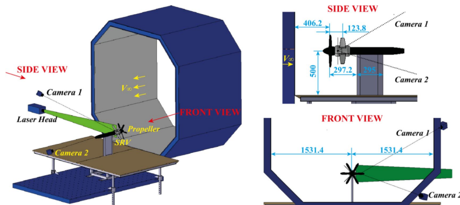
Fig. 9 Sketch of the experimental setup in the wind tunnel including a sketch of the PIV measurement setup (dimensions in millimeters).
