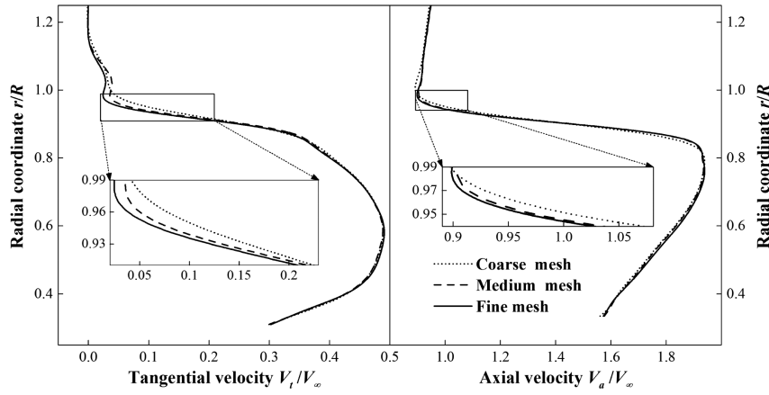
Fig. 5 Comparison of computed circumferentially averaged tangential and axial velocity distributions from different meshes at J = 0.6 .
