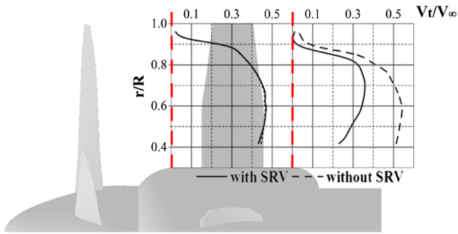
Fig. 14 Quantification of swirl recovery by SRVs from PIV measurements at J = 0.6 .
