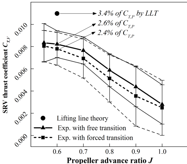
Fig. 10 Time-averaged propulsive performance of the SRVs measured with the load cells. LLT denotes the result computed with lifting-line theory.
