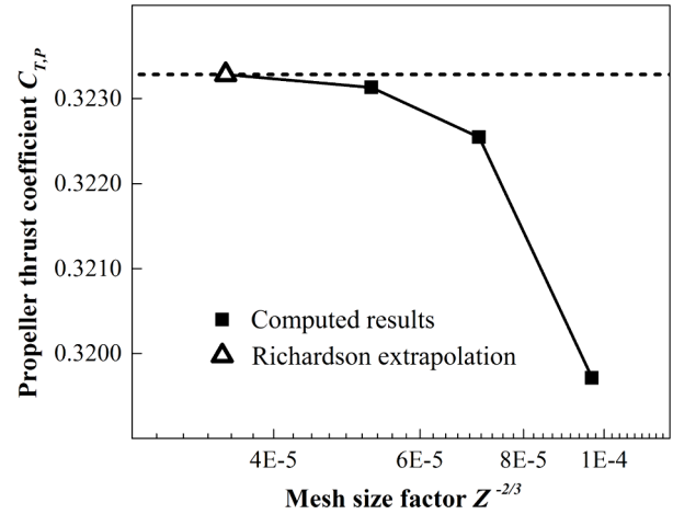
Fig. 4 Result of the mesh refinement study showing the propeller thrust coefficient as function of the mesh size factor Z .
