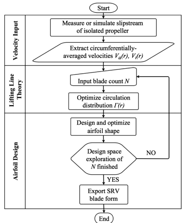
Fig. 1 Framework of the SRV design procedure.
