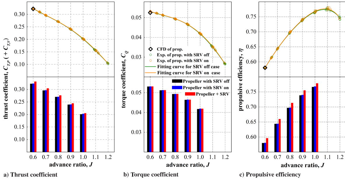
Fig. 12 Propulsive performance of the propulsion system with and without the SRVs installed.
