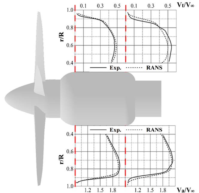
Fig. 13 Validation of the input velocities from RANS simulation of the propeller at J = 0.6 .
