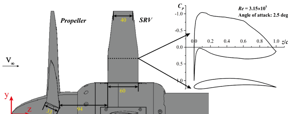
Fig. 8 Sketch of the propeller, the designed SRVs, and the coordinate system (dimensions in millimeters).
