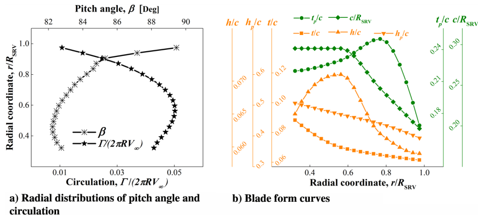
Fig. 7 Blade form curves of SRVs designed with vane count N of 4.
