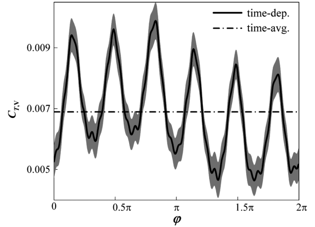
Fig. 11 Unsteady propulsive performance of one SRV at J = 0.6 without transition strip measured using the load cell. The 95% confidence level is indicated by the gray area.
