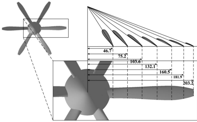
Fig. 2 Propeller layout (dimensions in millimeters).
