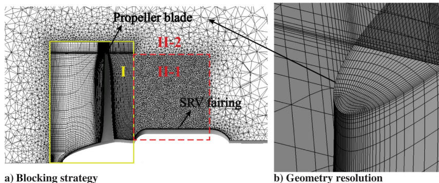
Fig. 3 Hybrid computation mesh for the isolated propeller.
