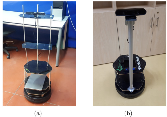
Fig. 4. Mobile robots TurtleBot 2 used in the experiments: (a) at the Carlos III University in Madrid, (b) at the Czech Technical University in Prague.
