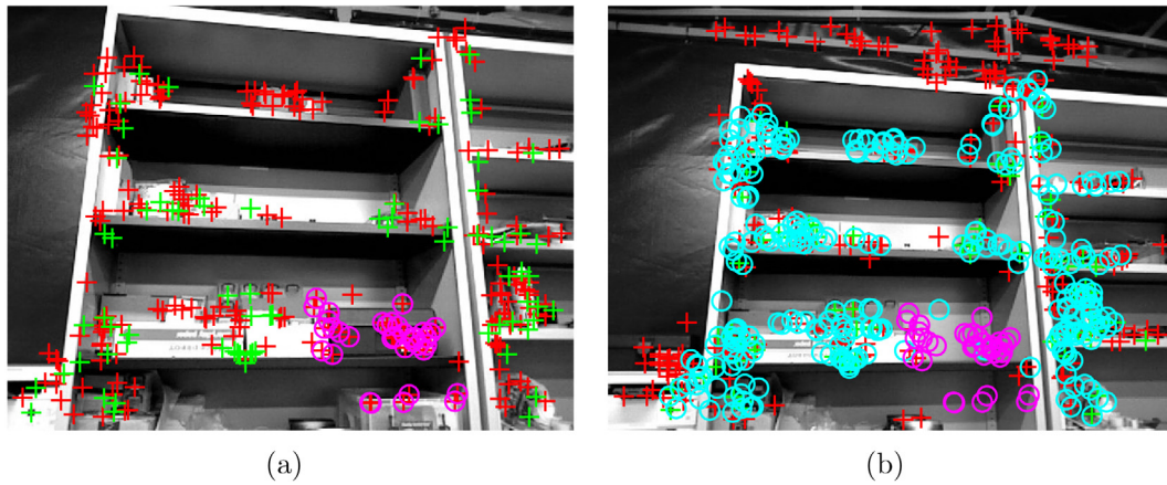
Fig. 3. A database image (a) and a query image with one object missing on the third shelf from the top (b). The crosses represent the features in both images. Tentative correspondences found by the matching algorithm are shown in green. The cyan circles show the transformations of the features from the database image to the query image. The magenta circles show the features that were identified as a change. (For interpretation of the references to color in this figure legend, the reader is referred to the web version of this article.)
