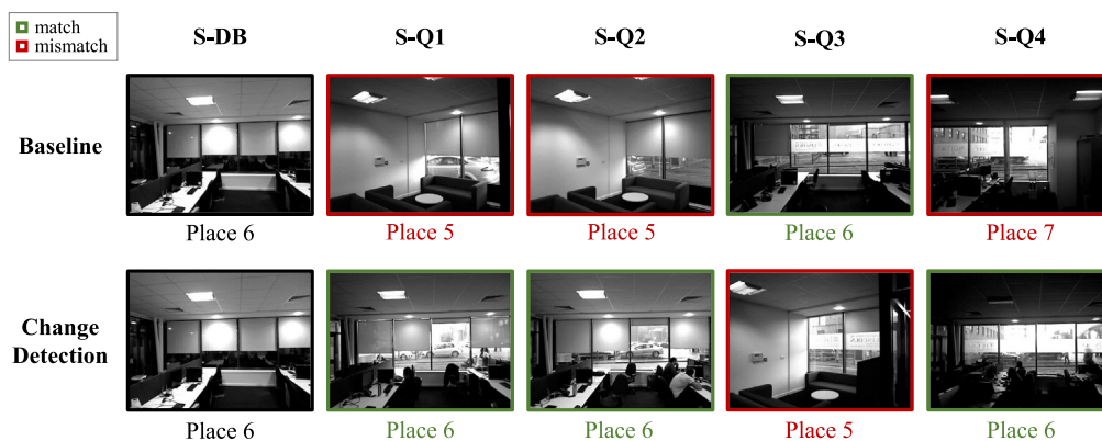
Fig. 10. Examples of images matched by the baseline method and using the change detection. The figure shows successful matches (S-Q1, S-Q2, S-Q4) as well as a localization failure (S-Q3) when using the change detection method.
