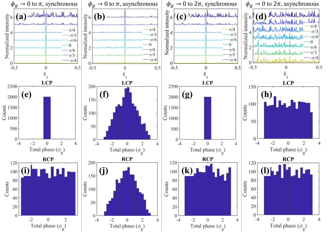
FIG. 3. The polarization-controlled tuning of momentum-space intensity distribution in synchronous and asynchronous systems. (a)–(d) The elliptical polarization states ([1, e^{i\delta}]^T , ellipticity \delta/2 is mentioned in legends) were used to actively tune the momentum-space intensity distribution from the asymmetric random scattering system for an input Gaussian beam of width 80d (the intensities are shifted for better visualization). The spatially disordered system was taken such that the geometric phase [\pm\phi_g(x), +(-) for RCP (LCP) polarization of light] of the transmitted light is uniformly distributed between (a), (b) -\pi/2 to \pi/2 and (c), (d) \pi to 2\pi . The momentum-space intensity distribution for (a), (c) synchronous [\phi_d(x) = \phi_g(x)] , and (b), (d) asynchronous [\phi_d(x) is distributed in same manner as \phi_g(x)] systems. The extraordinary spin-selective modes are observed for the synchronous systems. (e)–(l) The total phase-frequency distributions for LCP and RCP states are given below the corresponding normalized intensity distributions of the disordered medium.
