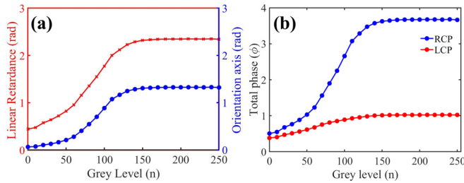
FIG. 8. The dependence of (a) polarization parameters and (b) the total phase ( \phi_d \pm \phi_g ) occupied by the light transmitted for input LCP and RCP polarization states of light on the gray level projected onto the SLM (adapted from Ref. [6]).
