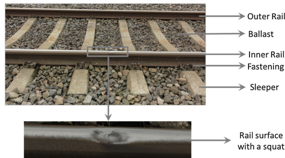
Fig. 5. A severe squat on the rail surface.
