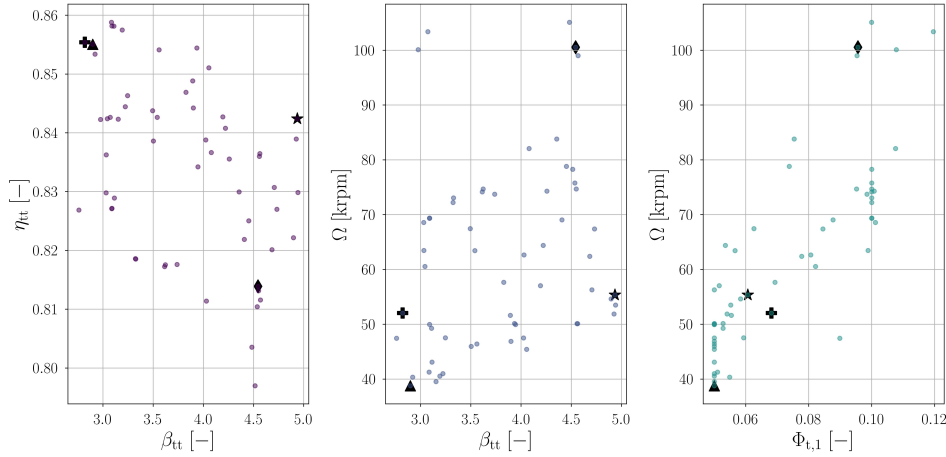
Figure 6.11: Variation of compressor efficiency and rotational speed as a function of pressure ratio, and variation of rotational speed as a function of swallowing capacity established over the Pareto front computed with the data-driven model. The markers identify the optimal solutions reported in Tab. 6.5.
