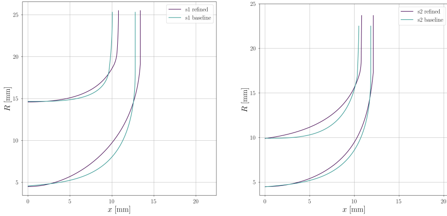
Figure 3.7: Meridional channel of the first (left chart) and second (right chart) stage of the compressor prototype obtained as a result of the second design iteration.
