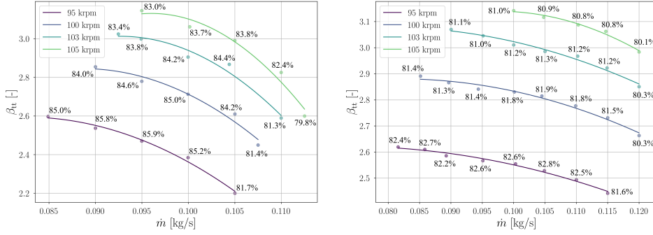
Figure 3.14: Predicted operating map of the first (left) and second (right) IRIS compressor stage obtained as an outcome of the second design iteration. The stage performance is computed with CFD accounting only for the presence of the impeller and the vaneless diffuser. The results are reported in terms of mass-flow averaged \beta_{tt} and \eta_{tt} .
