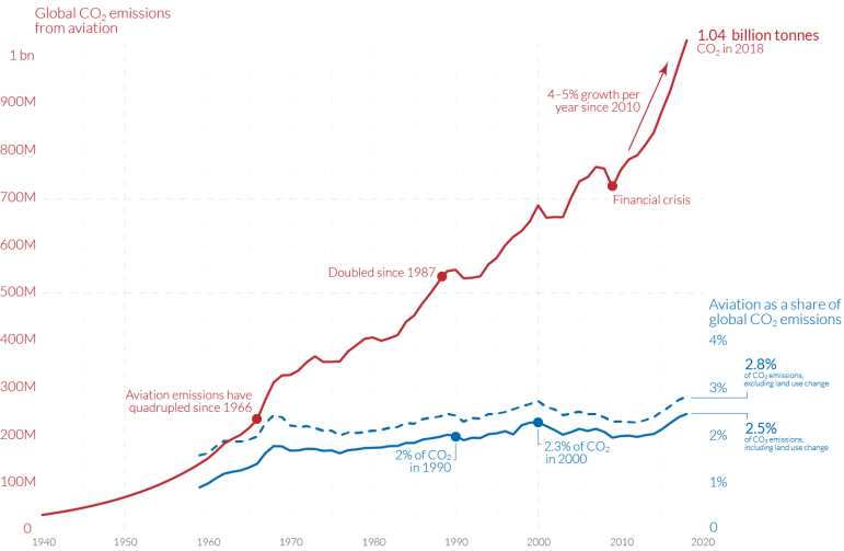
Figure 1.1: Historical evolution of global CO 2 emissions from aviation prior to the COVID-19 pandemic [12]. The emissions include passenger air travel, freight, and military operations.
