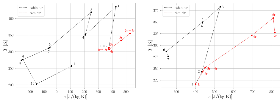
Figure 1.3: Thermodynamic diagram of an exemplary bleedless three-wheel bootstrap air cycle machine sized for an Airbus A320, operating on the ground (left) and in cruise conditions (right).
