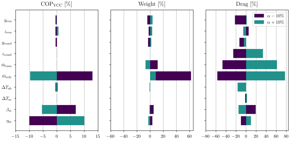
Figure 6.12: Sensitivity of the objective functions with respect to a \pm 10\% perturbation in the vector of design variables.
