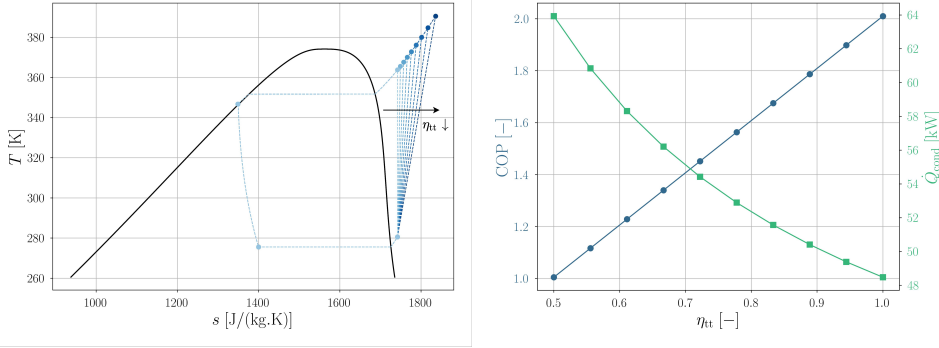
Figure 1.9: Influence of the compressor efficiency on the performance of an exemplary single-pressure level VCC system. The pressure ratio and the refrigerant mass flow rate are set to \beta_{tt} = 8 and \dot{m} = 0.35 kg/s, whereas the evaporation and condensation temperatures are equal to T_{eva} = 275.6 K and T_{cond} = 351.8 K, respectively.
