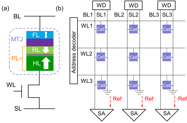
Fig. 1: (a) MTJ stack and 1T-1M cell, (b) STT-MRAM array.
