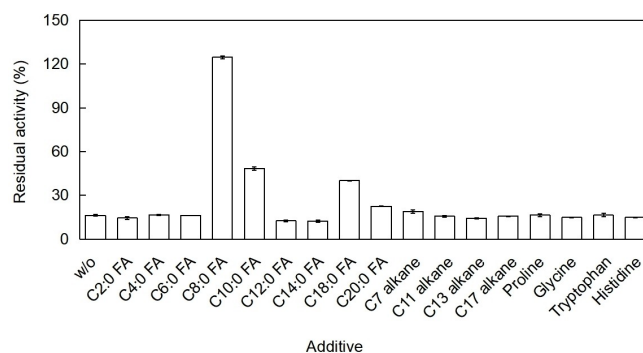
Figure 4. Influence of additive on the photostability of purified CvFAP. Incubation condition: [CvFAP] = 18 \mu M, buffer: 100 mM Tris-HCl (pH 8.5), [DMSO] = 5 vol%, light intensity of blue light = 14.5 \mu EL -1 s -1 , T = 30 °C, pre-illumination time = 2 h, [additive] = 10 mM. Activity assay conditions: [palmitic acid] 0 = 13 mM, [DMSO] = 30 vol%, buffer: 100 mM Tris-HCl (pH 8.5), [CvFAP] = 3–6 \mu M, light intensity of blue light = 14.5 \mu EL -1 s -1 , T = 37 °C, reaction time = 30 min. Data represent the mean \pm SD of two independent experiments.
