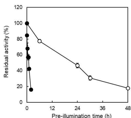
Figure 2. Comparison of photochemical inactivation of CvFAP as purified enzyme (●) and crude cell extract preparation (○). Incubation conditions: [CvFAP] = 18 \mu M, buffer: 100 mM Tris-HCl (pH 8.5), light intensity of blue light = 14.5 \mu EL -1 s -1 , T = 30 °C. Activity assay conditions: [palmitic acid] 0 = 13 mM, [DMSO] = 30 vol%, buffer: 100 mM Tris-HCl (pH 8.5), [CvFAP] = 3–6 \mu M, light intensity of blue light = 14.5 \mu EL -1 s -1 , T = 37 °C, reaction time = 30 min. Data represent the mean \pm SD of two independent experiments.
