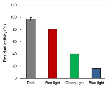
Figure 3. Residual activity of purified CvFAP illuminated under different wavelength of LEDs. Incubation conditions: [CvFAP] = 18 \mu M, buffer: 100 mM Tris-HCl (pH 8.5), protected from light or illuminated by different colour of light, T = 30 °C, pre-illumination time = 2 h. Activity assay conditions: [palmitic acid] 0 = 13 mM, [DMSO] = 30 vol%, buffer: 100 mM Tris-HCl (pH 8.5), [CvFAP] = 3–6 \mu M, light intensity of blue light = 14.5 \mu EL -1 s -1 , T = 37 °C, reaction time = 30 min. Data represent the mean \pm SD of two independent experiments.
