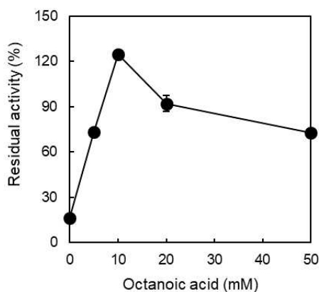
Figure 5. Influence of additive on the photostability of purified CvFAP. Incubation condition: [CvFAP] = 18 \mu M, buffer: 100 mM Tris-HCl (pH 8.5), [DMSO] = 5 vol %, light intensity of blue light = 14.5 \mu EL -1 s -1 , T = 30 °C, incubation time = 2 h, [caprylic acid] = 0–50 mM. Activity assay conditions: [palmitic acid] 0 = 13 mM, [DMSO] = 30 vol %, buffer: 100 mM Tris-HCl (pH 8.5), [CvFAP] = 3 \mu M, light intensity of blue light = 14.5 \mu EL -1 s -1 , T = 37 °C, reaction time = 30 min. Data represent the mean \pm SD of two independent experiments.
