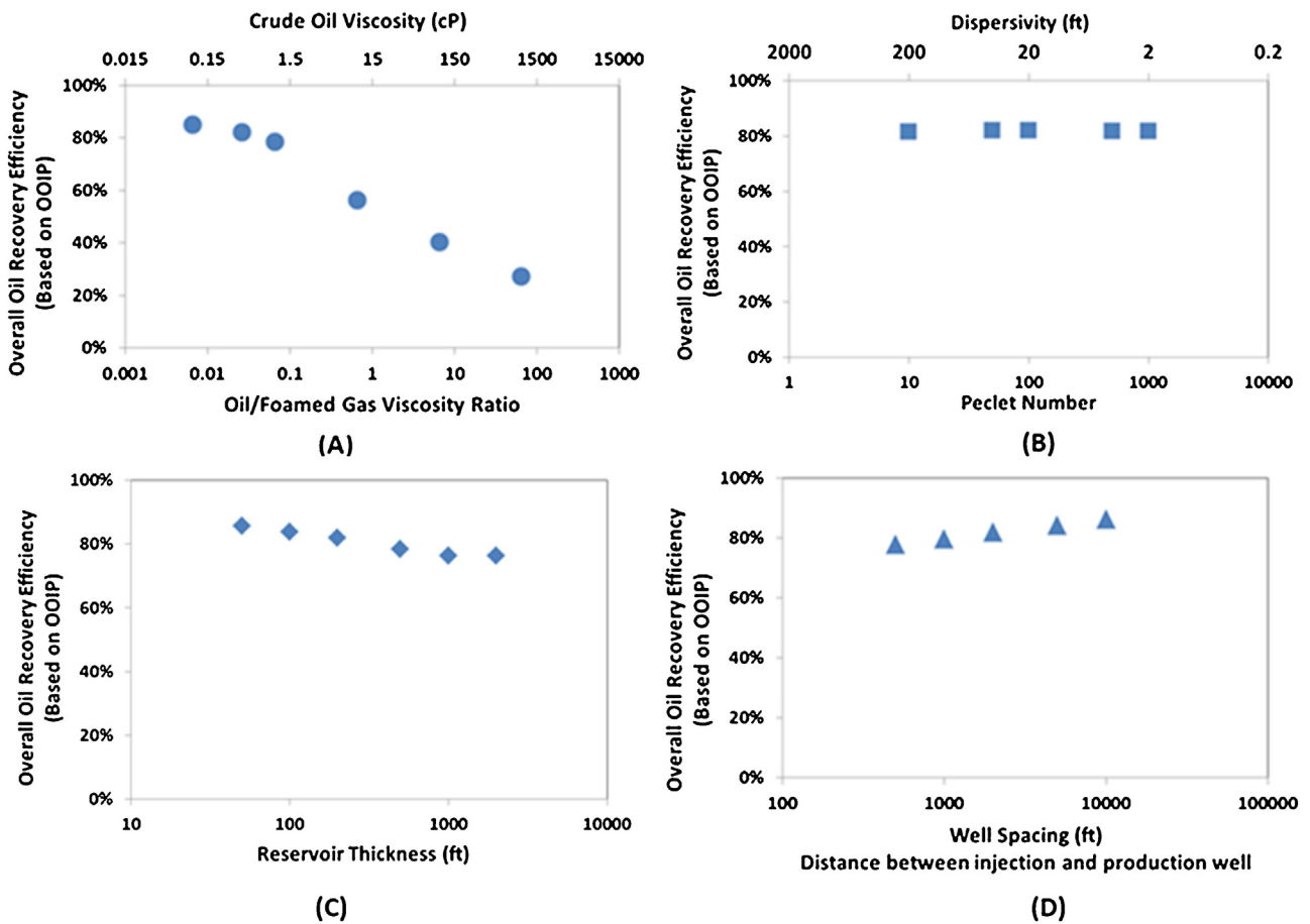
Fig. 11. Sensitivity analysis: (A) Overall oil recovery efficiency as function of crude oil viscosity and oil/foamed gas viscosity ratio. (B) Overall oil recovery efficiency as function of Pelet number and dispersivity of the surfactant. (C) Overall oil recovery efficiency as function of reservoir thickness. (D) Overall oil recovery efficiency as function of well spacing (distance between injection and production wells).
