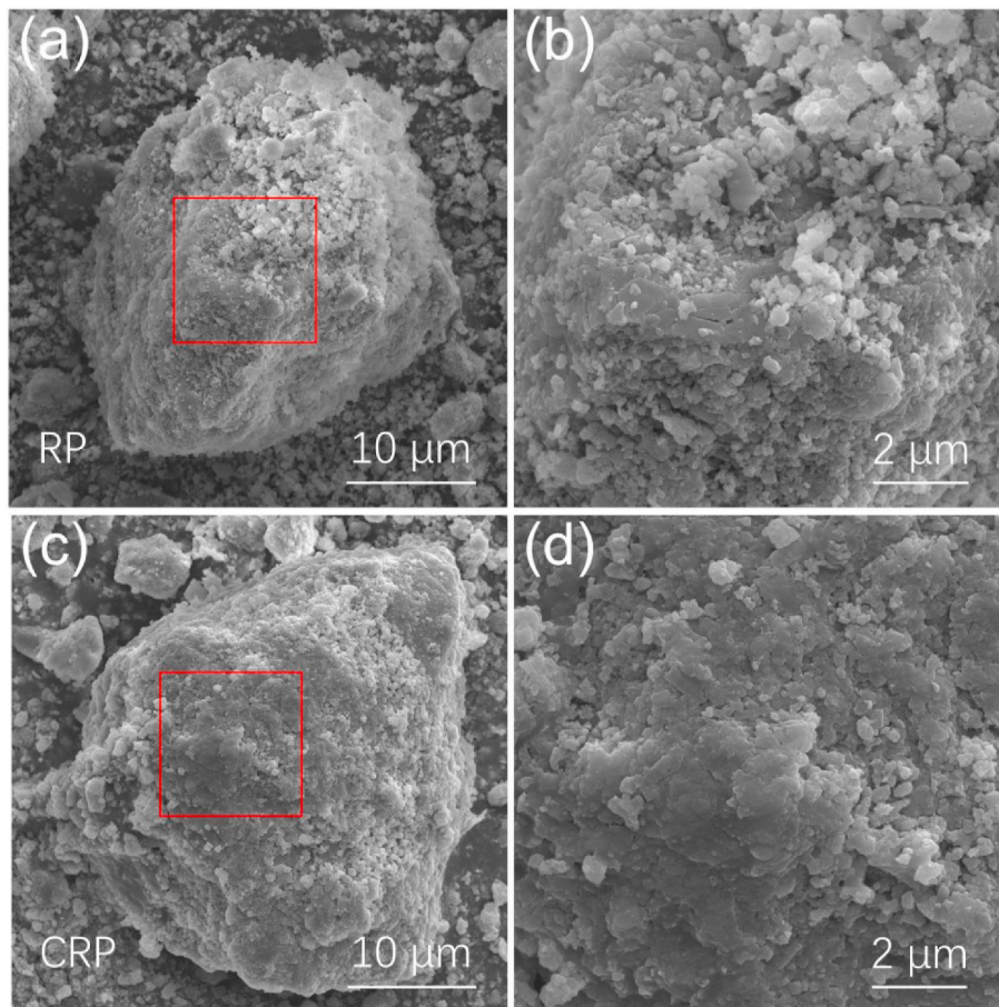
Fig. 5. Morphology of RP (a, b) and CRP (c, d).
