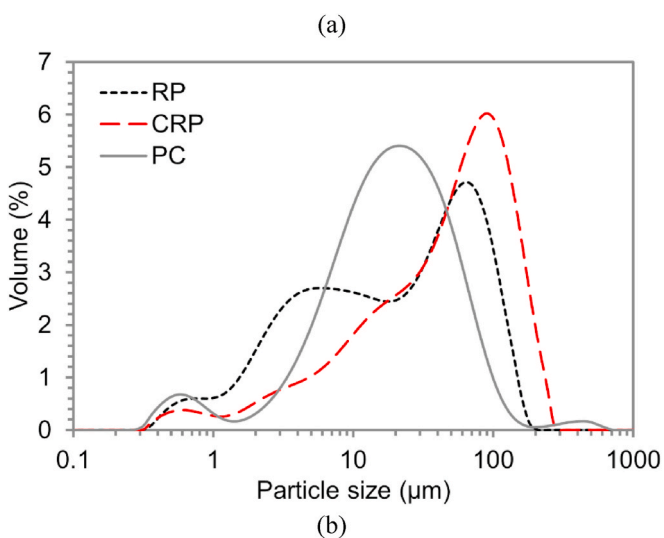
Fig. 1. Cumulative distribution (a) and volume distribution (b) of particle size of cement, RP and CRP.
