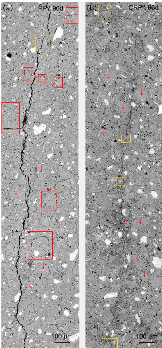
Fig. 11. Crack propagation in cement paste incorporating 30% RP (a), and 30% CRP (b) at 96 days (The red boxes mark the crack propagated alongside the RP or CRP particles, the yellow boxes refer to the crack passed through the RP or CRP particles, and the red arrows indicate the RP or CRP particles). (For interpretation of the references to colour in this figure legend, the reader is referred to the Web version of this article.)
