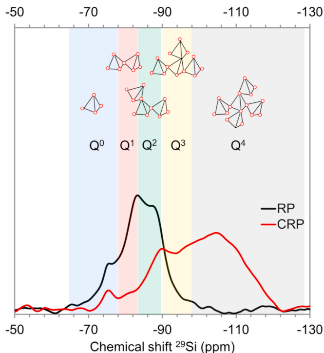
Fig. 4. 29 Si MAS NMR spectra for RP and CRP.
