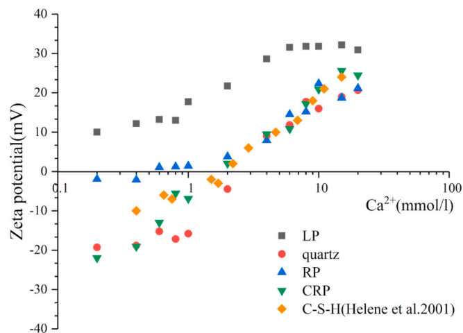
Fig. 6. The zeta potential of RP and CRP as a function of Ca 2+ concentration in Ca(OH) 2 solution.
