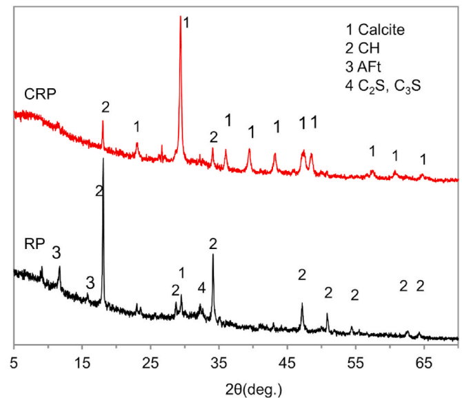
Fig. 2. XRD patterns of RP and CRP.
