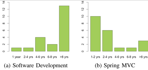
Figure 2: Participants' experience
