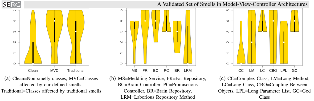
Figure 3: Participants on the severity of each smell.
