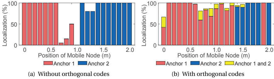
Figure 7.1: Localization accuracy experiment with two anchors placed two meters apart. We demonstrate the elimination of the packet reception dead zone with orthogonal codes, see Section 7.3.1 for details of the experiment setup.
