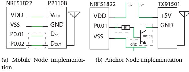
Figure 7.2: Implementation of WiPLOC components: (a) Mobile Node: Nordic Semiconductors nRF51822 SoC [153] connected to Powercast energy harvester P2110B [166]; and (b) Anchor Node: nRF51822 connected to Powercast power transmitter [166]. Note that in case of nRF51822 only the relevant pin connections are shown as other pins are left as not connected. The connections inside the dotted line are only applicable for WiPLOC++, refer to Section 7.5. The value for R_1 = 330 \Omega .
