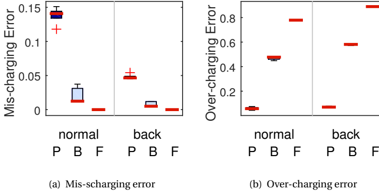
Figure 6.10: WPTN experiment results: (a); B—Beaconing, P—Probing, F—Freerun; Refer to Section 6.7.4 for more explanation.
