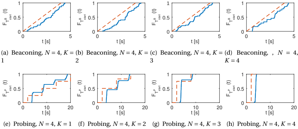
Figure 6.8: WPTN time to charge CDF: P—Probing, B—Beaconing, solid line—experiment, dashed line—analysis.
