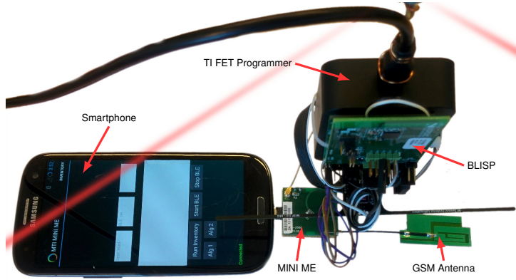
Figure 5.4: Mobile receiver BLISP test setup. BLISP and TI FET programmer/power monitor are hanging from an overhead crane (the red diagonal wires) [27] as described in Section 5.6.1. MINI ME mobile RFID reader is shown without plastic housing, easing connection of a different antenna.
