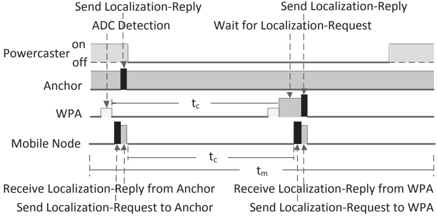
Figure 7.5: Semi-passive wakeup process during localization period t_m .
