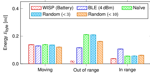
(a) Energy per byte comparison for all setups in different scenarios
