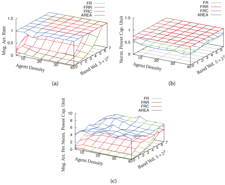
Figure 3.4: (a).Average message arriving rate for various agent densities and bandwidths. (b).Normalized average power consumption unit for various agent densities and bandwidths. (c).Average message arriving count per normalized power consumption unit for various agent densities and bandwidths.
