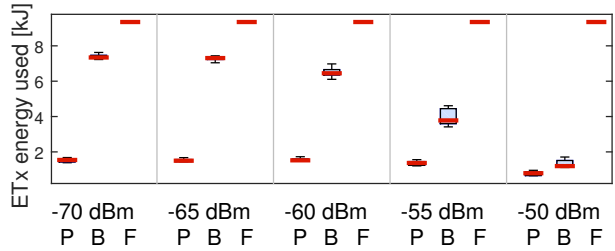
(b) ETx consumed energy
