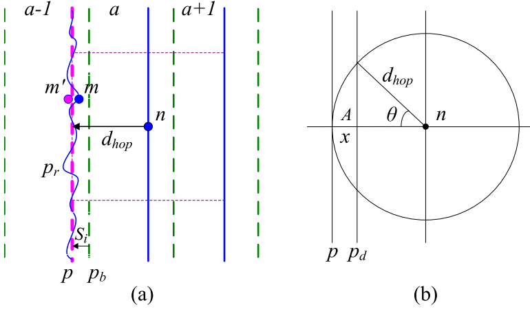
Figure 4.4: (a). Overestimation of gradient width reduction. (b). Expected reduced wave width.
