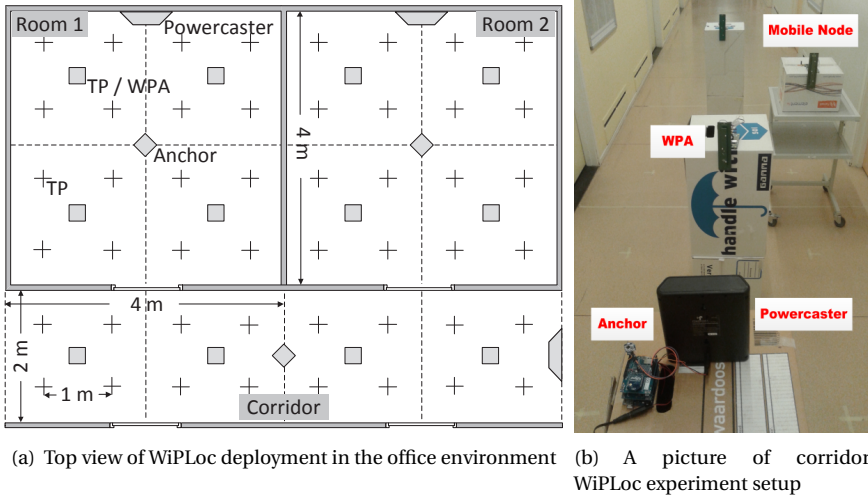
Figure 7.3: Experiment setup: TP/WPA : The places marked as "□" are used as the testing positions (TP) of Mobile Node in the room-level localization experiment of Section 7.4 and the deployment positions of WPA and in the cell-level localization experiment of Section 7.5, respectively. TP : places marked as "+" are the testing positions (TP) of Mobile Node in the cell-level localization experiment of Section 7.5.
