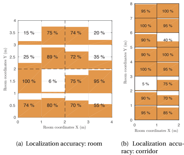
Figure 7.7: WiPLoc++ localization results. The values in orange rectangles of two figures represent the cell-level localization accuracy of WiPLoc++ measured per testing positions of (a) room two and (b) corridor as shown in Fig. 7.3(a).
