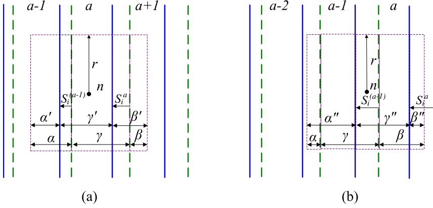
Figure 4.3: Average gradient for reduced width waves.
