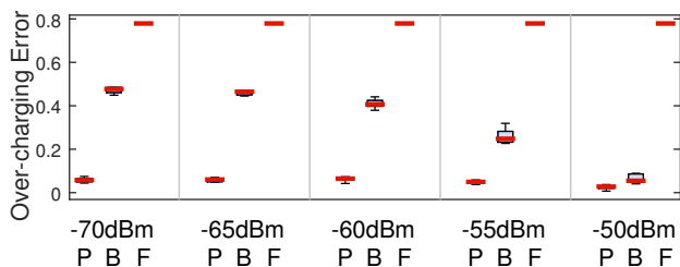
(c) Over-charging Error
