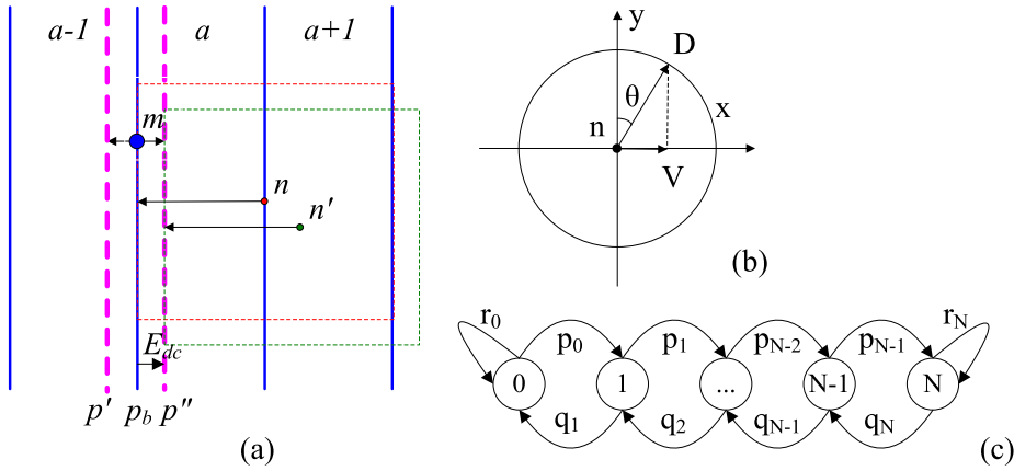
Figure 4.5: (a). Influence of node mobility to the border of the hop-count gradient wave. (b). Expected moving distance. (c). Moving distances of each time step of a round in the Markov Chain.
