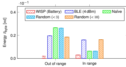
(a) Energy per byte comparison for all setups in different scenarios
