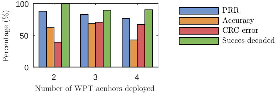
Figure 7.4: Cell-level localization as a function of number of Anchor Nodes deployed. The radio interference from multiple Anchor Nodes causes the increase of CRC error and the decrease of success decode rate.
