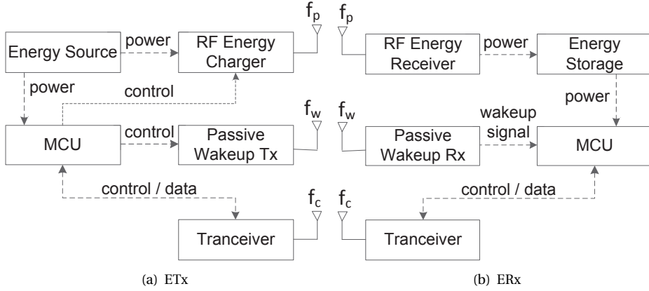
Figure 6.2: WPTN components: ETx (left) and ERx (right).
