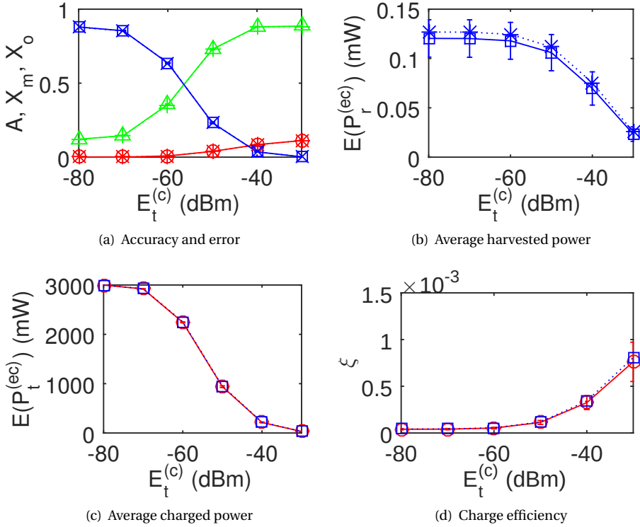
Figure 6.3: Simulation (solid line) and analytical (dotted line) results of WPTN evaluation parameters: (a) charging accuracy (green triangle), over-charging error (blue square), mis-charging error (red circle); (b) average harvested power; (c) average charged power; and (d) charging efficiency. In the simulation the ERx is placed at 10000 random positions with 10 test rounds. The parameters are: R_{\min} = 1 m; R_{\max} = 10 m; d_0 = 1 m; n = 3 ; \sigma = 7 ; f_p = 915 MHz; f_c = 2.4 GHz; E_t^{(e)} = -10 dBm; P_t^{(e)} = 3000 mW; P_t^{(c)} = 10 mW.
