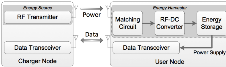
Figure 2.12: The operation process of the wireless power transfer system researched in this dissertation. Parallel RF channels are used to transfer energy and exchange data.
