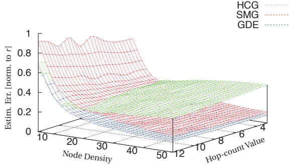
Figure 4.6: Absolute error for various node densities and hop-count gradient values.
