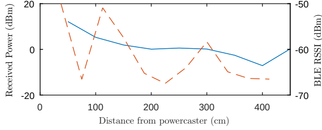
Figure 7.6: Signal strength of WPT and BLE communication signal. The solid line shows the received power calculated from the D_{out} from the harvester. The dotted line shows the RSSI from the nRF51822.
