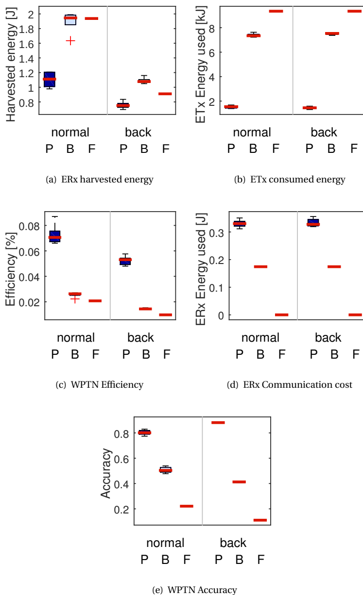
Figure 6.9: WPTN experiment results: (a); B—Beaconing, P—Probing, F—Freerun; Refer to Section 6.7.4 for more explanation.
