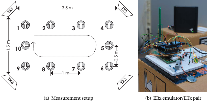
Figure 6.5: WPTN experiment setup: (a) ERx—gray circles, with its position (marked as 1–10) and its orientation (marked with arrows), where dashed arrow denotes the ERx movement direction; and ETx—white trapezoid, see also Section 6.6.4, (b) photograph of the ERx emulator/ETx pair in the laboratory setting—front: ERx emulator, back: one ETx.
