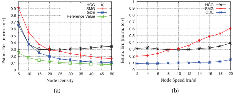
Figure 4.7: (a). Absolute error for various node densities. (b). Absolute error for various node speeds.
