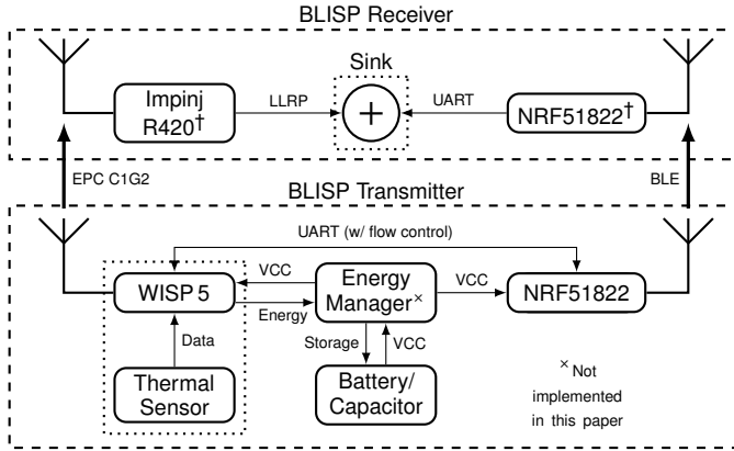
Figure 5.2: Overview of the BLISP system consisting of one transmitter and one receiver. The temperature sensor providing data is part of WISP but displayed separately for clarity and completeness. All displayed connections depict a flow of energy or data and do not directly correspond to physical connections. For a detailed description of the physical connections see [79]. † For the mobile reader experiments the Impinj R420 is replaced by an MTI MINI ME, and the NRF51822 by the BLE receiver of a Samsung Galaxy S3.
