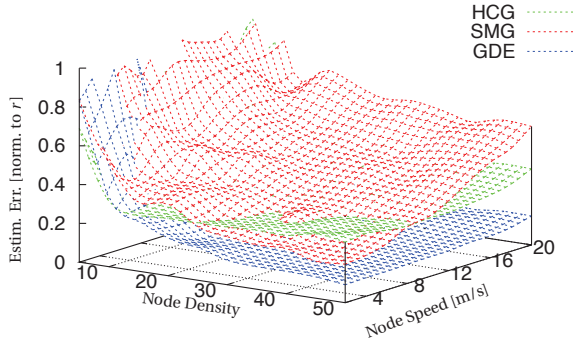
Figure 4.8: Absolute error for various node densities and node speeds.
