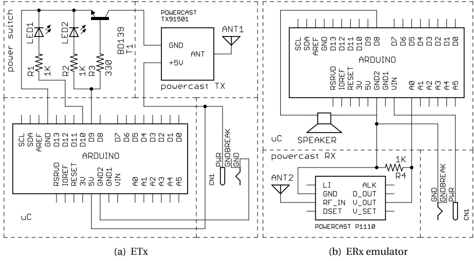
Figure 6.4: Components of the implemented WPTN: (a) ETx, and (b) ERx emulator and a charge measuring unit. Notes: LED1 and LED2 are used for ETx state indication purpose; value of resistor R4 is user-changeable allowing to test the effect of various ERx impedances on the WPTN performance.
