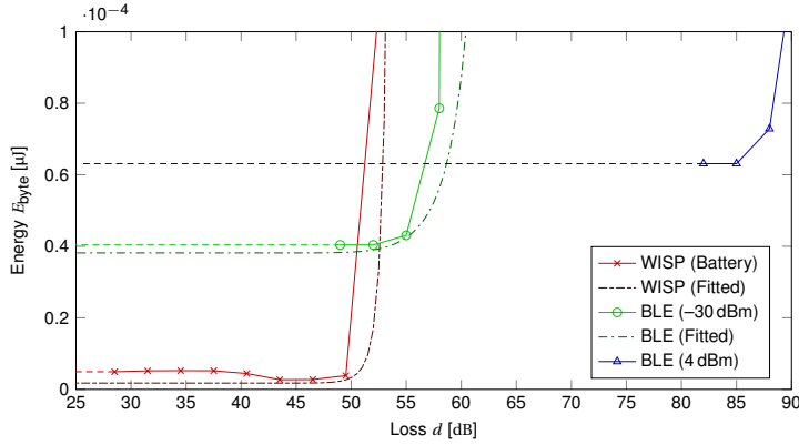
Figure 5.1: Energy per byte over distance for WISP and BLE. The dashed data points are extrapolated, the constant power consumption for the BLE radio and all data being received, yields constant energy per byte. Fitted plots are based upon (5.1). Parameters for fitted WISP curve: a_i = 30 , d_i = 4 , E_{tx,i} = (L + H)5\mu\text{J} with L = 96 and H = 320 . Parameters for fitted BLE curve: a_i = 87 , d_i = 2 , E_{tx,i} = (L + H)21\mu\text{J} , L and H are equal to WISP.
