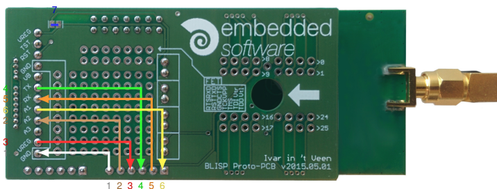
(b) Bottom side of the BLISP. Symbolically illustrated directional connections by color, as numbered: (1) white : ground; (2) brown : clear to send; (3) red : power supply; (4) green : WISP to BLE serial channel; (5) orange : BLE to WISP serial channel (unused); (6) yellow : ready to send, and (7) blue : power supply.
