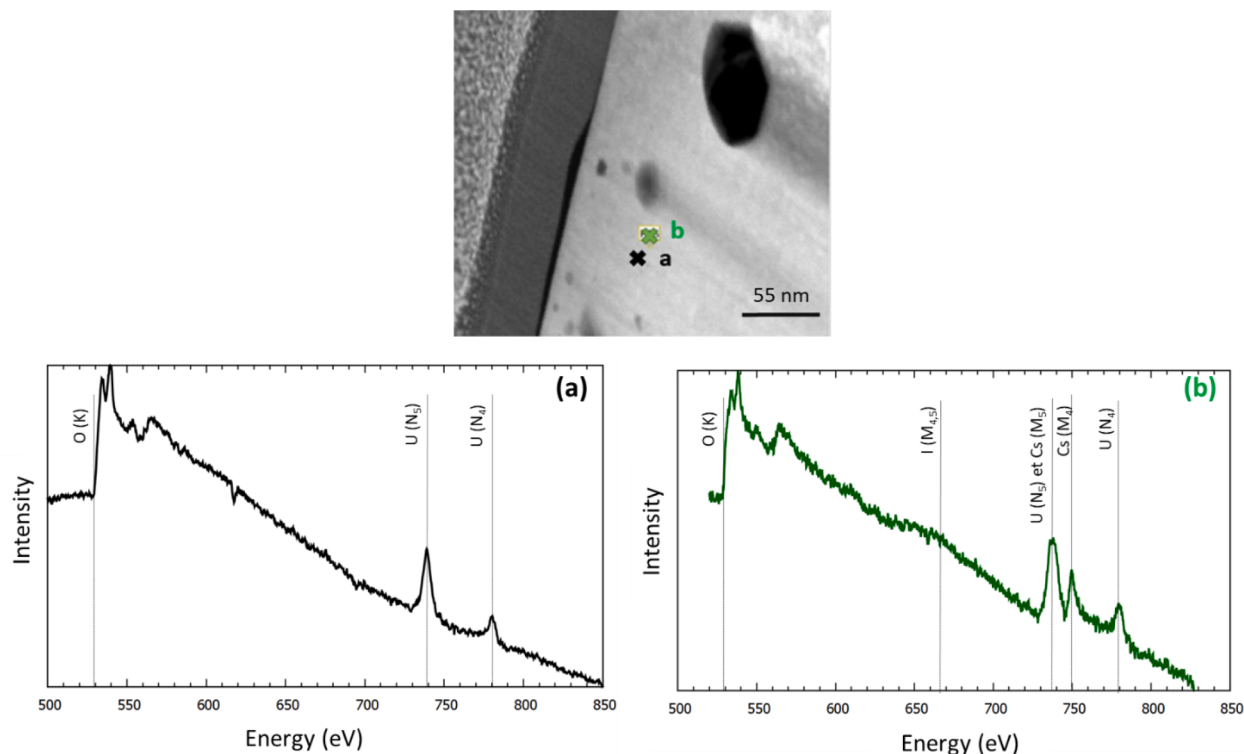
Fig. 13. HAADF image and EELS spectra from sample HC heat treated at 1200°C at different positions: (a) in the \text{UO}_2 matrix and (b) in a bubble containing Cs and I.
