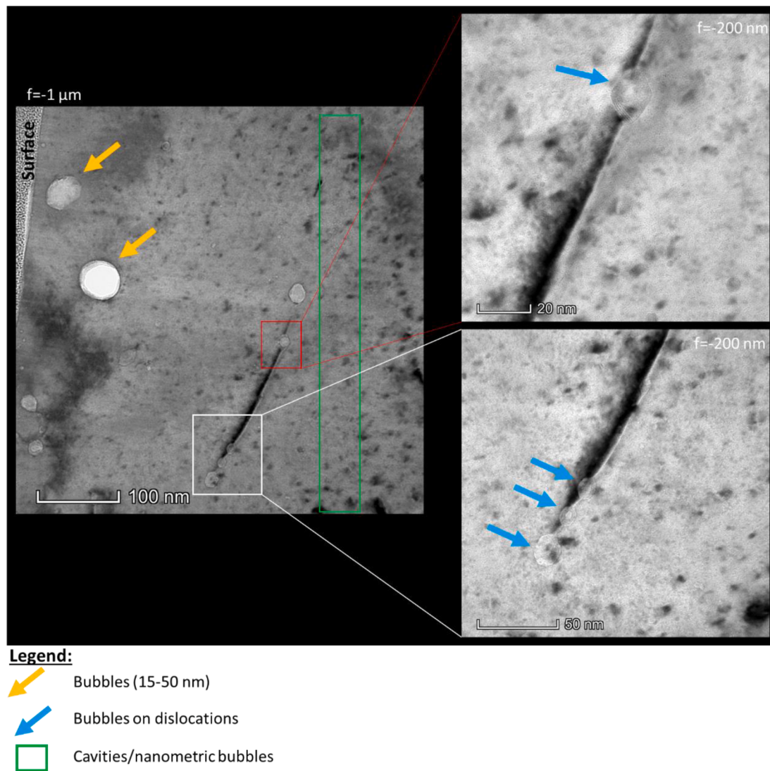
Fig. 6. Bright field TEM images of the HC sample after a thermal treatment at 1200°C during 1 h (f indicates focus).
