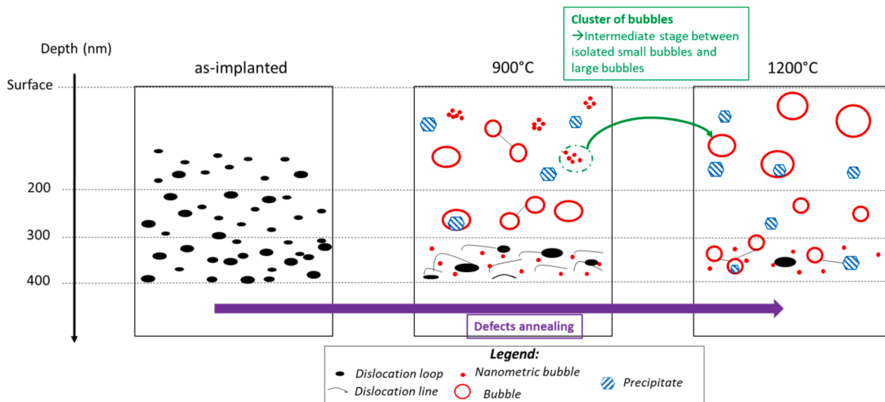
Fig. 14. Schematic illustration of the evolution of the microstructure of \text{UO}_2 lamellae implanted with Cs and I before and after annealing at 900°C and 1200°C.
