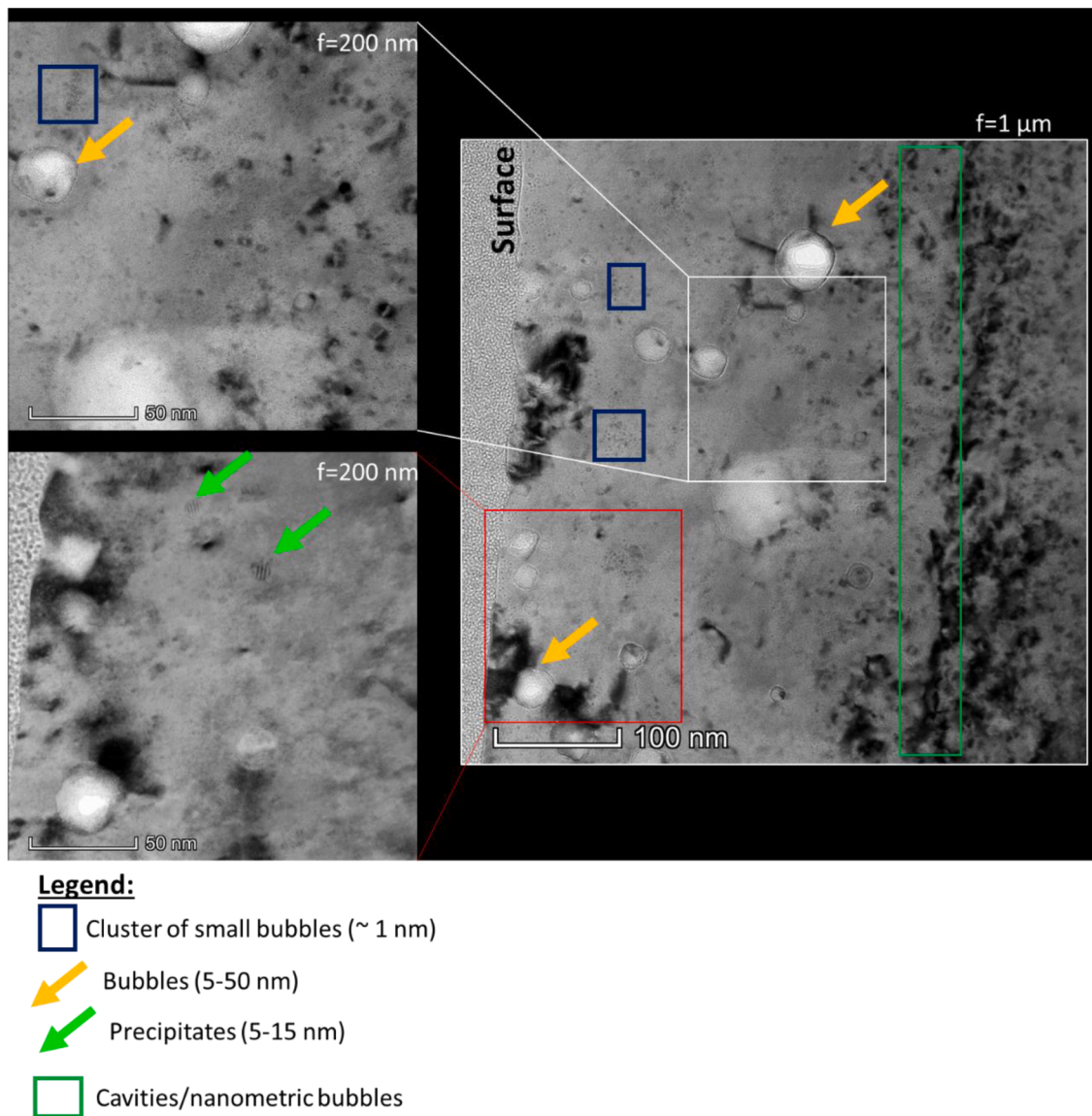
Fig. 5. Bright field TEM images in over-focused conditions of the HC sample after a heat treatment at 900°C during 4 h (f indicates focus).
