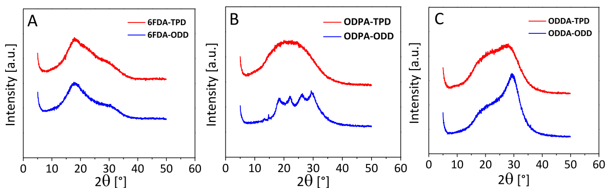
Fig. 4. XRD results of the fully imidized PI films. The intensity is plotted as a function of the scattering angle. All curves have been translated vertically for sake of clarity. (A) 6FDA-series, (B) ODPA-series and (C) ODDA-series.
