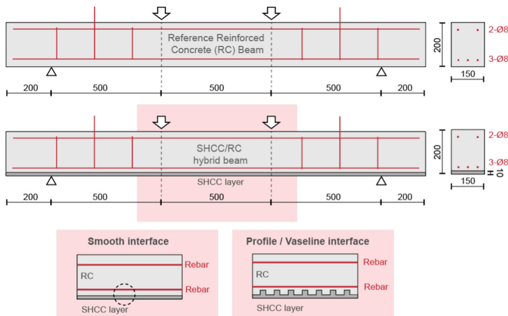
Fig. 1. Design details of the beams [unit in mm].
