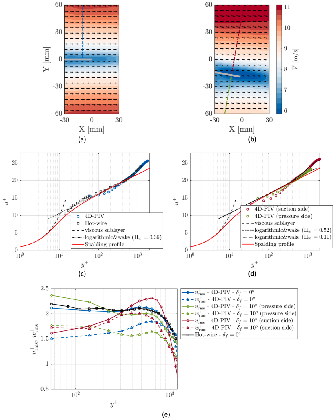
Fig. 15. Mean flow over the trailing edge and boundary-layer mean velocity profile measured at the trailing edge at \delta_f = 0^\circ (a and c respectively) and \delta_f = 10^\circ (b and d respectively) and root mean square (RMS) of the stream and spanwise velocity fluctuations (e). The dashed lines in (a) and (b) represent the region of extraction of the boundary-layer velocity profiles.
