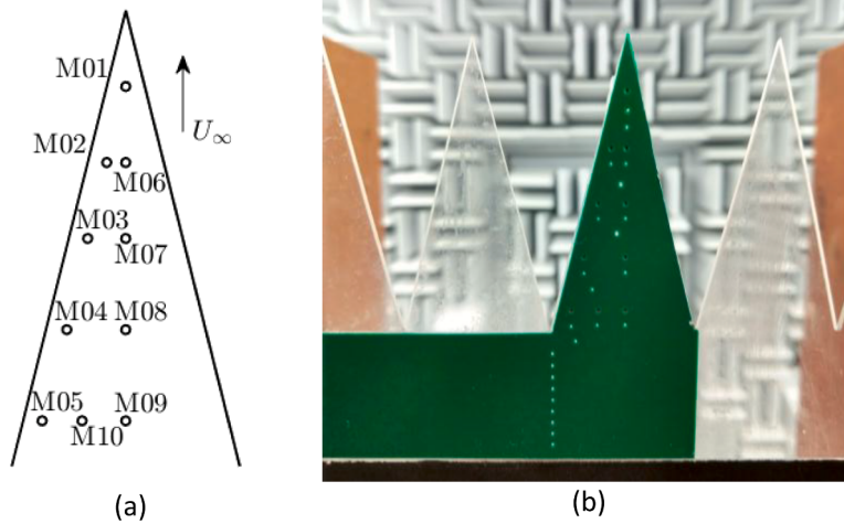
Fig. 2. Schematic description of the surface pressure sensors on the trailing-edge sawtooth (a). Photograph of the PCB integrated with the trailing-edge insert (b).
