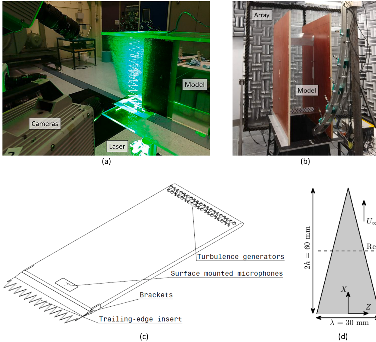
Fig. 1. Experimental set-up for the 3D-PIV (a) and acoustic (b) measurements. Details of the flat plate model (c) and the trailing-edge geometries tested (d). In the last picture, Ref. refers to the position of the baseline straight trailing edge at X = 1h used. The same picture also shows the coordinate system and origin adopted in the remainder of the study.
