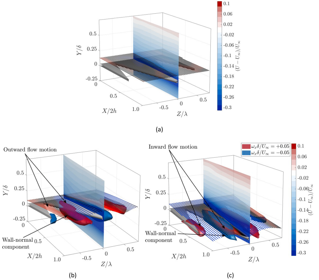
Fig. 4. 3D visualization of the mean flow over the trailing-edge serration at \delta_f = 0^\circ (a) and \delta_f = 10^\circ from the pressure (b) and suction side (c). Isosurfaces of streamwise vorticity are shown in red ( \omega_x \delta^* / U_\infty = +0.05 ) and blue ( \omega_x \delta^* / U_\infty = -0.05 ). Streamlines of the flow at Y/\delta = 0.1 . Black streamlines are undistorted, red and blue correspond to w \geq 0.04U_\infty and w \leq -0.04U_\infty respectively.
