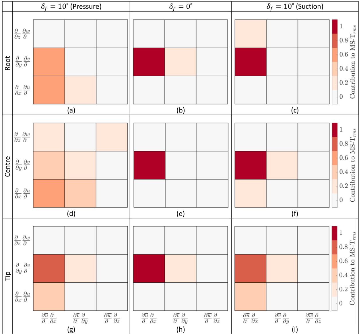
Fig. 12. Relative contribution of the root-mean-squared of each component \frac{\partial \bar{u}_i}{\partial x_j} \frac{\partial \bar{u}_j}{\partial x_i} to the mean shear-turbulence (MS-T) interaction term of the pressure Poisson equation estimated along the edges of the serration (one momentum thickness above the wall). Different flap angles, \delta_f = 0^\circ (b, e, and h) and \delta_f = 10^\circ on the pressure (a, d, and g) and suction sides (c, f, and i) are represented.
