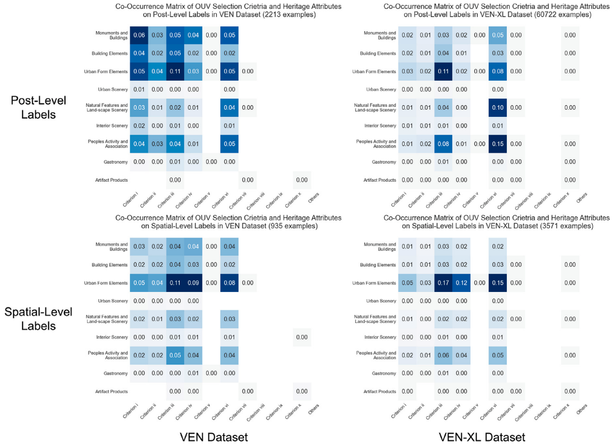
Fig. 8. The normalized co-occurrence matrix heatmaps O of the OUV and HA categories in post-level label array \hat{Y} and spatial-level label array \hat{Z} in both VEN and VEN-XL datasets.
