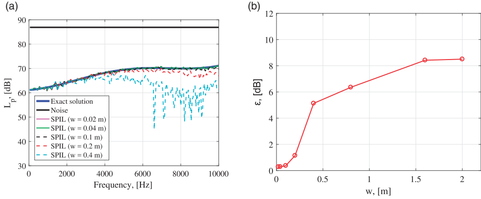
Figure 12. (a) Results of the sensitivity analysis performed for the SPIL method with respect to the ROI width w . Adapted from Sarradj et al. 25 (b) Average absolute errors \varepsilon made for each width case. For these results x_0 = 0 , l = 2 m and \Delta x = 0.01 m.
