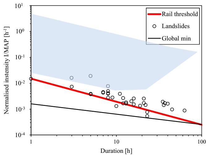
Fig. 10. I_{MAP-D} threshold for landslides on rail earthworks in Ireland. Shaded area – extent of I_{MAP-D} thresholds collated by Guzzetti et al. (2007). Global minimum I_{MAP-D} threshold – thin black line (Guzzetti et al., 2008).
